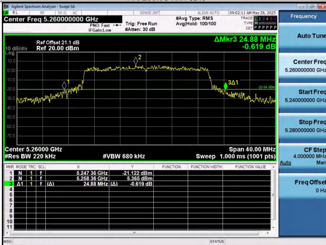
11AX20SISO-Ant1-5260
