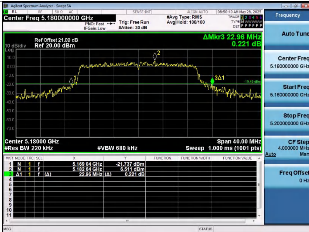
11AX20SISO-Ant1-5180
