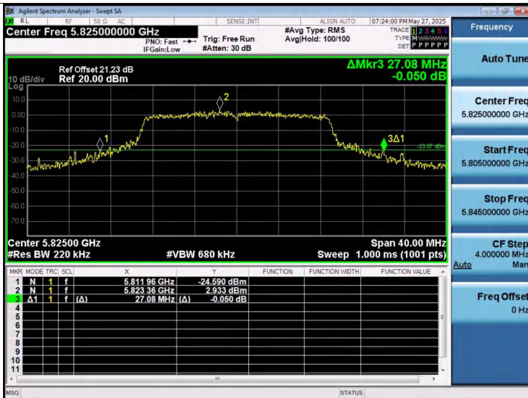
11AC20SISO-Ant1-5825
