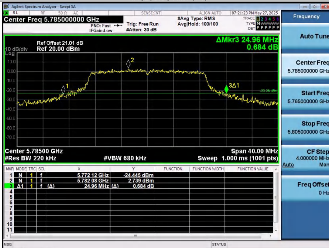
11AC20SISO-Ant1-5785
