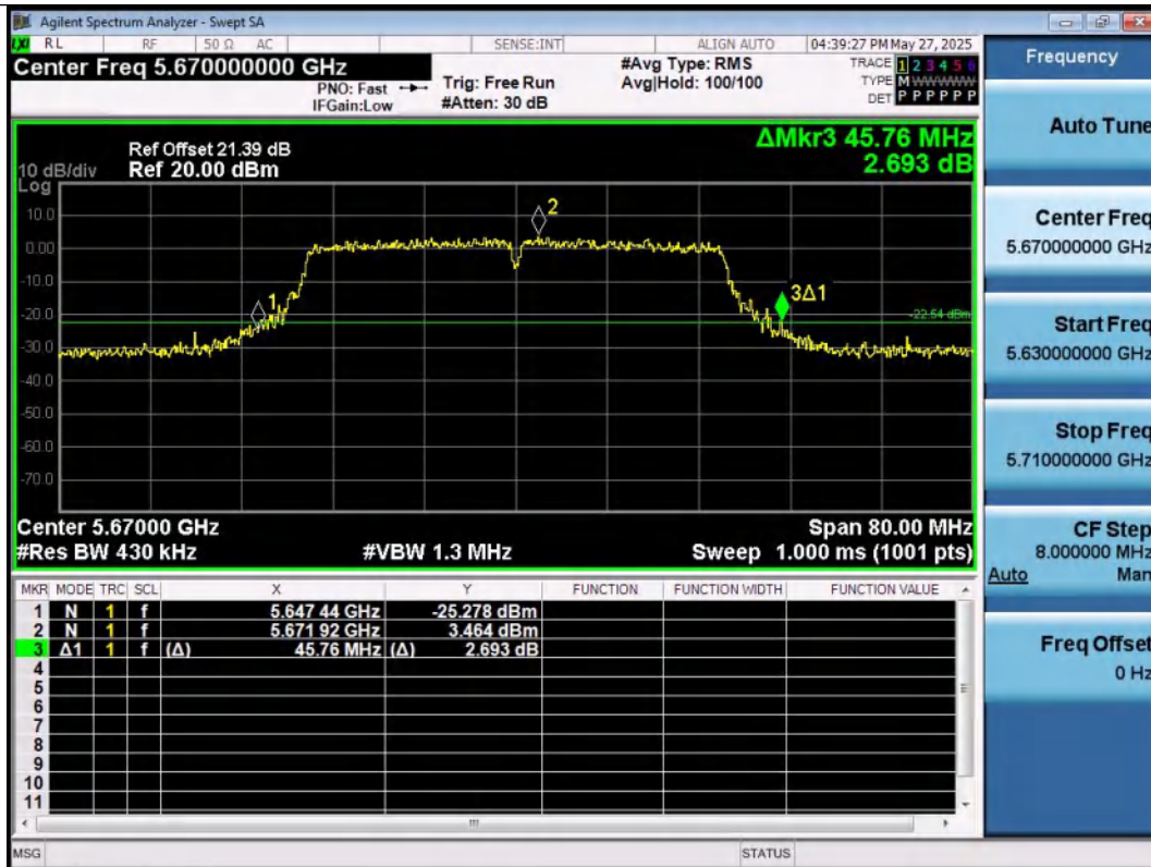
11N40SISO-Ant1-5670
