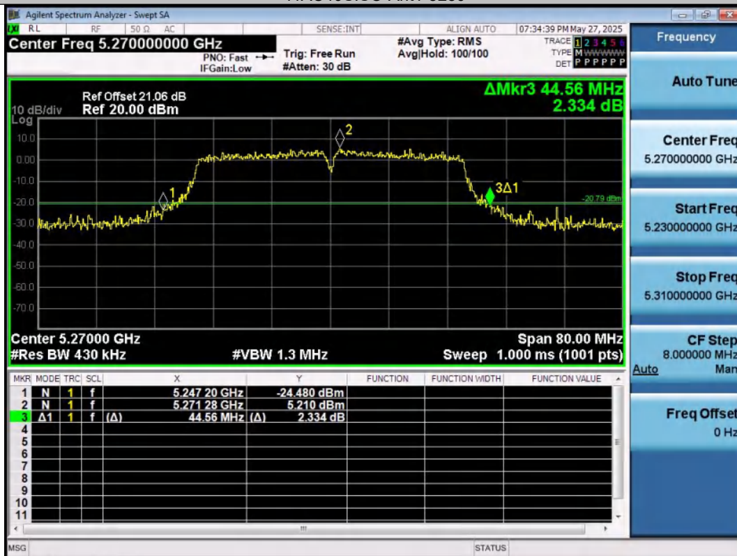
11AC40SISO-Ant1-5270
