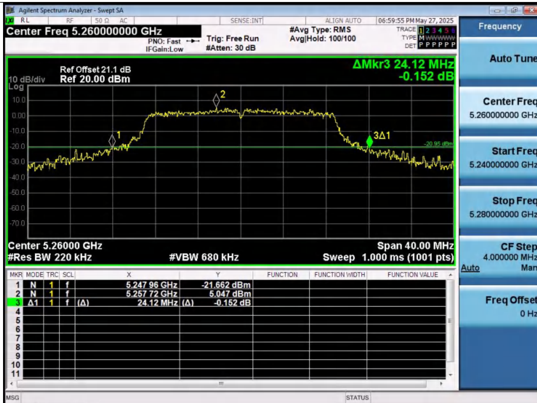
11AC20SISO-Ant1-5260
