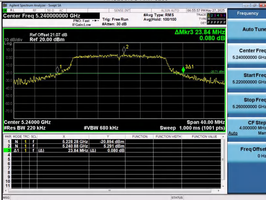
11AC20SISO-Ant1-5240
