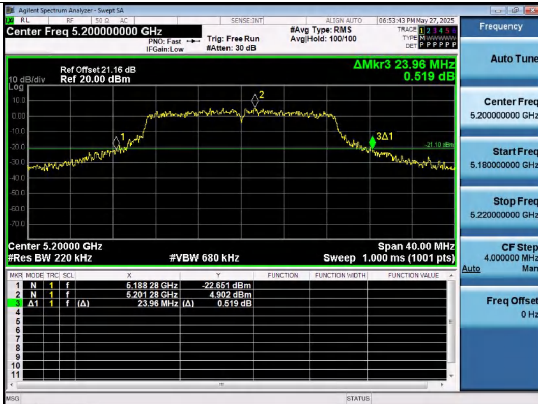
11AC20SISO-Ant1-5200
