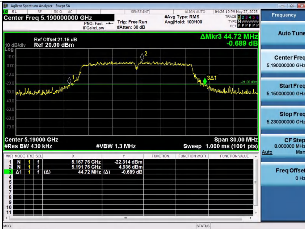
11N40SISO-Ant1-5190
