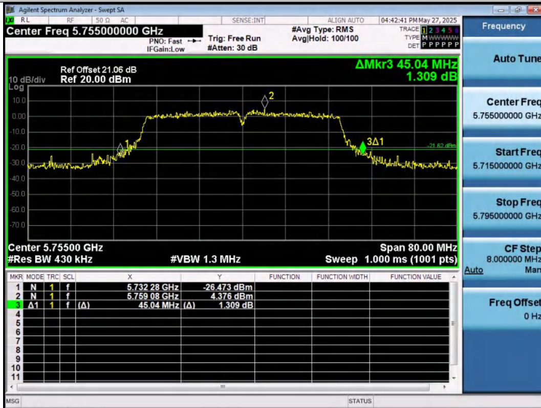
11N40SISO-Ant1-5755
