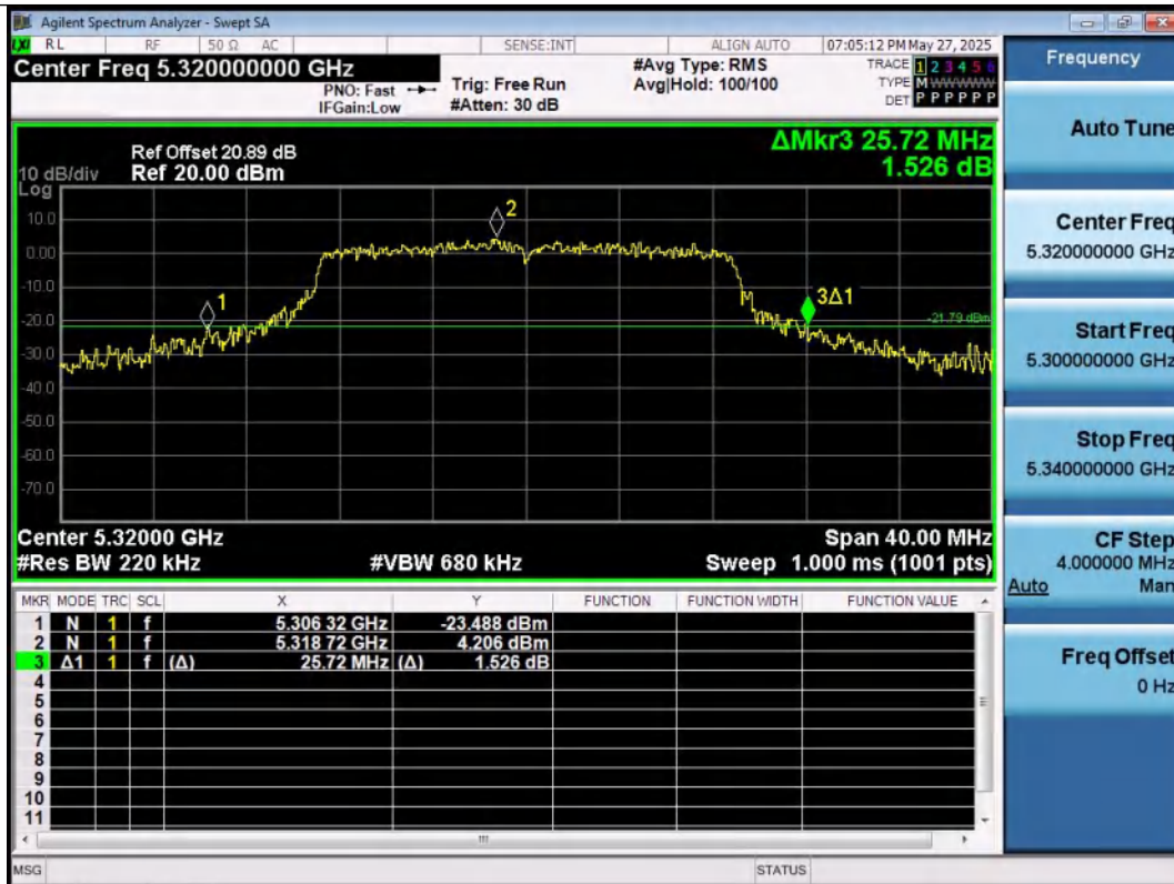
11AC20SISO-Ant1-5320
