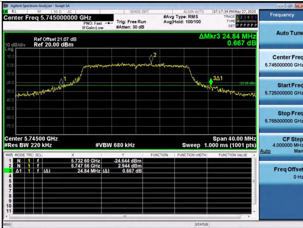
11AC20SISO-Ant1-5745
