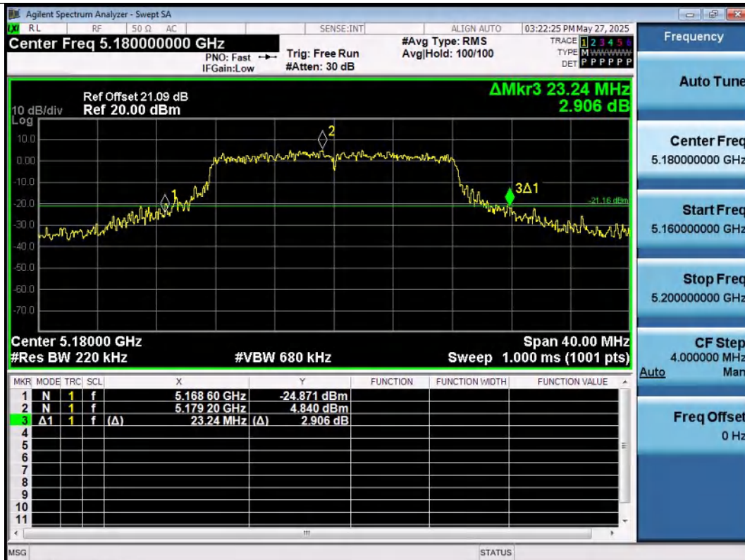
11A-Ant1-5180
