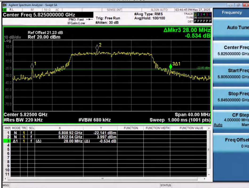
11A-Ant1-5825
