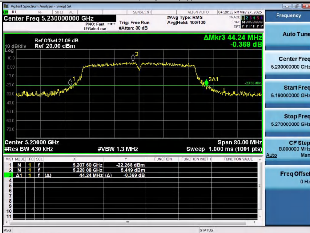
11N40SISO-Ant1-5230
