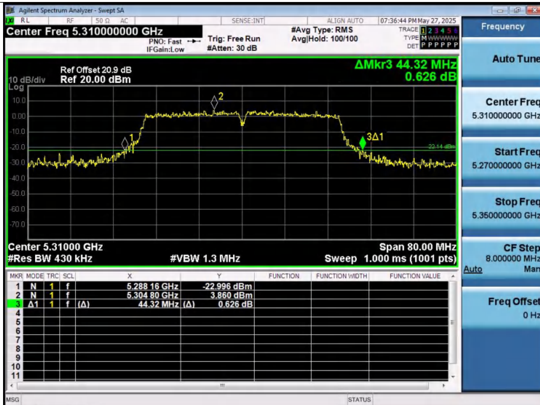
11AC40SISO-Ant1-5310
