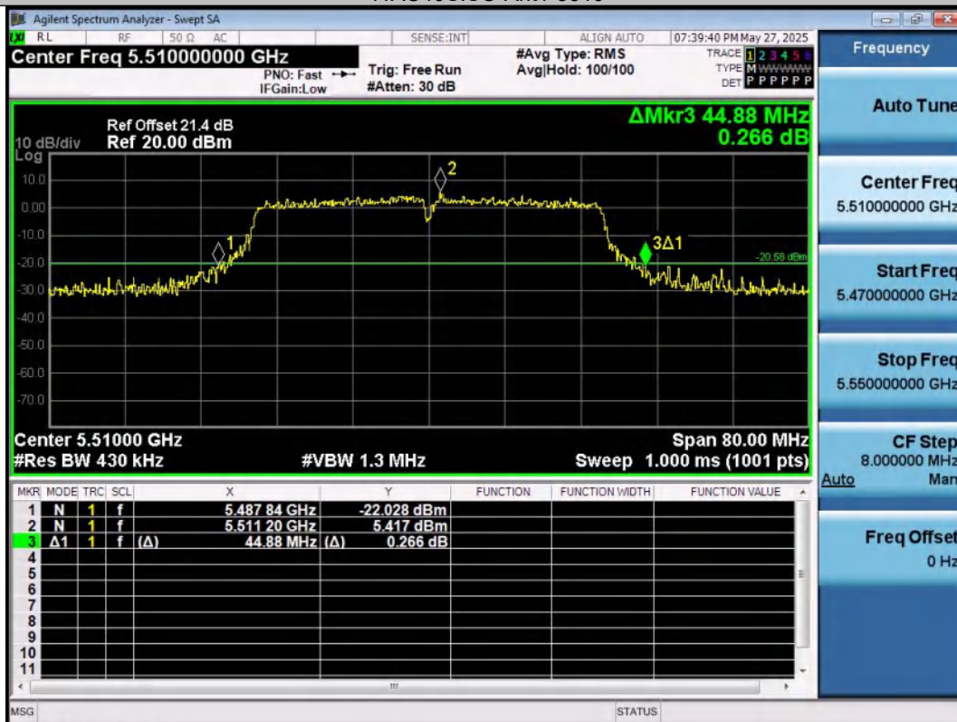
11AC40SISO-Ant1-5510
