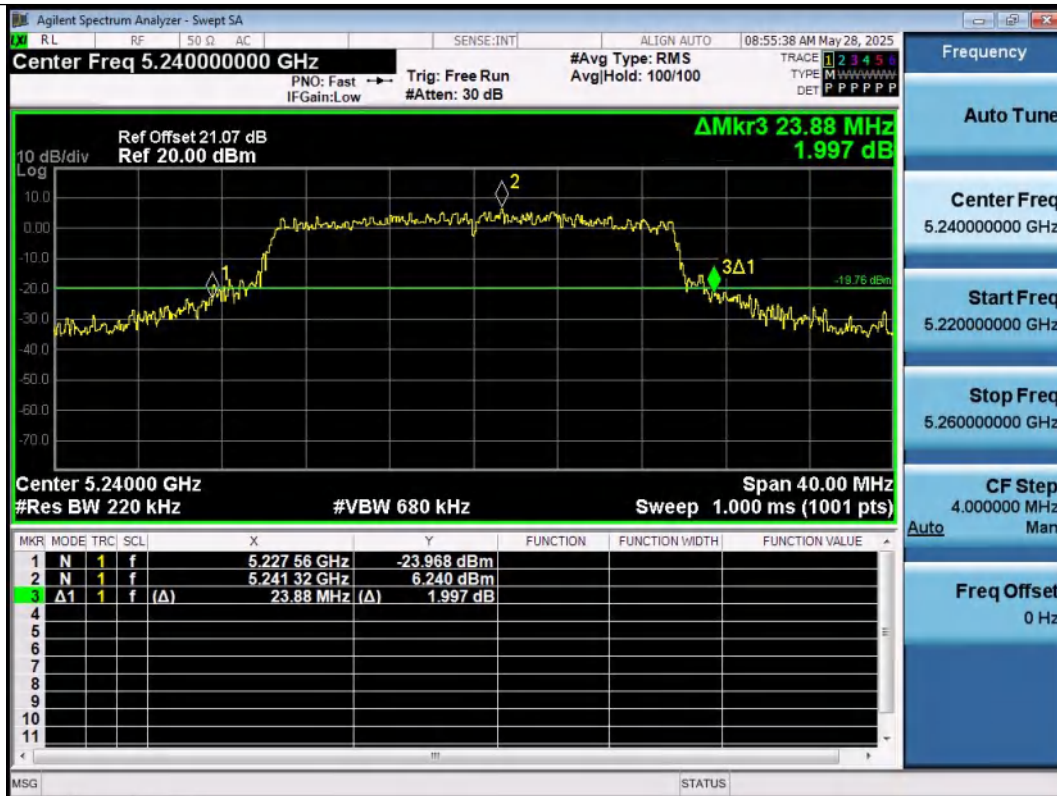
11AX20SISO-Ant1-5240
