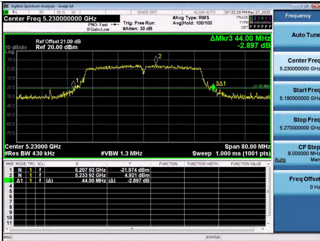
11AC40SISO-Ant1-5230
