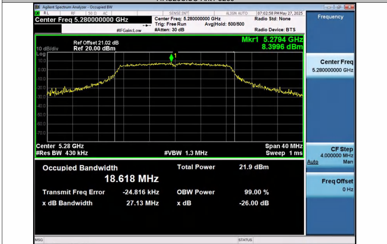
11AC20SISO-Ant1-5280
