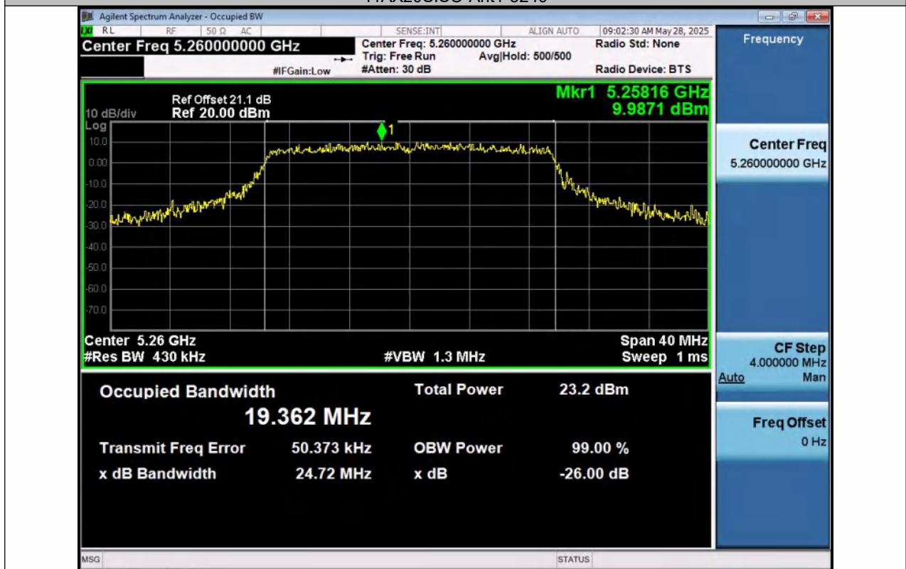
11AX20SISO-Ant1-5260
