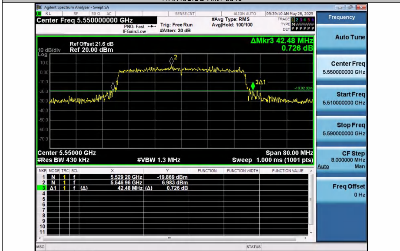
11AX40SISO-Ant1-5550
