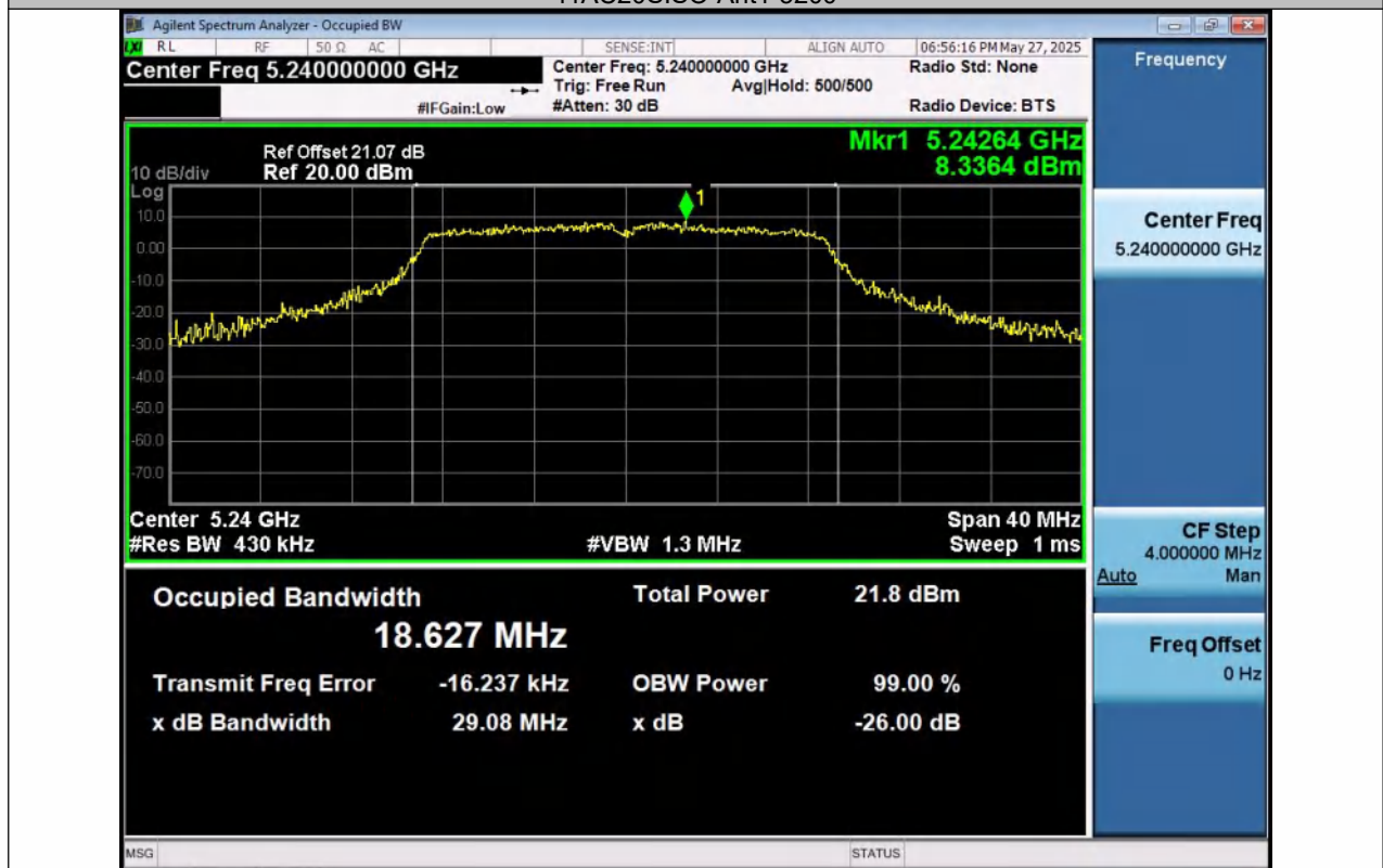
11AC20SISO-Ant1-5240
