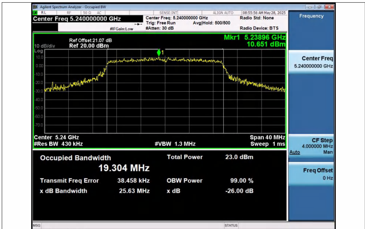
11AX20SISO-Ant1-5240
