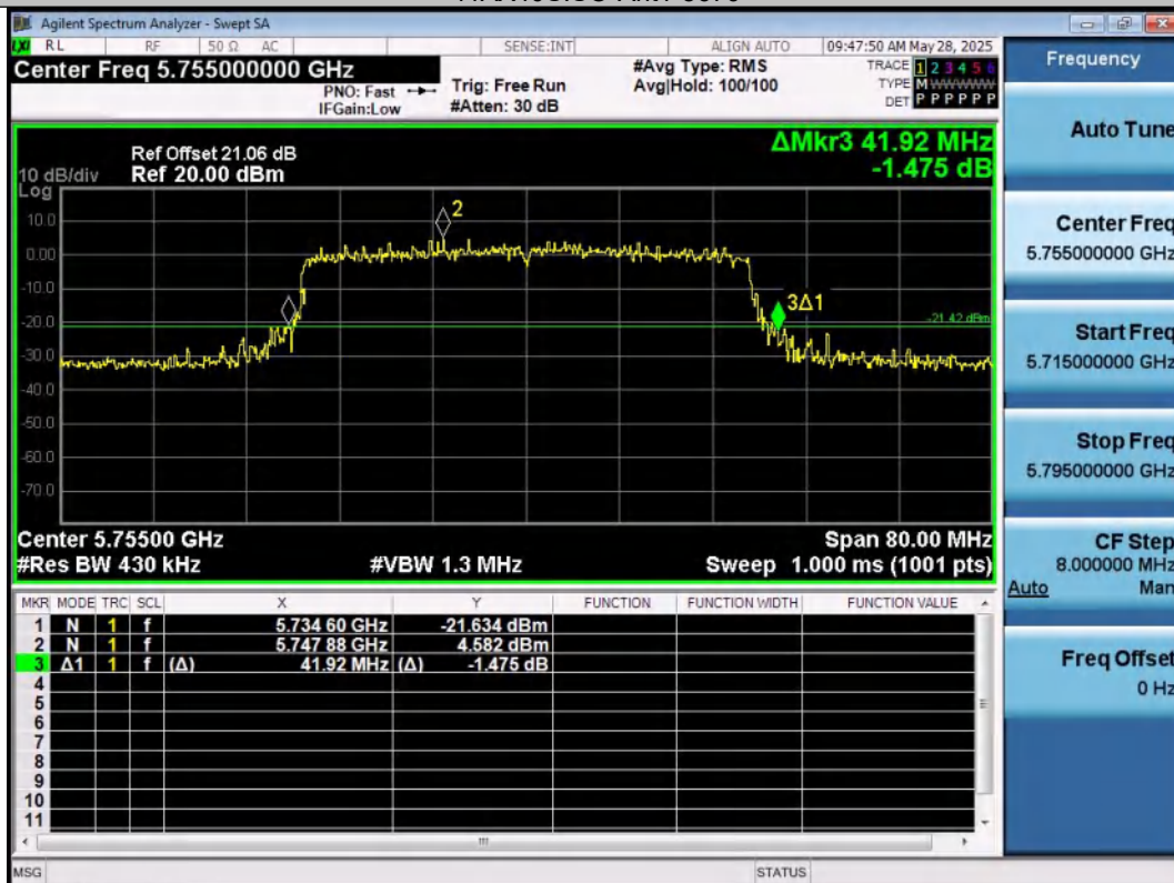
11AX40SISO-Ant1-5755
