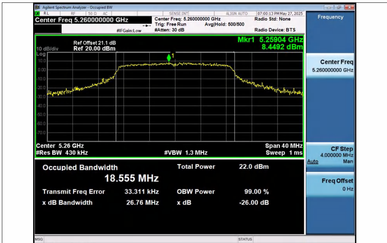
11AC20SISO-Ant1-5260
