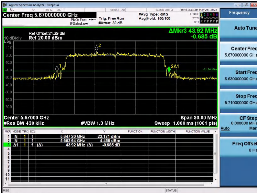
11AX40SISO-Ant1-5670
