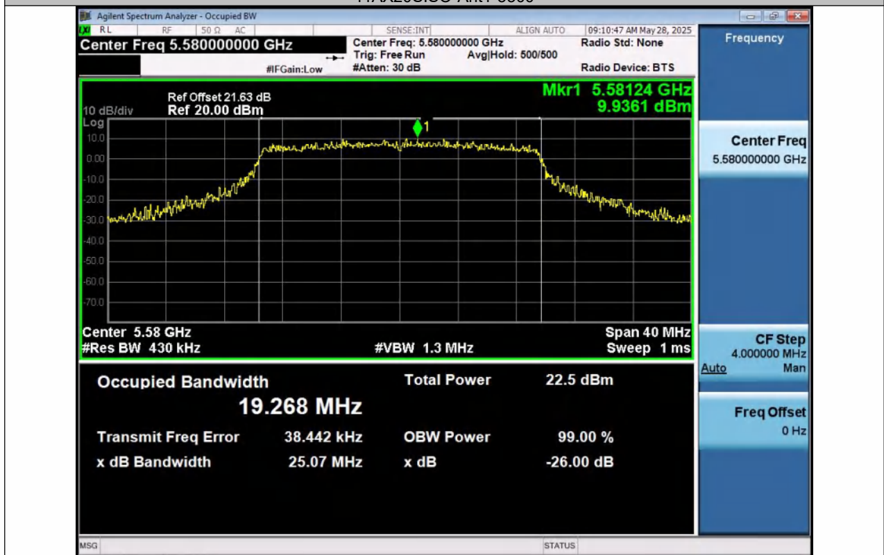
11AX20SISO-Ant1-5580
