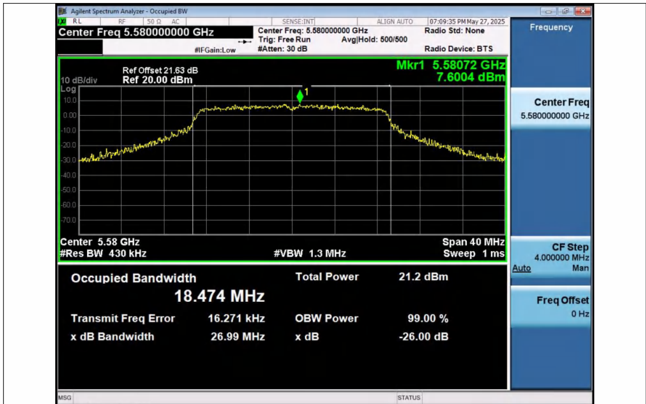
11AC20SISO-Ant1-5580
