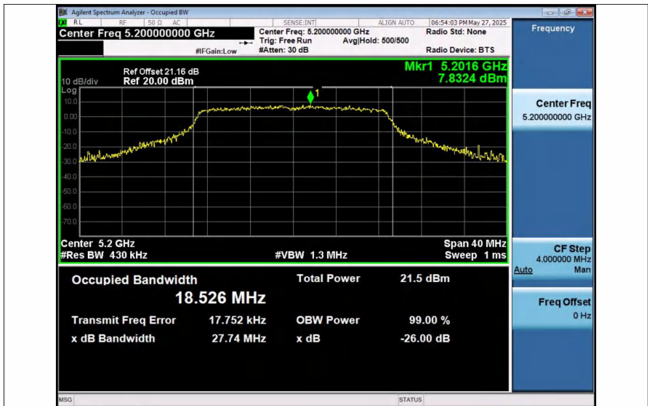
11AC20SISO-Ant1-5200
