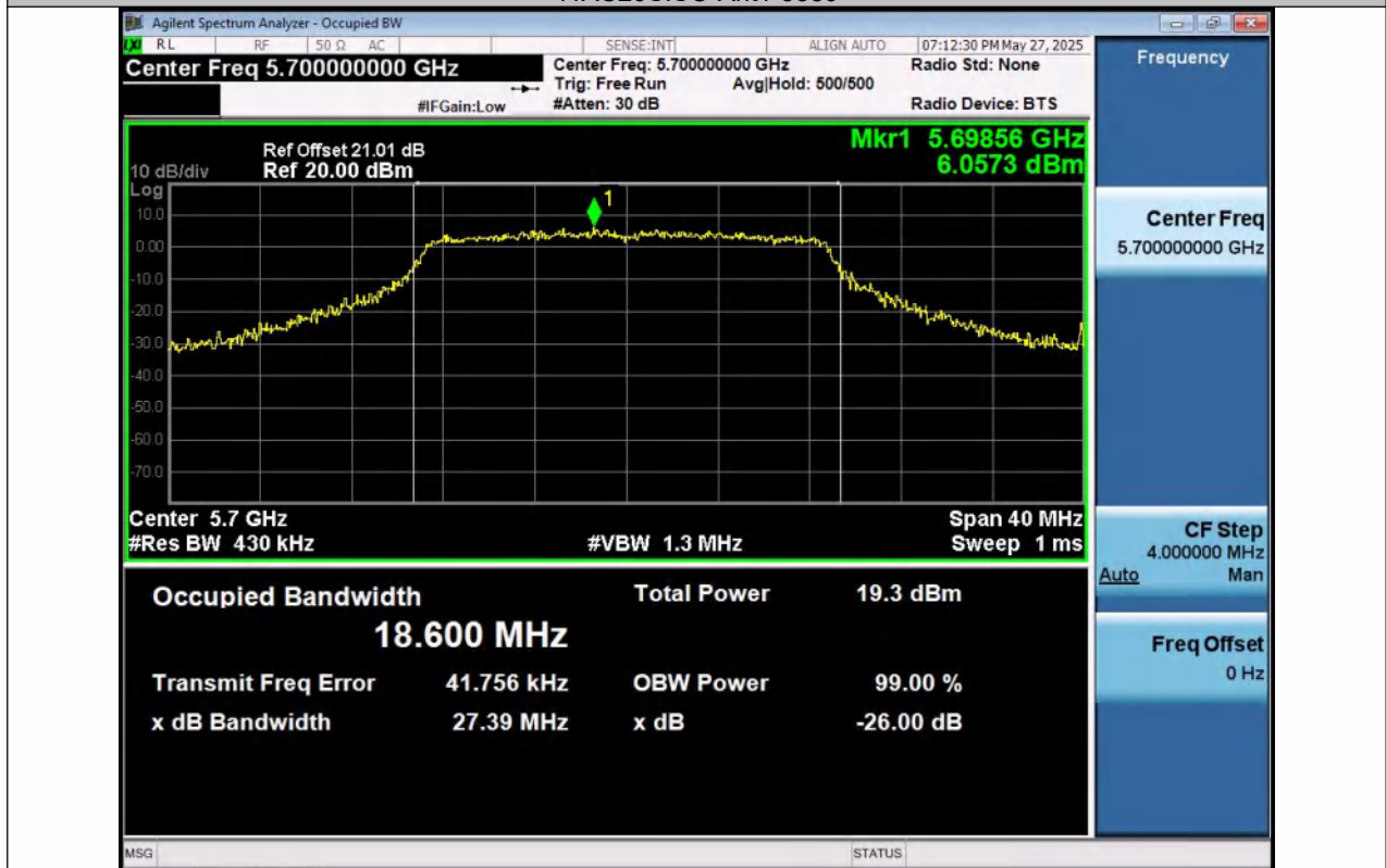
11AC20SISO-Ant1-5700
