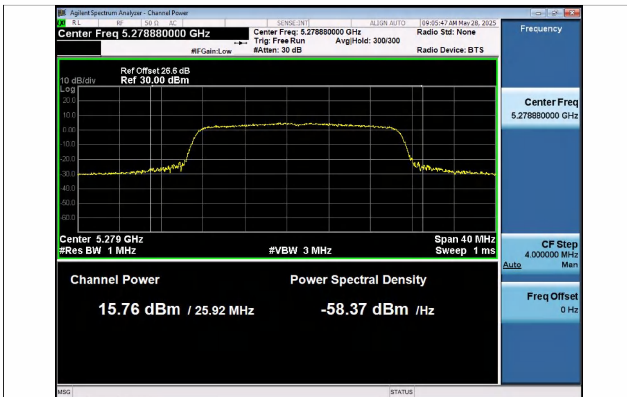
11AX20SISO-Ant1-5280-PASS
