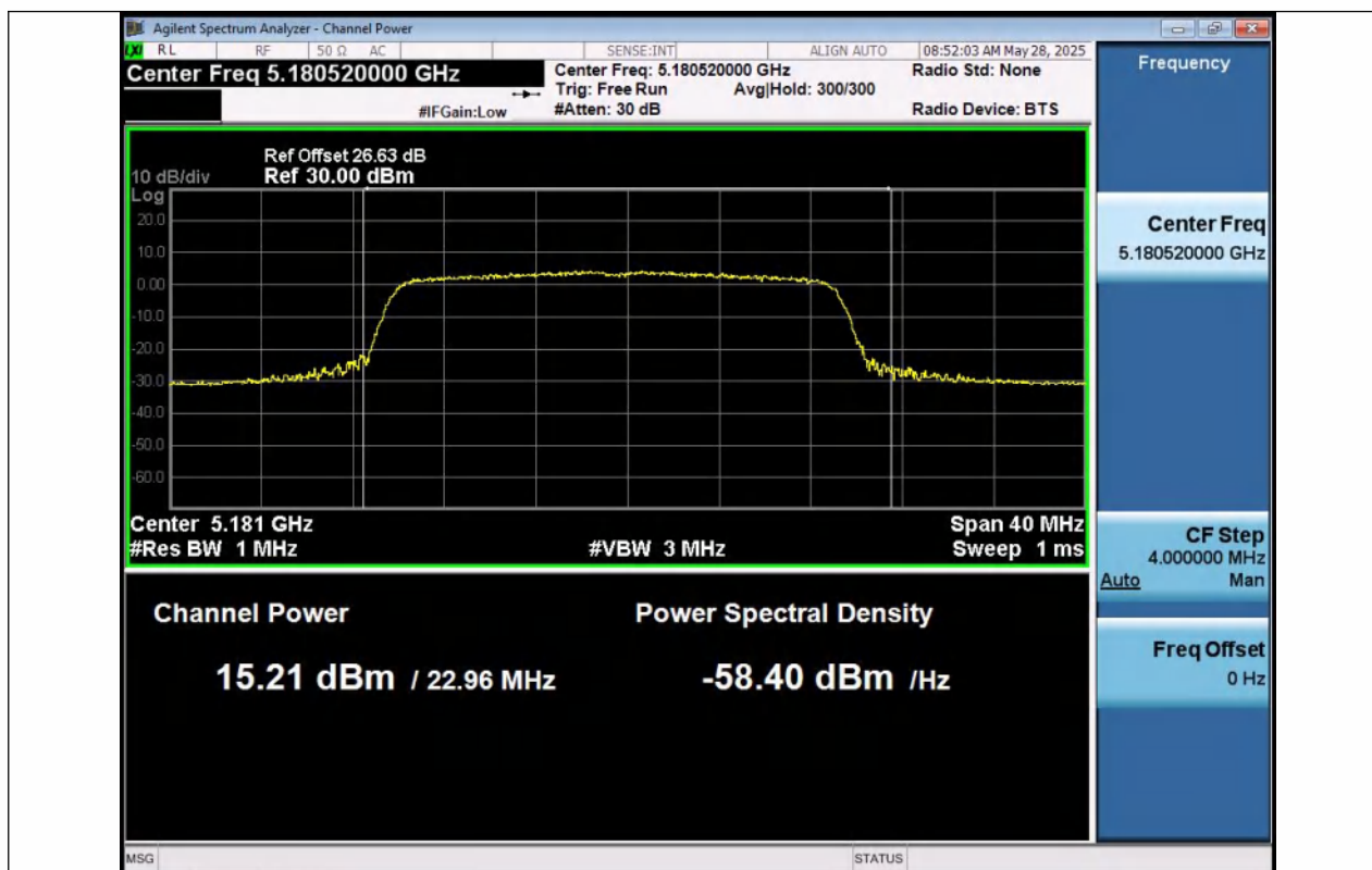
11AX20SISO-Ant1-5180-PASS
