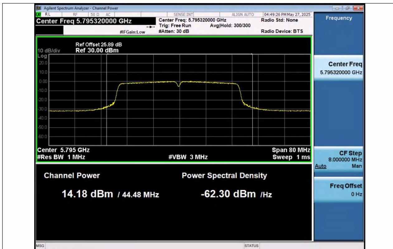
11N40SISO-Ant1-5795-PASS
