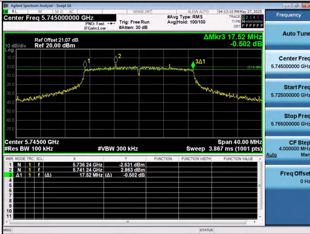
11N20SISO-Ant1-5745-PASS
