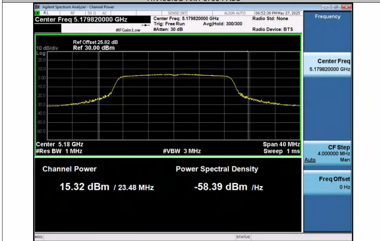
11AC20SISO-Ant1-5180-PASS
