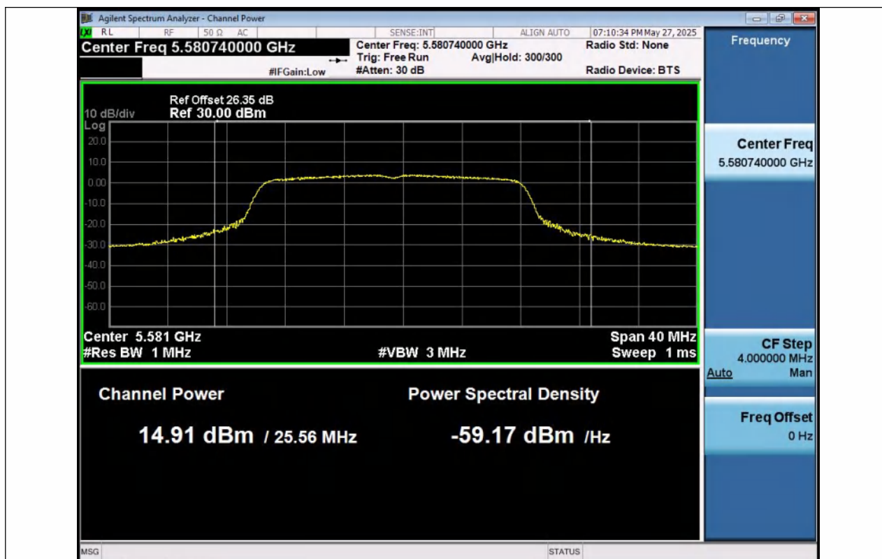
11AC20SISO-Ant1-5580-PASS
