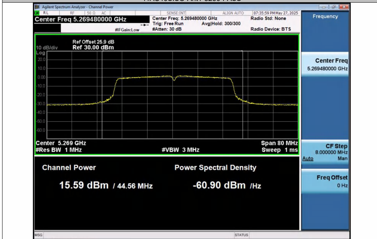
11AC40SISO-Ant1-5270-PASS
