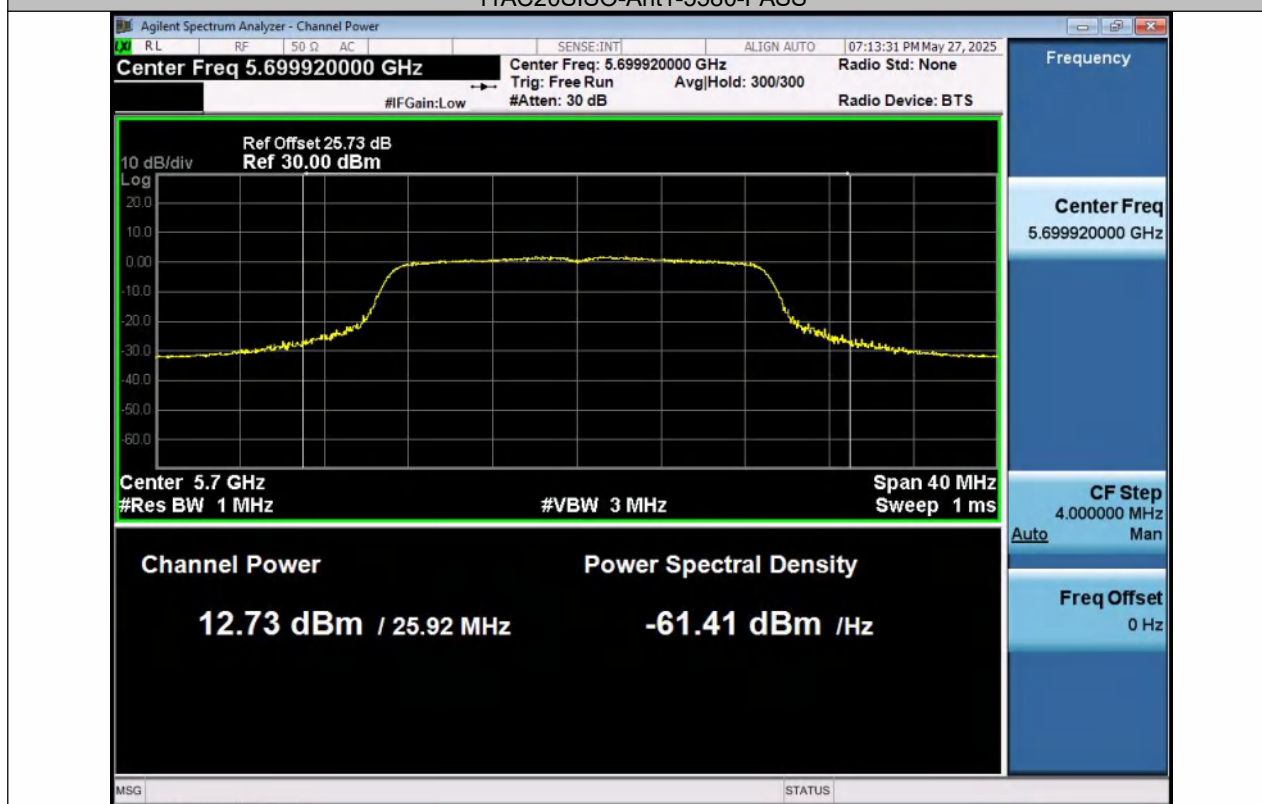
11AC20SISO-Ant1-5700-PASS
