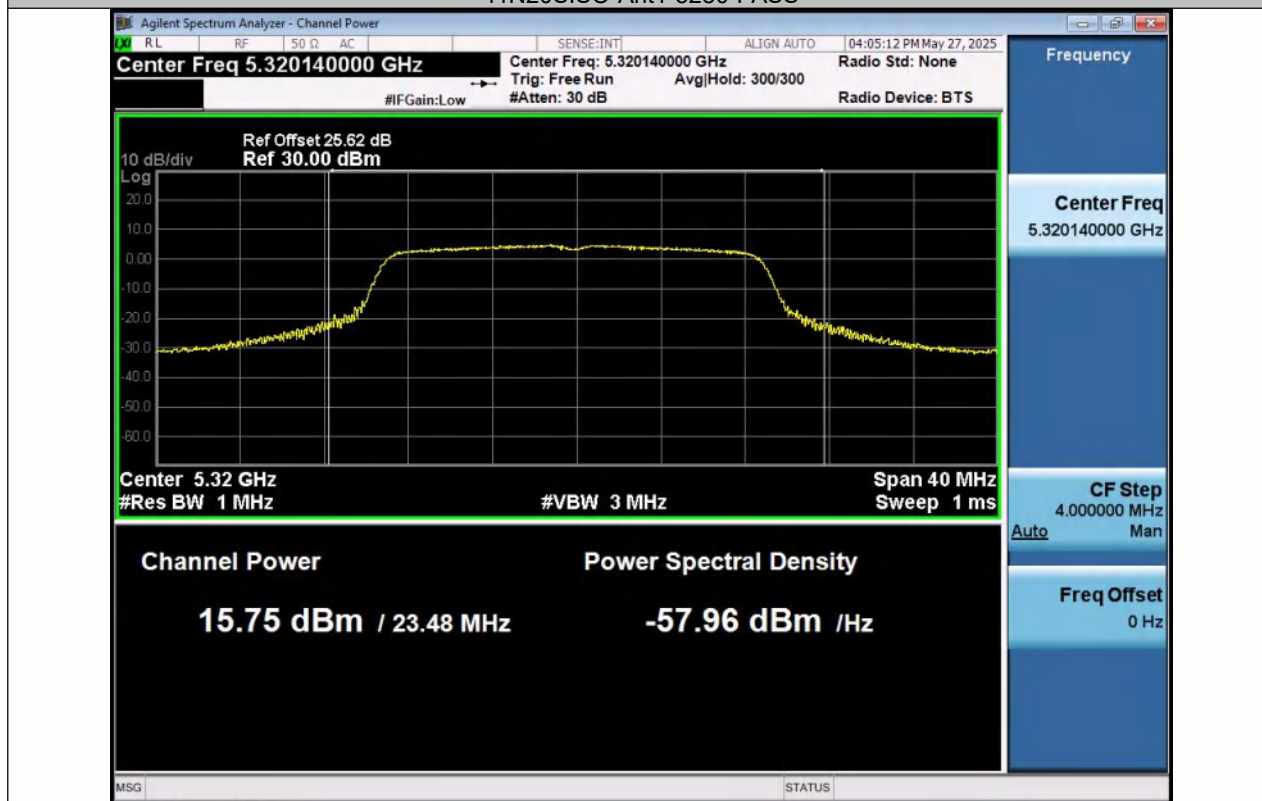
11N20SISO-Ant1-5320-PASS
