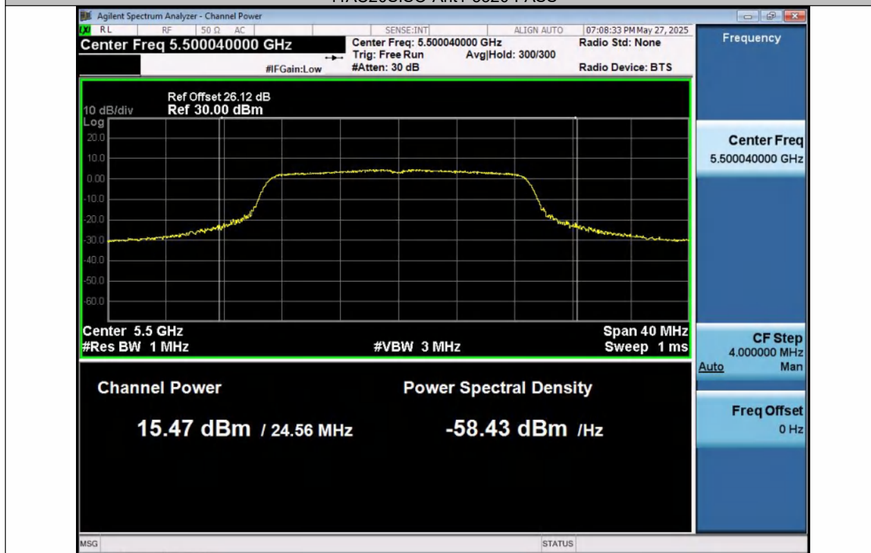
11AC20SISO-Ant1-5500-PASS
