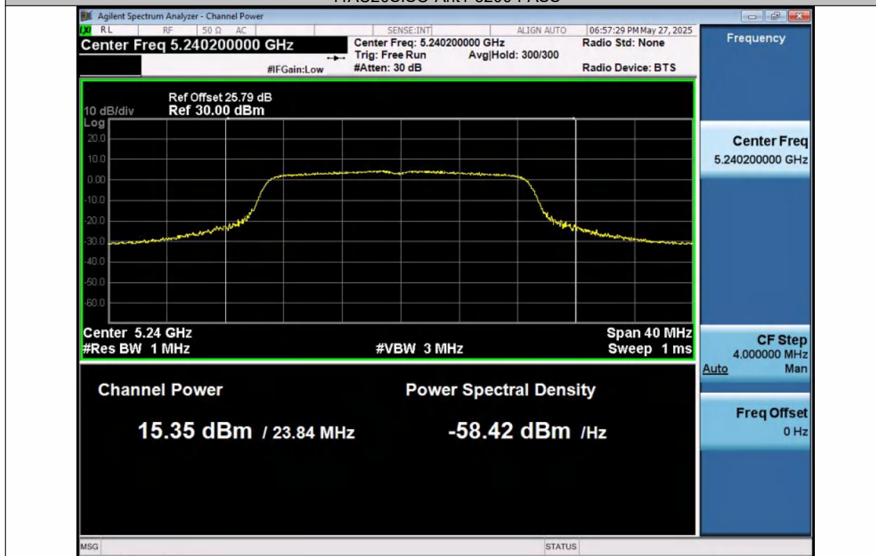
11AC20SISO-Ant1-5240-PASS
