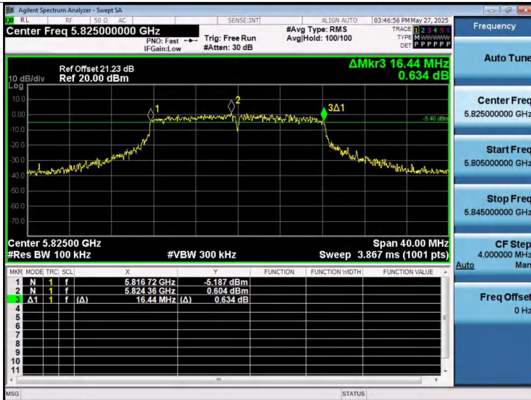
11A-Ant1-5825-PASS
