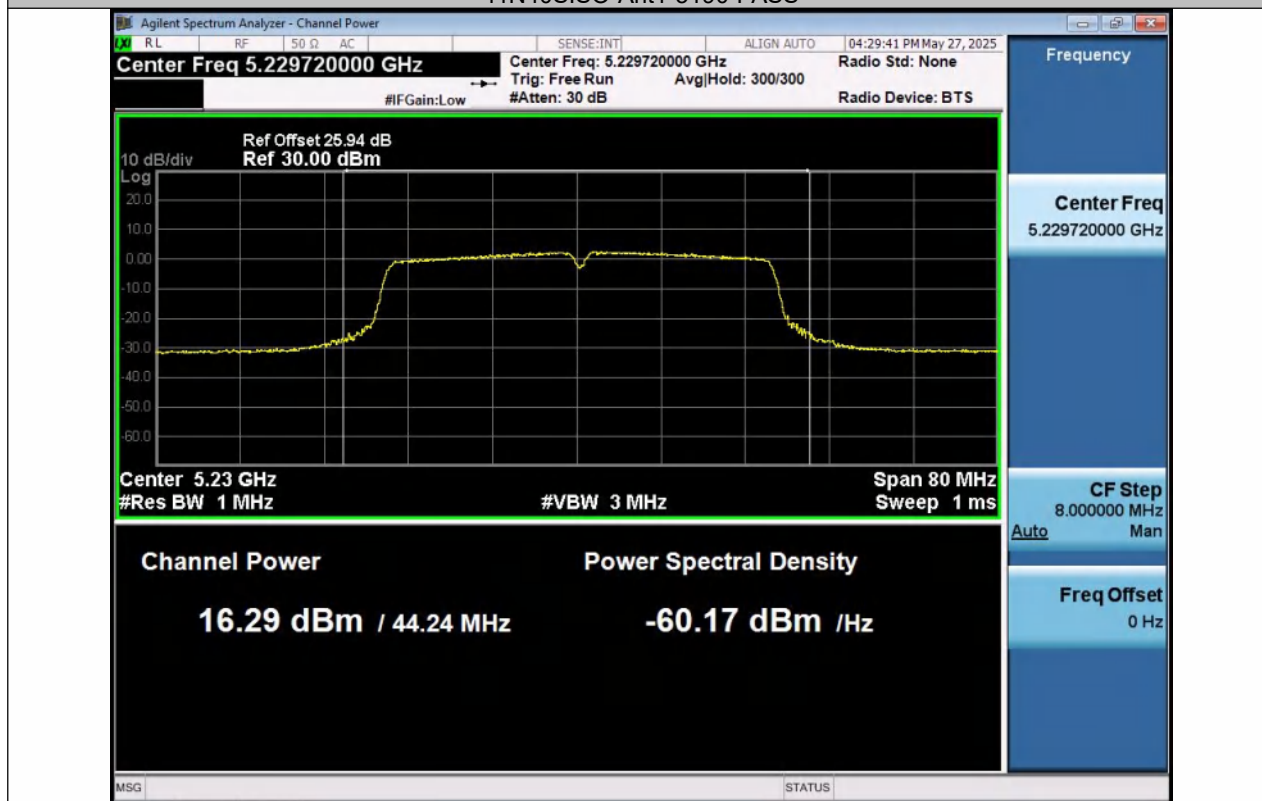
11N40SISO-Ant1-5230-PASS
