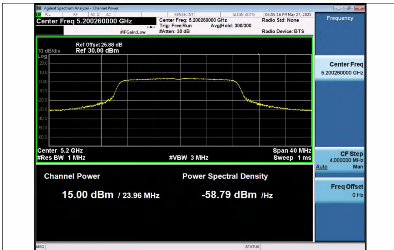
11AC20SISO-Ant1-5200-PASS
