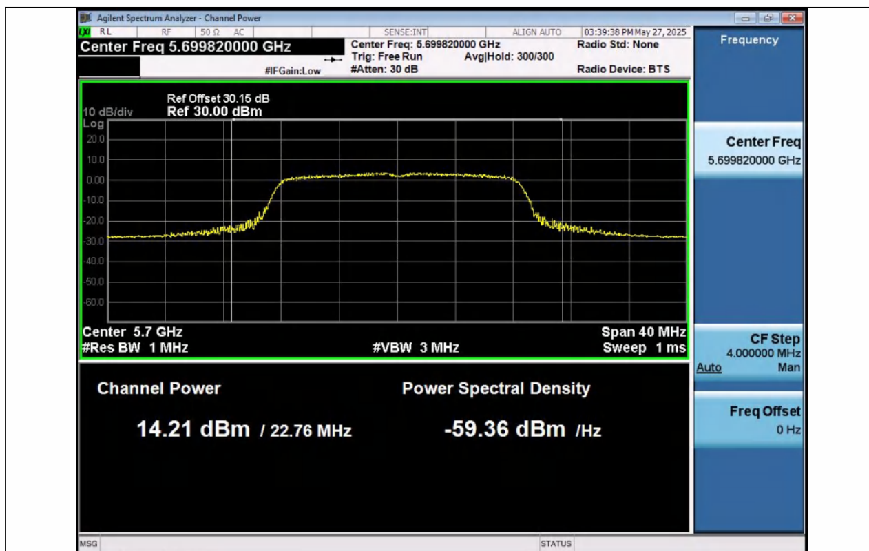
11A-Ant1-5700-PASS
