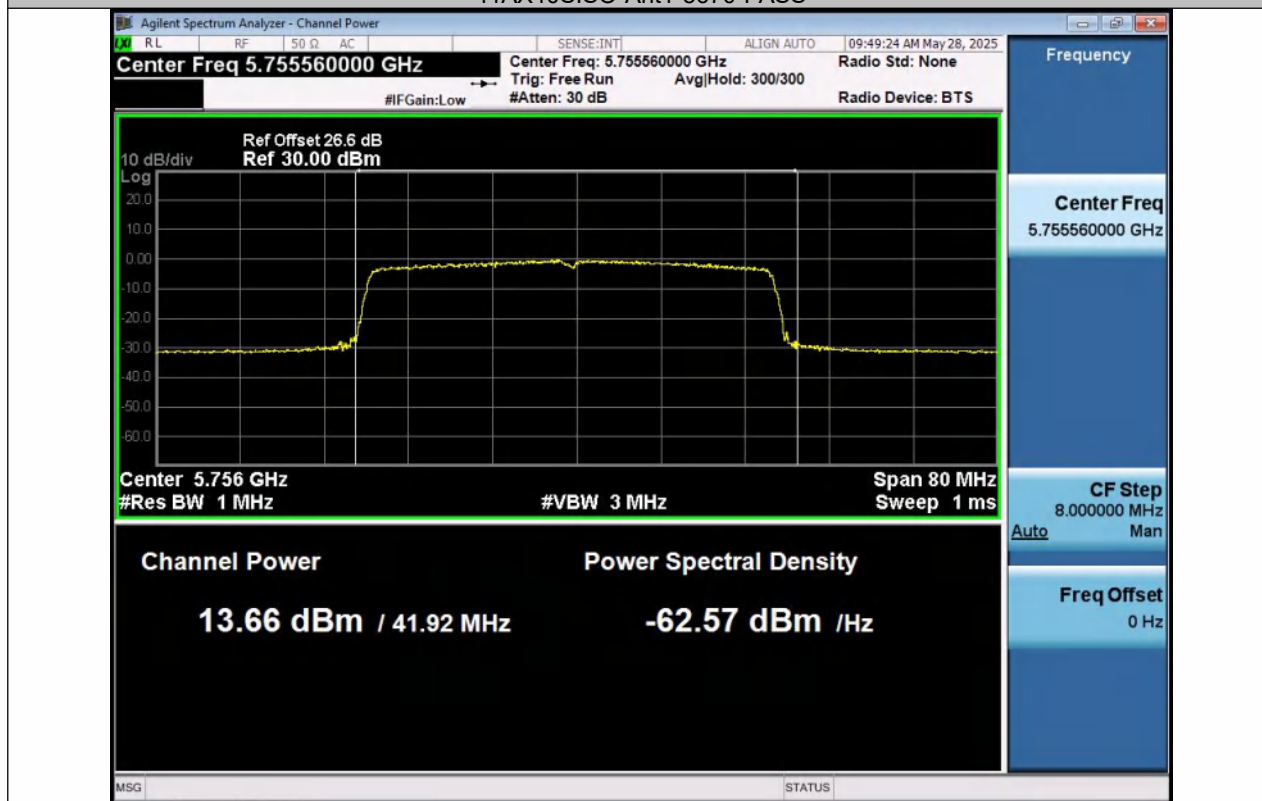
11AX40SISO-Ant1-5755-PASS
