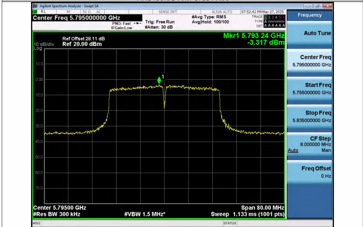
11AC40SISO-Ant1-5795-PASS
