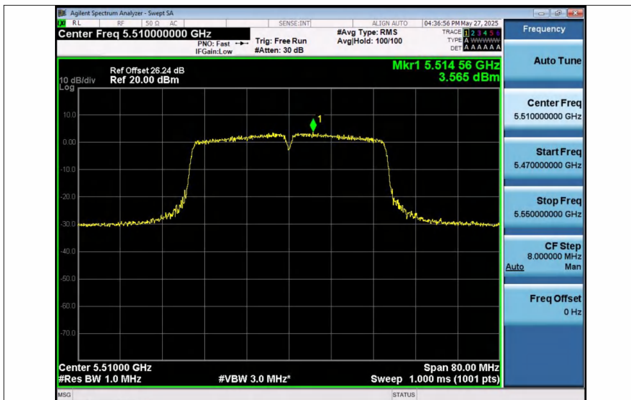
11N40SISO-Ant1-5510-PASS
