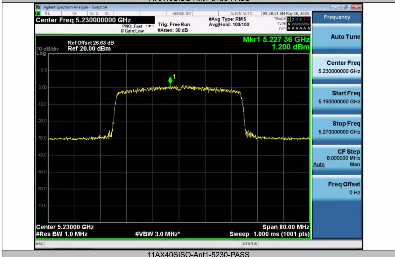
11AX40SISO-Ant1-5230-PASS
