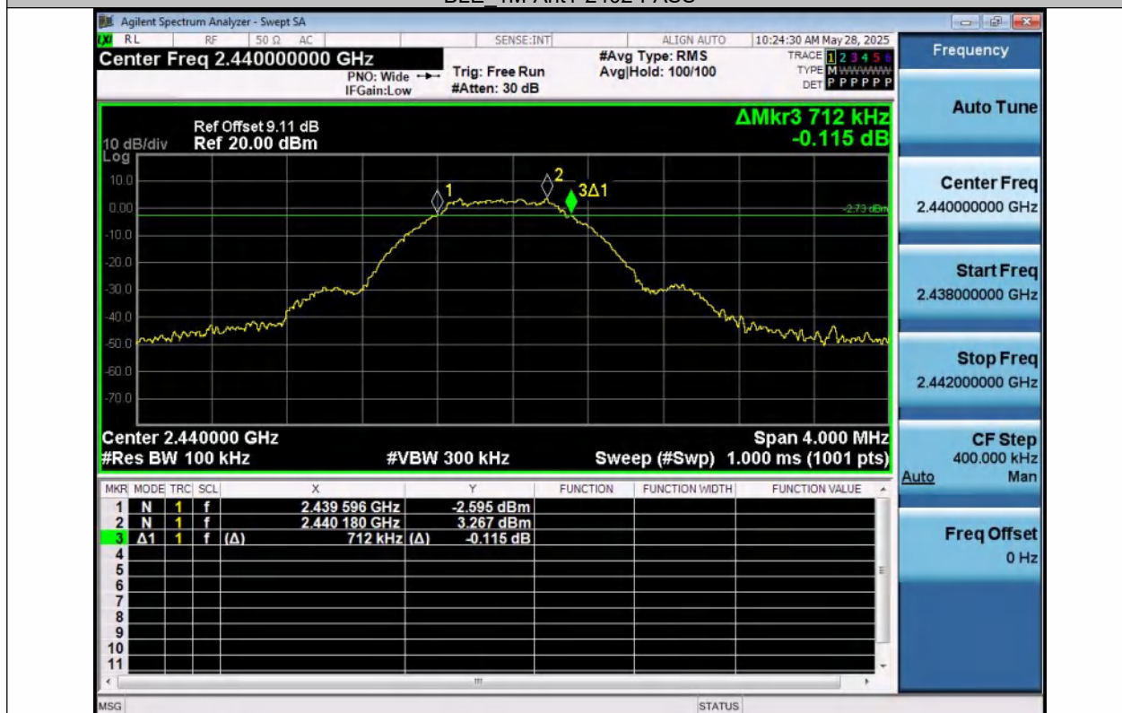
BLE_1M-Ant1-2440-PASS
