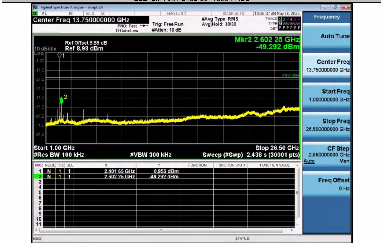
BLE_2M-Ant1-2402-1000~26500-PASS
