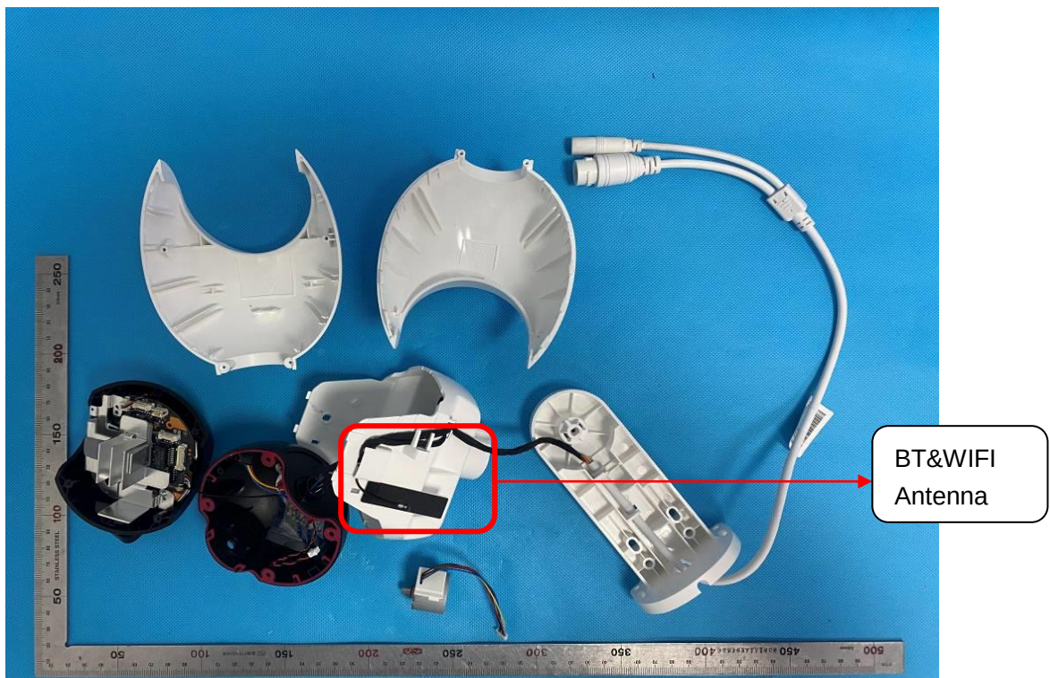
OPEN VIEW OF EUT(FIGURE 2)
