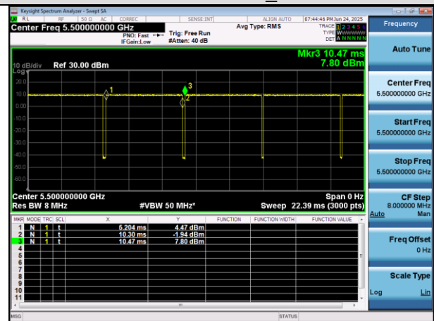
IEEE 802.11ac-VHT20_U-NII 2C
