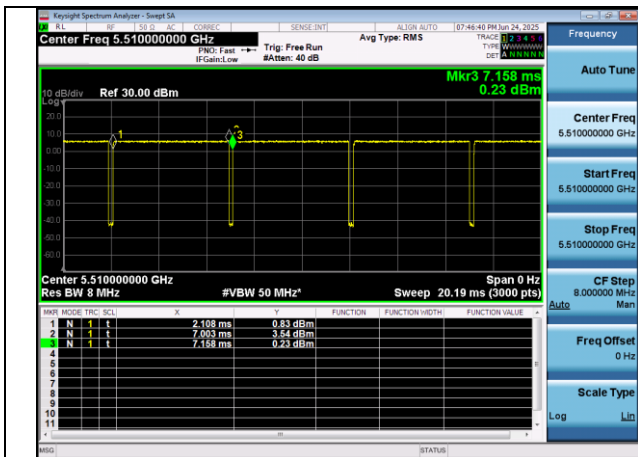
IEEE 802.11ac-VHT40_U-NII 2C
