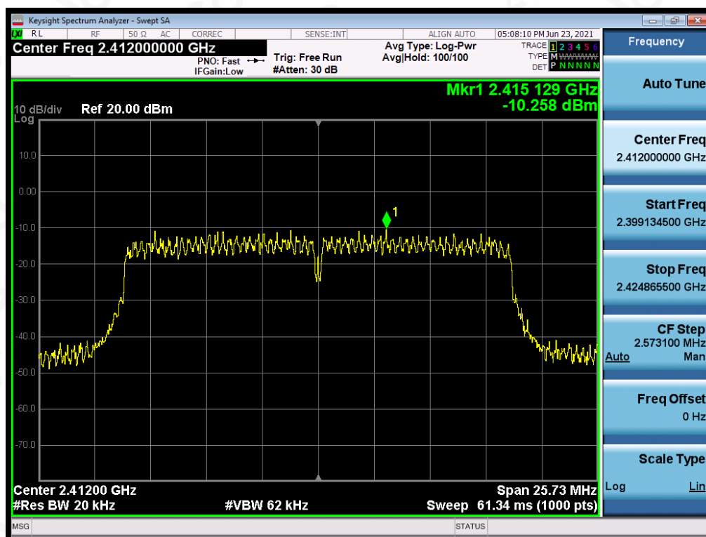
Test Graph 802.11n20 ANT1 2412 MCS0 PSD
