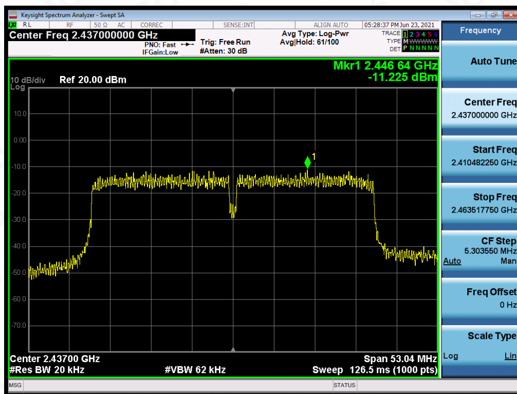
Test_Graph_802.11n40_ANT1_2437_MCS0_PSD
