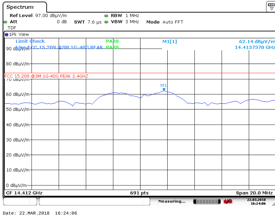
6 th harmonic – ch2402MHz, HP – PK
