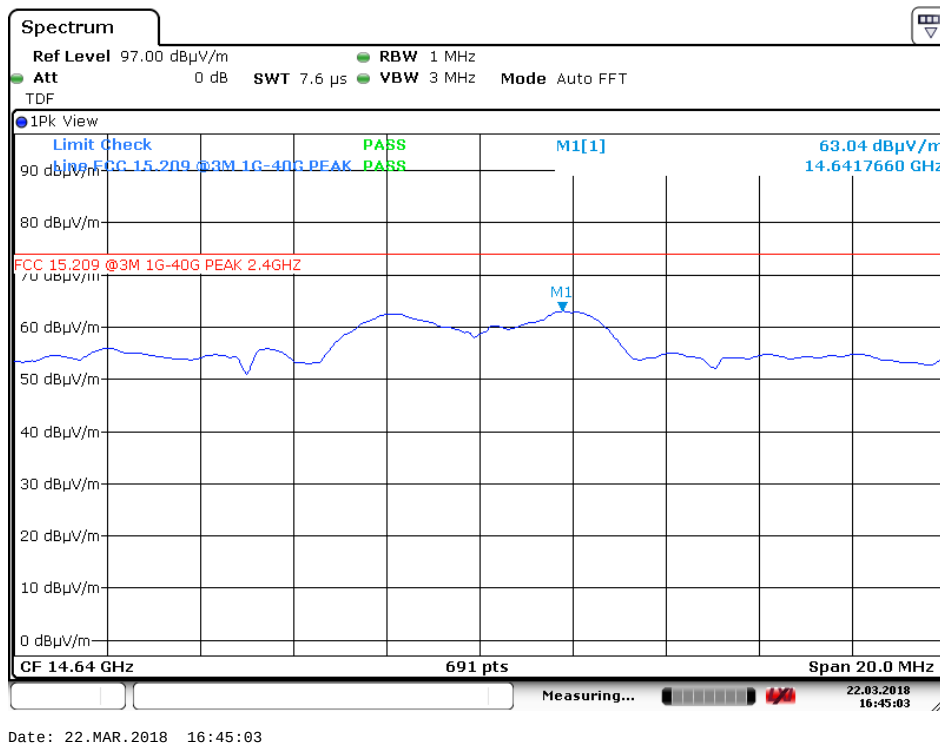
6 th harmonic – ch2440MHz, HP – PK
