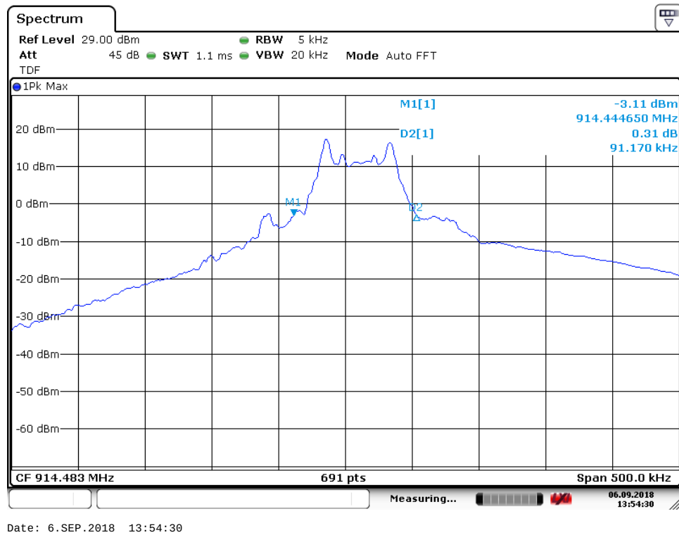
20 dB Bandwidth, ch50 (Air modem)
