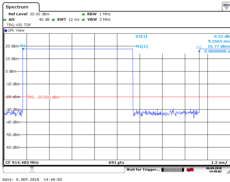
Sequence time (Air modem)
