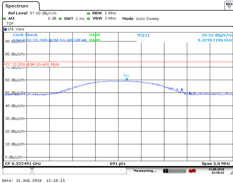
7 th harmonic – ch1, VP – PK (Air modem)
