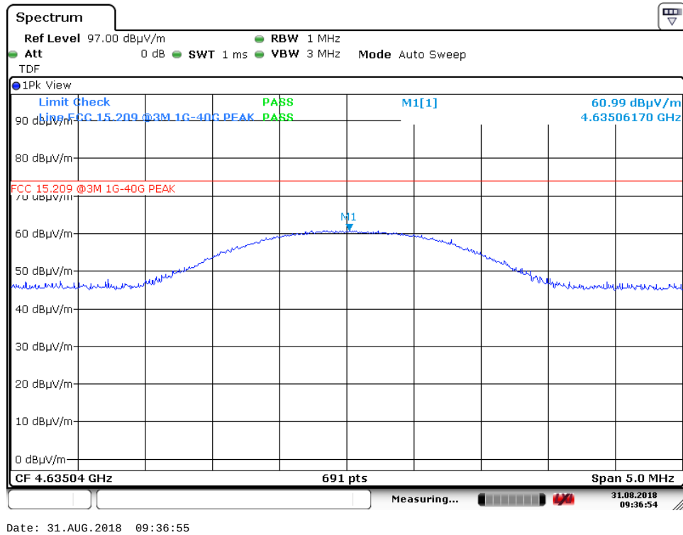
5 th harmonic – ch100, VP – PK (Air modem)
