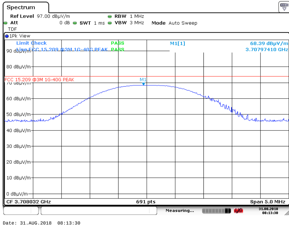
4 th harmonic – ch100, VP – PK (Ground modem)
