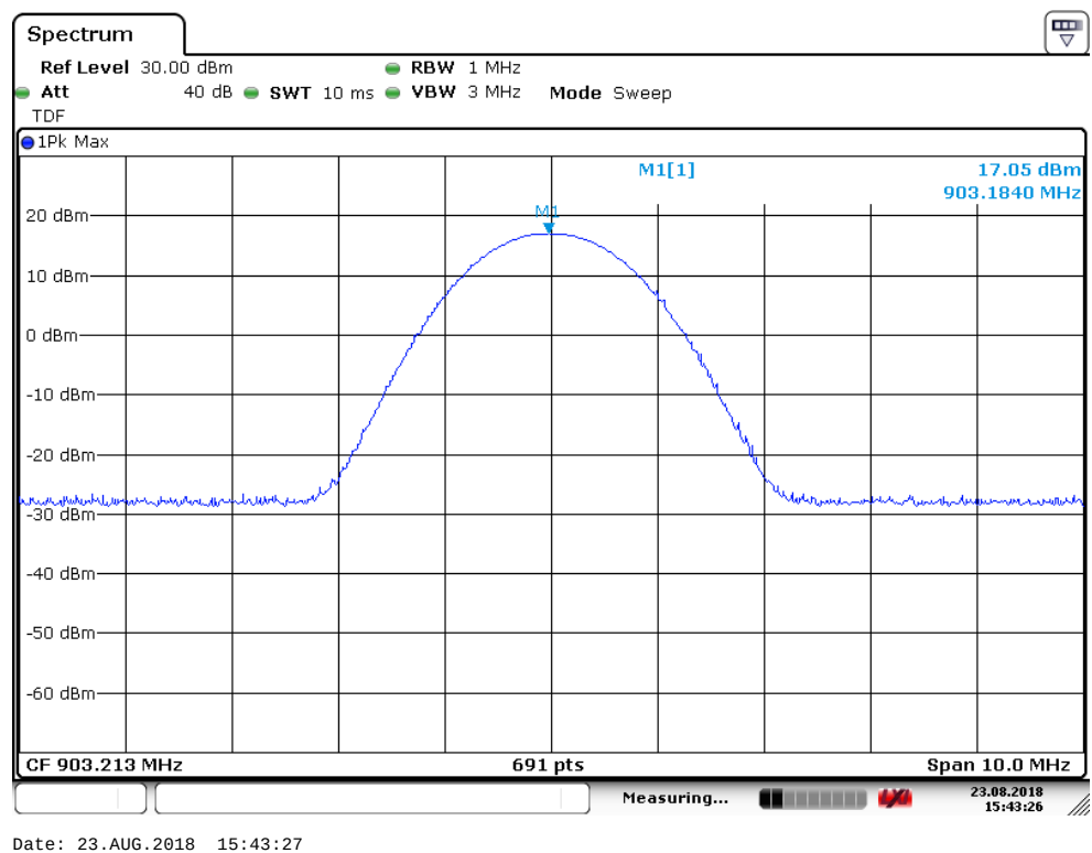
Conducted power – ch1 (Ground modem)
