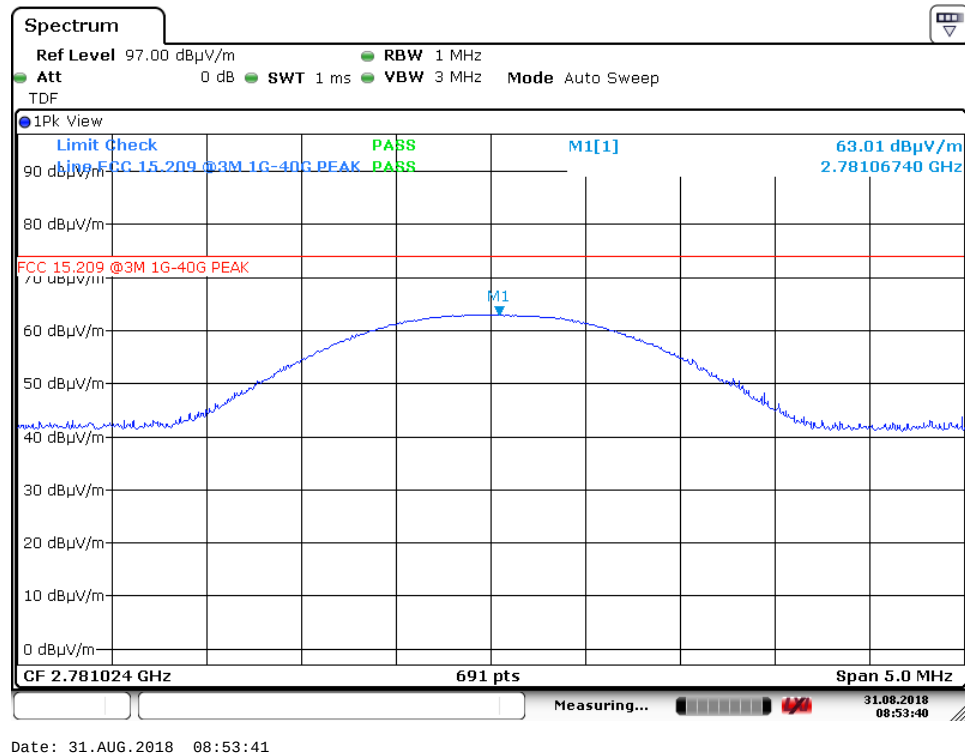
3 rd harmonic – ch100, VP – PK (Ground modem)
