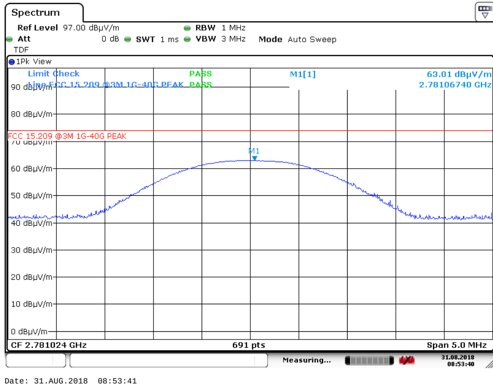
3 rd harmonic – ch100, VP – PK (Air modem)
