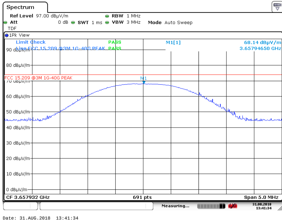
4 th harmonic – ch50, VP – PK (Air modem)
