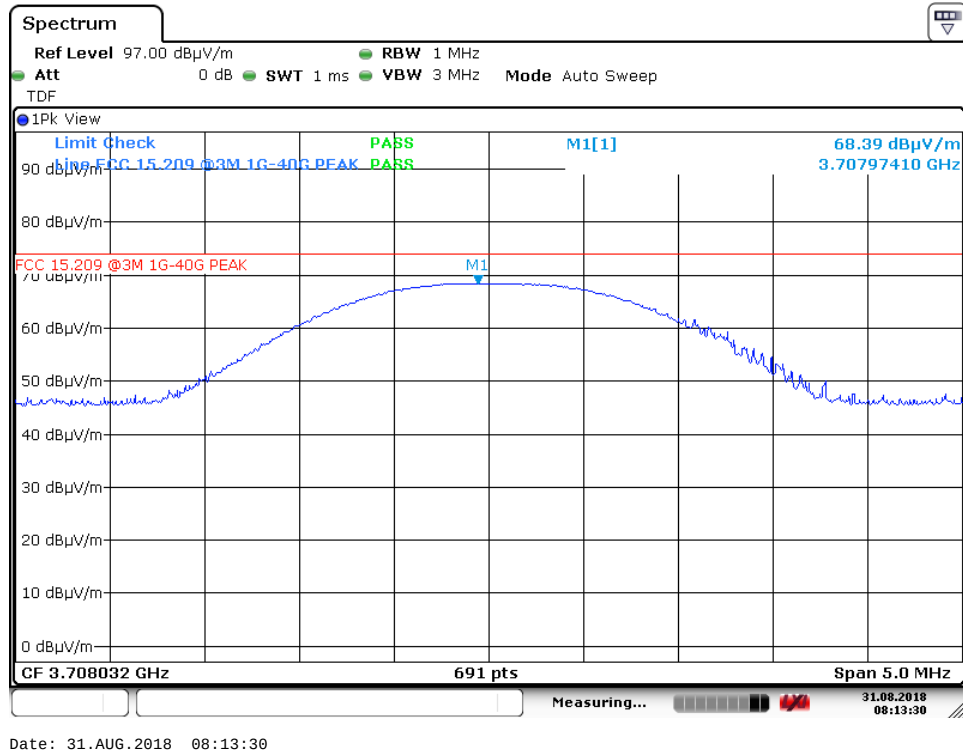
4 th harmonic – ch100, VP – PK (Air modem)
