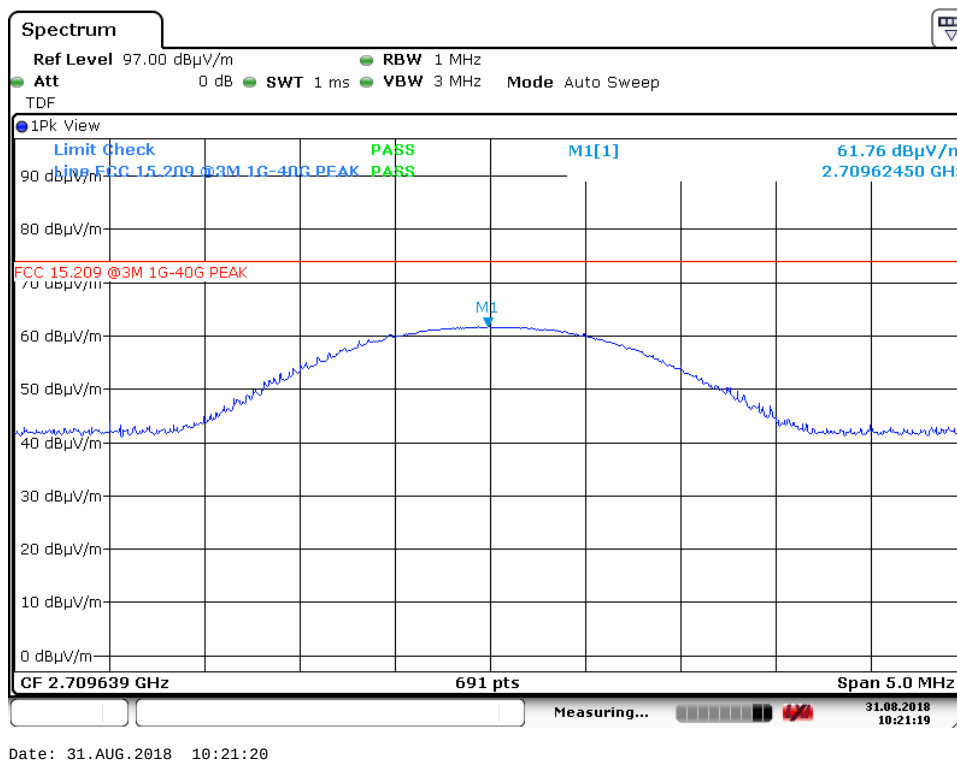
3 rd harmonic – ch1, VP – PK (Ground modem)
