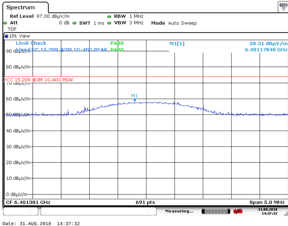
7 th harmonic – ch50, VP – PK (Air modem)
