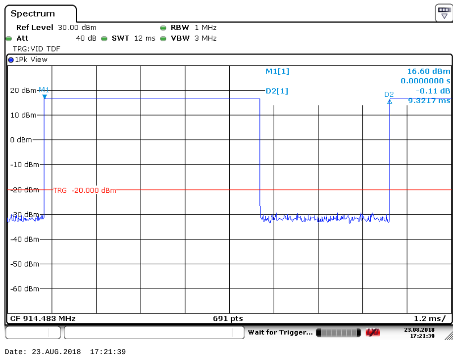
Sequence time (Ground modem)
