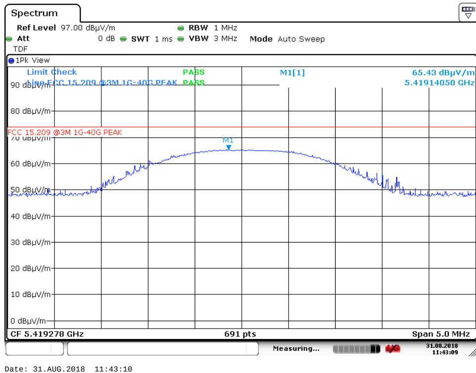
6 th harmonic – ch1, HP – PK (Ground modem)
