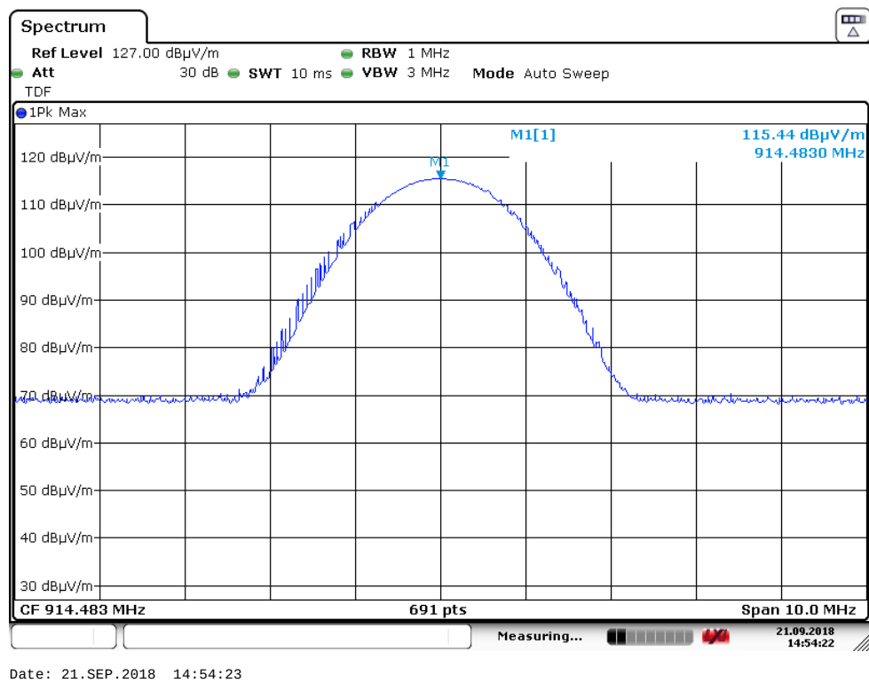
Radiated field strength, VP, ch50 (Air modem)
