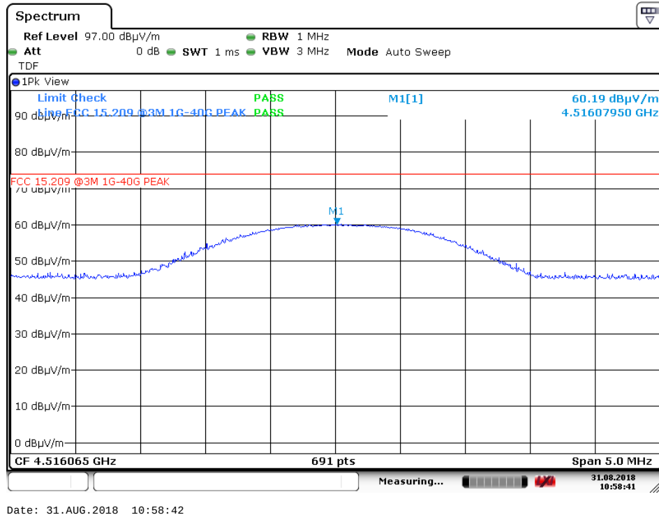
5 th harmonic – ch1, VP – PK (Ground modem)
