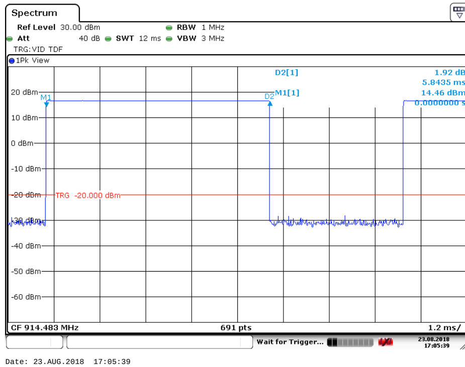
Burst length (Ground modem)
