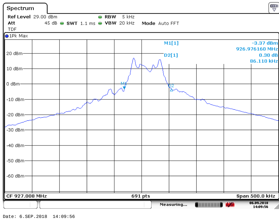
20 dB Bandwidth, ch100 (Air modem)
