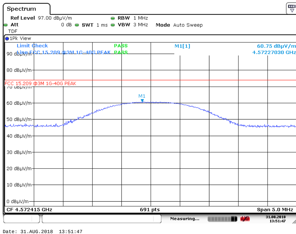
5 th harmonic – ch50, VP – PK (Air modem)
