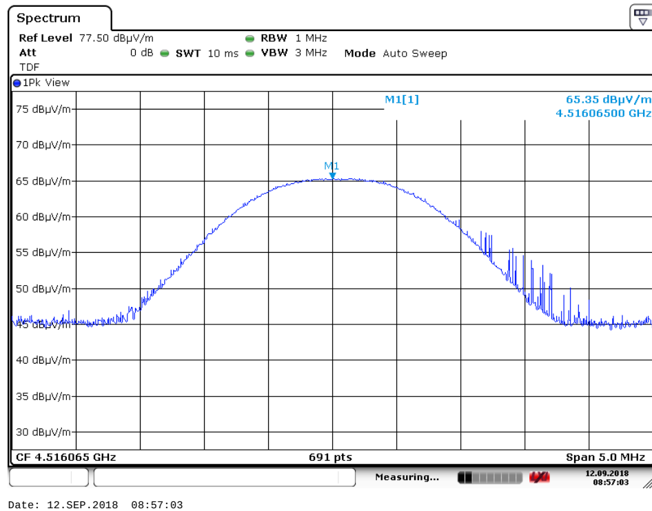
5 th harmonic – ch1, VP – PK (Air modem)
