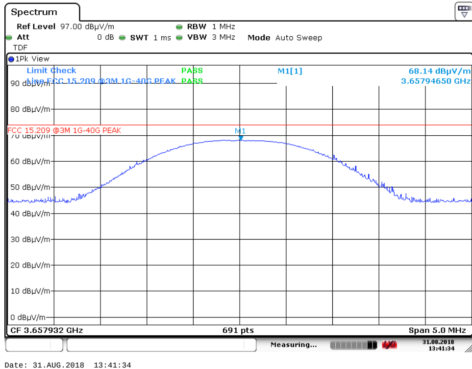
4 th harmonic – ch50, VP – PK (Ground modem)
