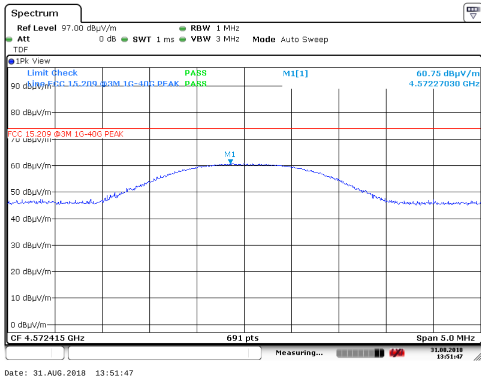
5 th harmonic – ch50, VP – PK (Ground modem)
