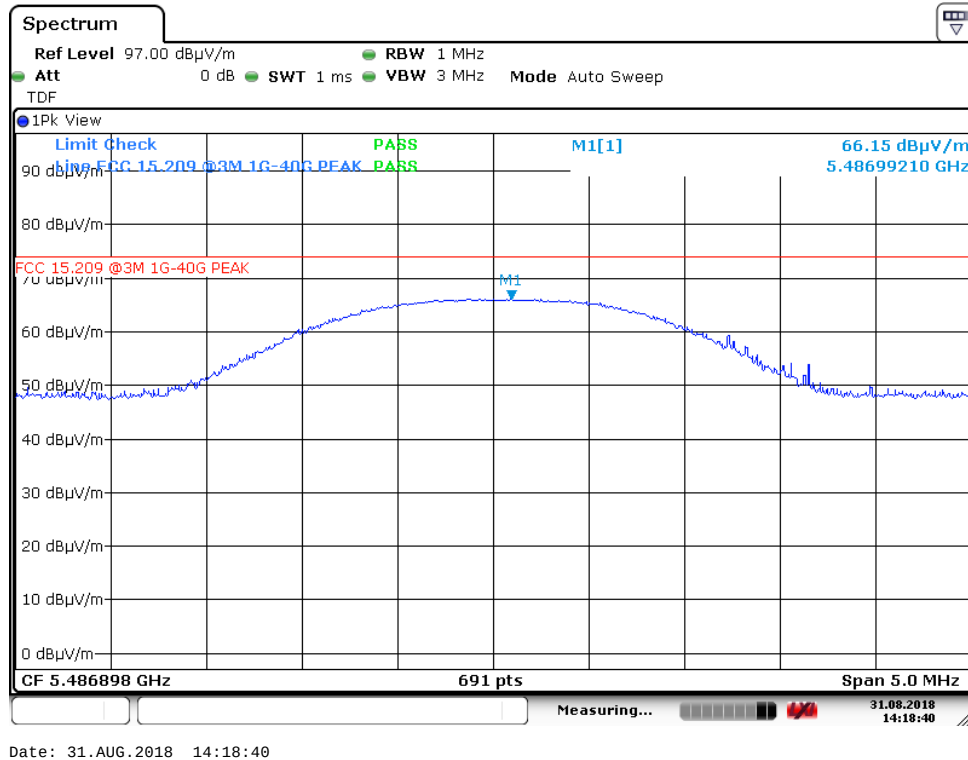
6 th harmonic – ch50, HP – PK (Ground modem)
