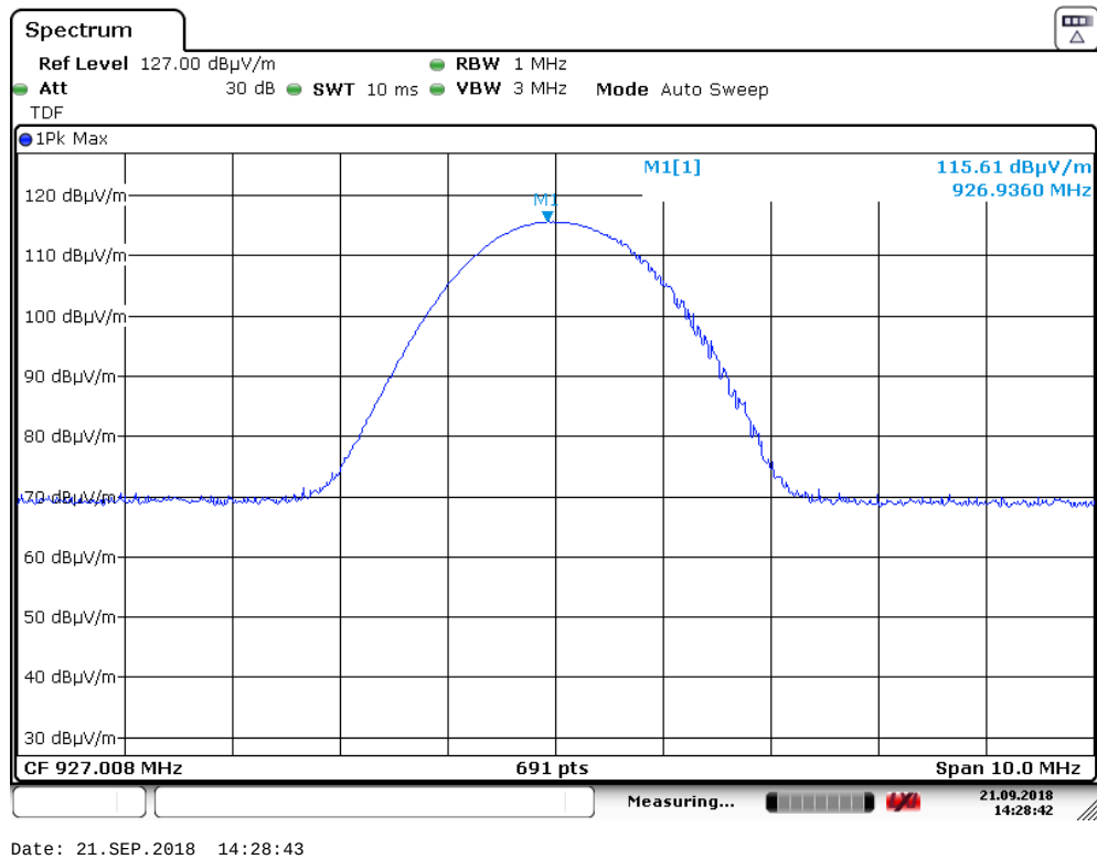
Radiated field strength, HP, ch100 (Ground modem)
