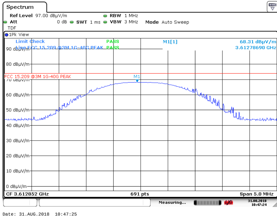
4 th harmonic – ch1, VP – PK (Ground modem)
