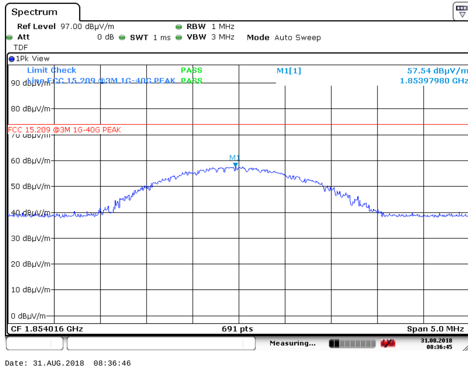
2 nd harmonic – ch100, HP – PK (Ground modem)
