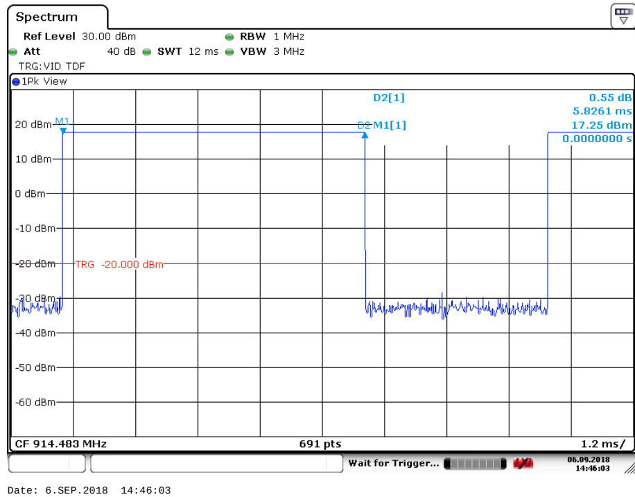
Burst length (Air modem)
