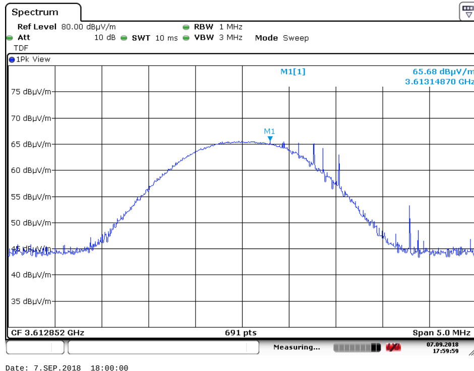
4 th harmonic – ch1, VP – PK (Air modem)
