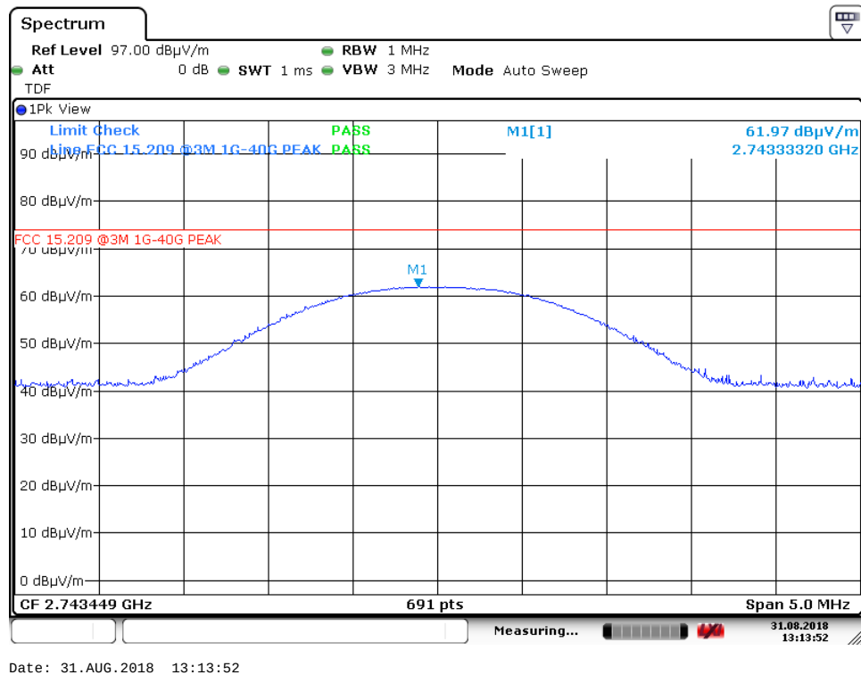
3 rd harmonic – ch50, VP – PK (Ground modem)
