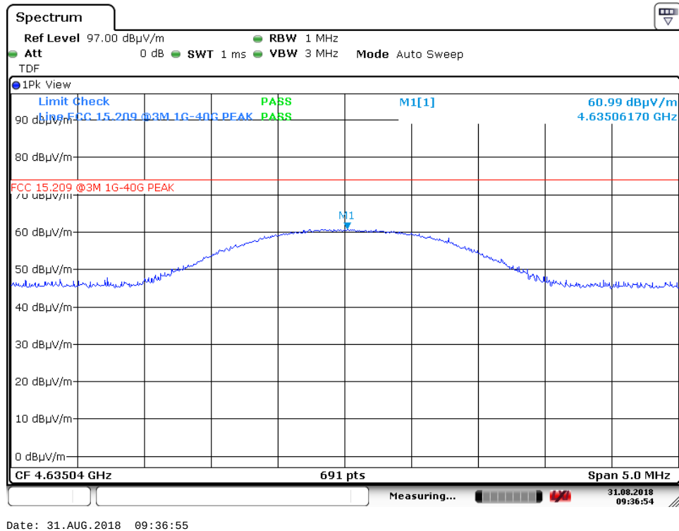
5 th harmonic – ch100, VP – PK (Ground modem)
