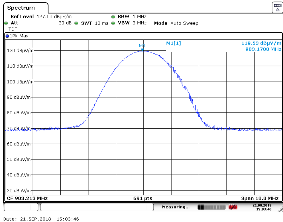
Radiated field strength, VP, ch1 (Air modem)
