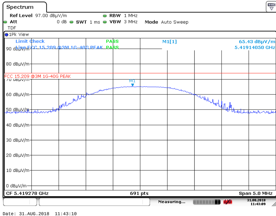
6 th harmonic – ch1, HP – PK (Air modem)
