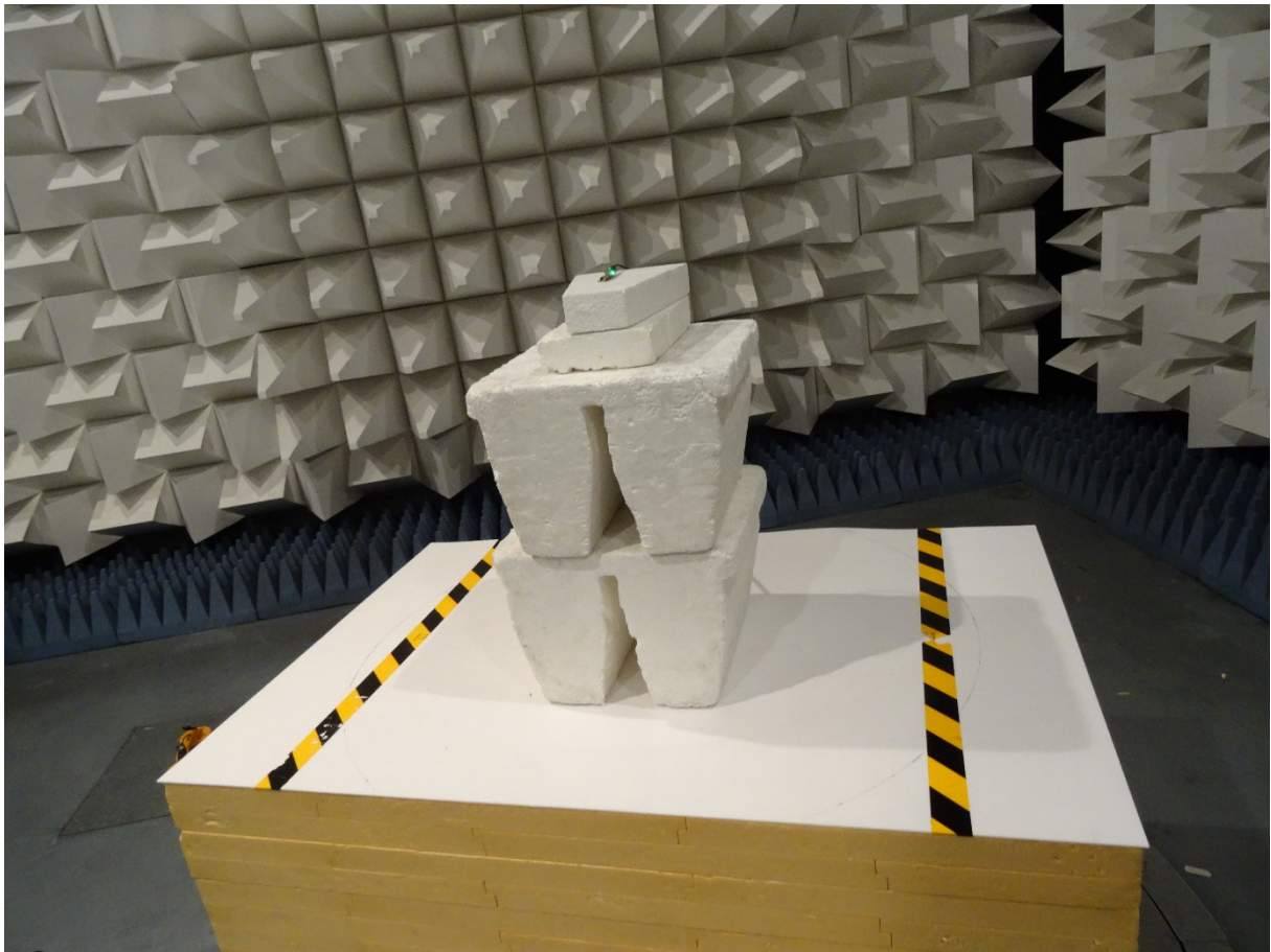
Spurious radiated emission setup over 1GHz (Ground modem)
