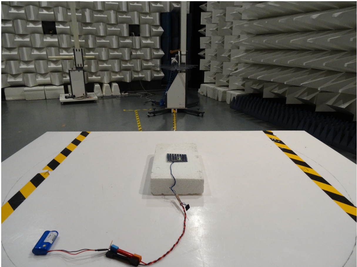
Spurious radiated emission 200 MHz - 1000 MHz (Air modem)
