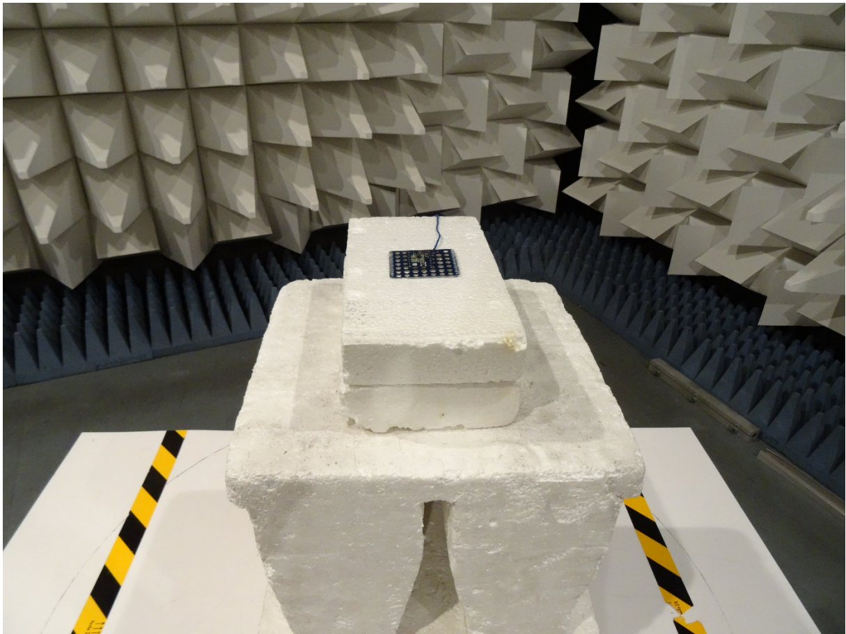
Spurious radiated emission setup over 1GHz (Air modem)
