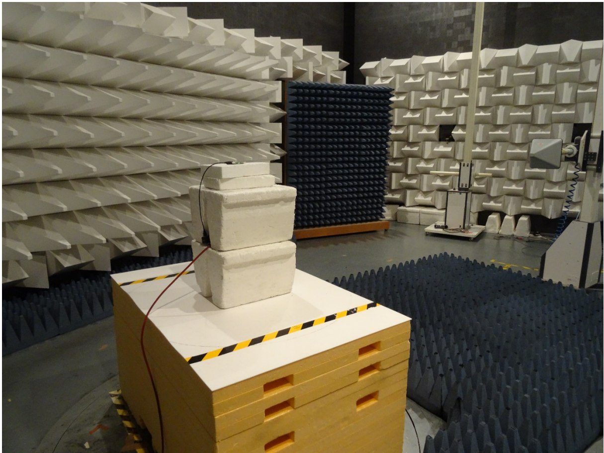
Spurious radiated emission 1GHz - 10 GHz (Ground modem)
