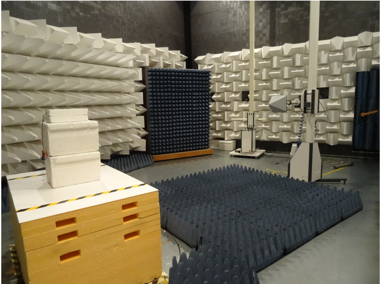
Spurious radiated emission 1GHz - 10 GHz (Air modem)
