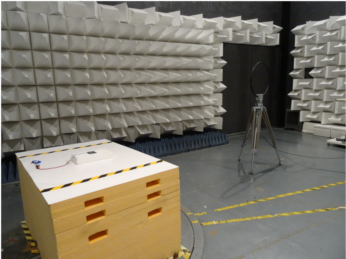
Spurious radiated < 30MHz (Air modem)
