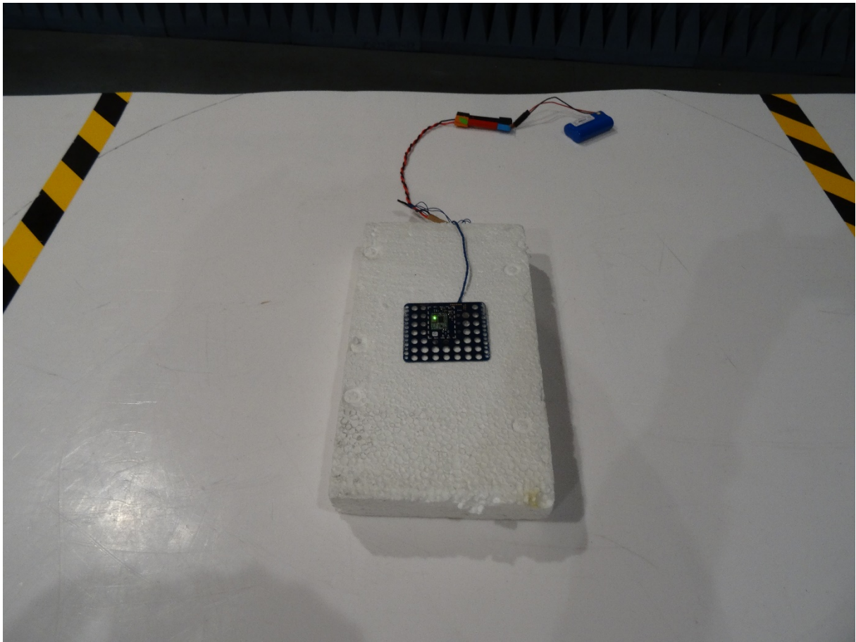
Spurious radiated emission setup below 1GHz (Air modem)
