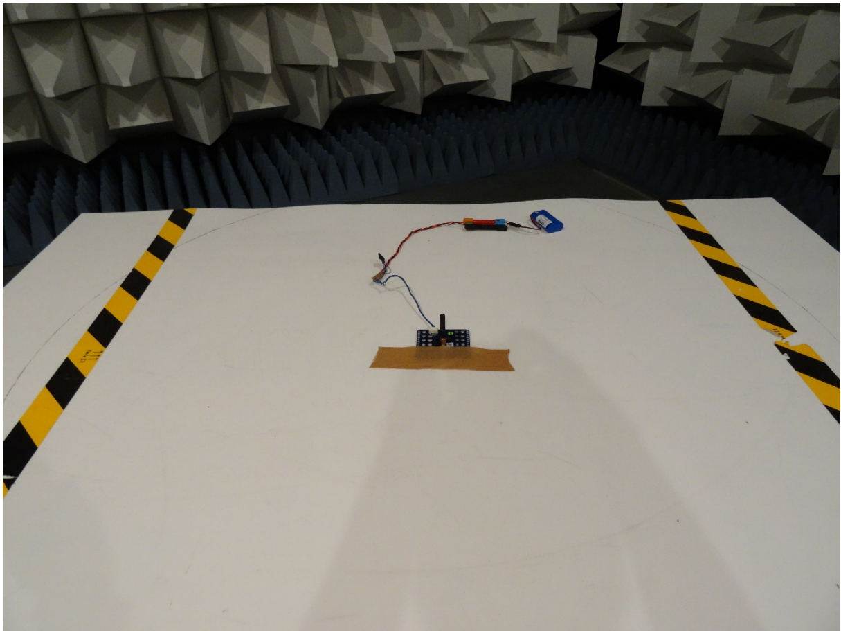
TX radiated emission setup (Air modem)
