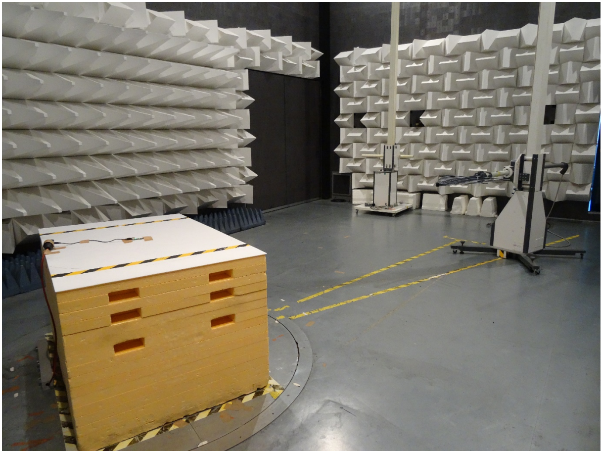
Spurious radiated emission 200 MHz - 1000 MHz (Ground modem)
