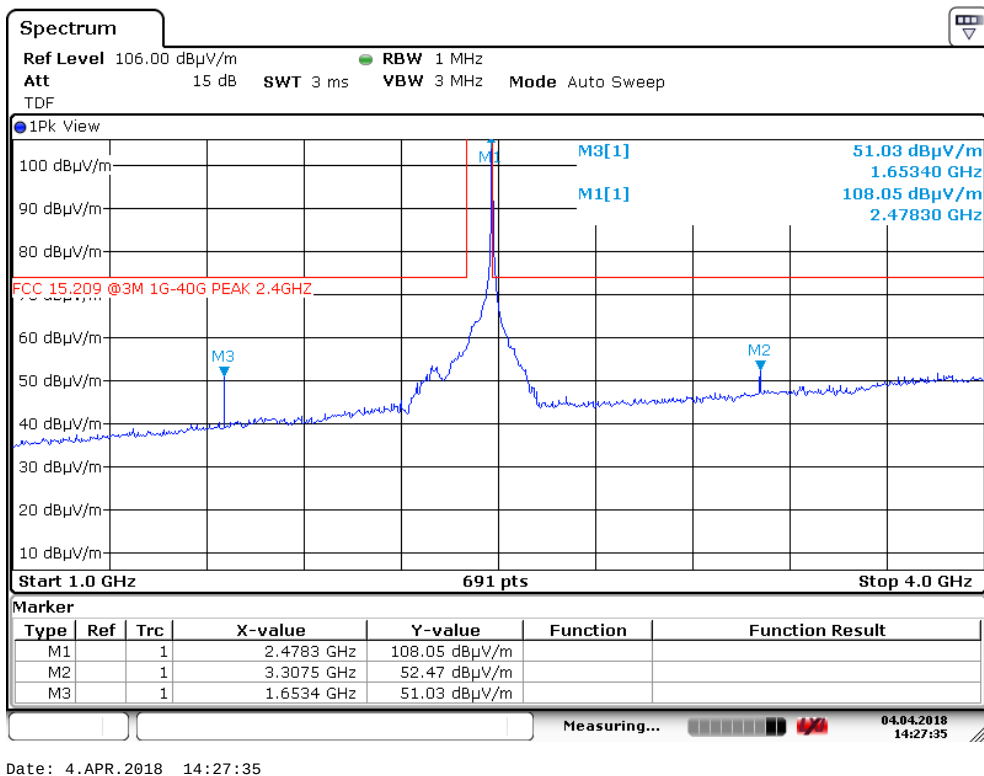
Radiated Emissions ch. 2479 MHz, 1 – 4 GHz, HP, @3m – Pre-scan, antenna 1
