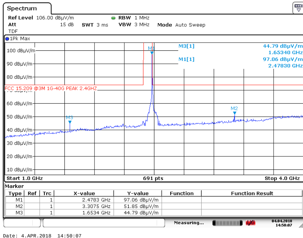
Radiated Emissions ch. 2479 MHz, 1 – 4 GHz, VP, @3m – Pre-scan, antenna 1
