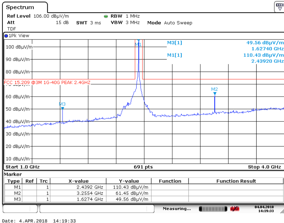
Radiated Emissions ch. 2440 MHz, 1 – 4 GHz, HP, @3m – Pre-scan, antenna 1
