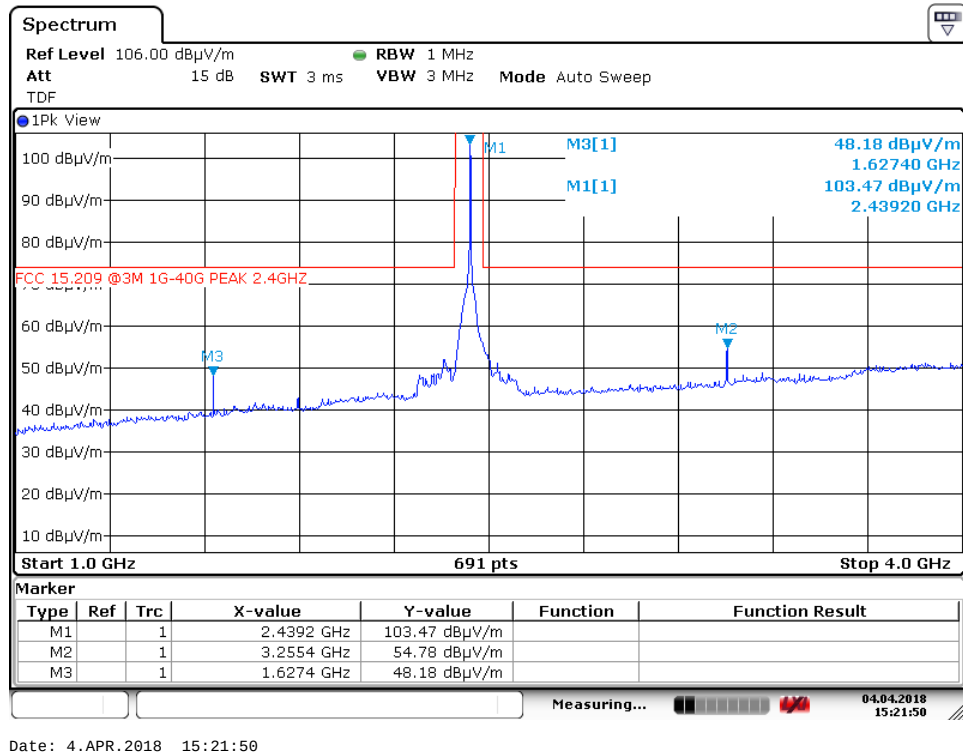
Radiated Emissions ch. 2440 MHz, 1 – 4 GHz, VP, @3m – Pre-scan, antenna 1
