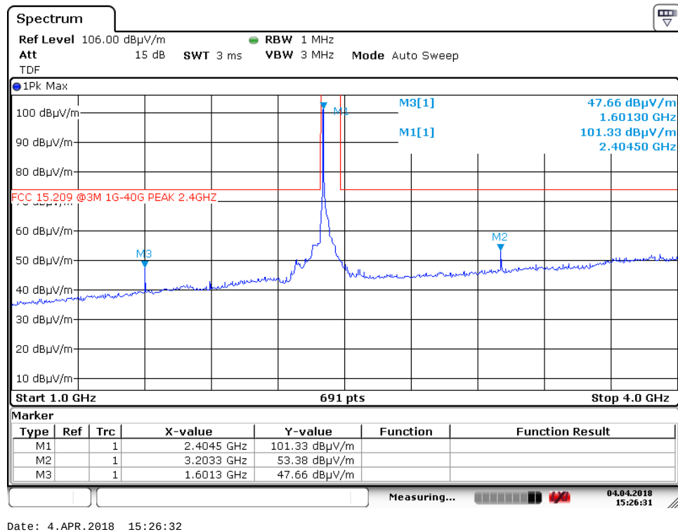
Radiated Emissions, 2402 MHz, 1 – 4 GHz, VP, @3m – Pre-scan, antenna 1
