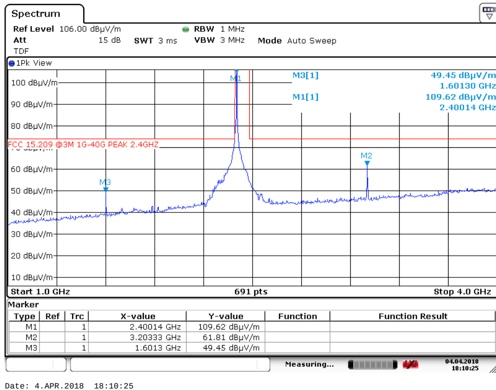
Radiated Emissions, 2402 MHz, 1 – 4 GHz, HP, @3m – Pre-scan, antenna 1
