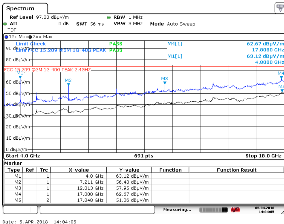
Radiated Emissions ch. 2402 MHz, 4 – 18 GHz, HP, @3m – Pre-scan, antenna 1
