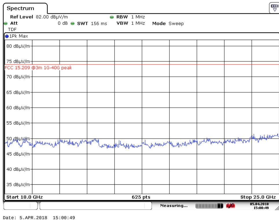
Radiated Emissions ch. 2440 MHz, 18 – 25 GHz, HP, @3m – Pre-scan, antenna 1
