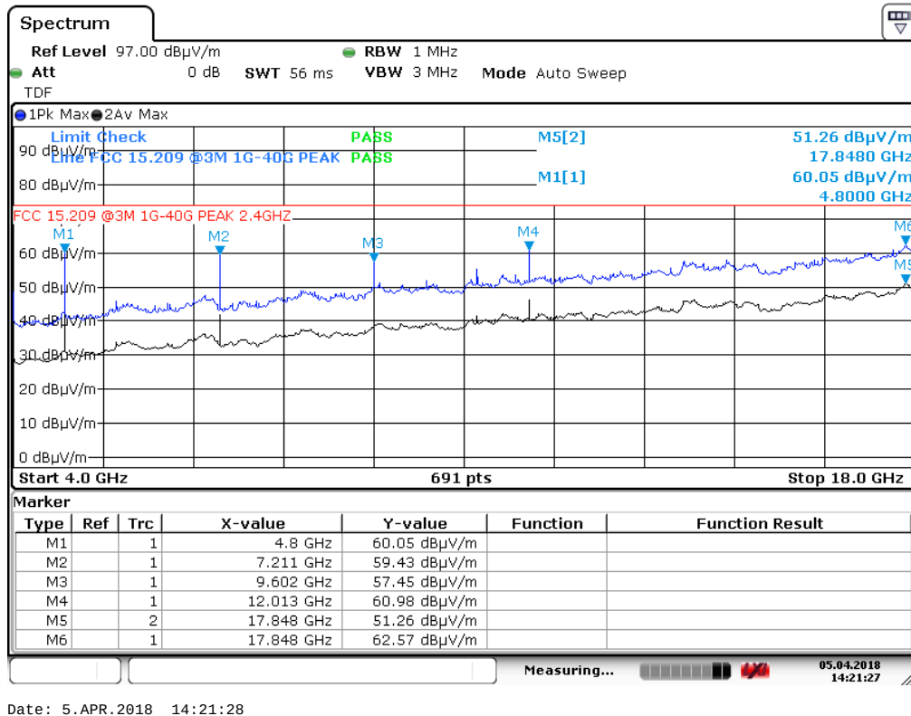
Radiated Emissions ch. 2402 MHz, 4 – 18 GHz, VP, @3m – Pre-scan, antenna 1
