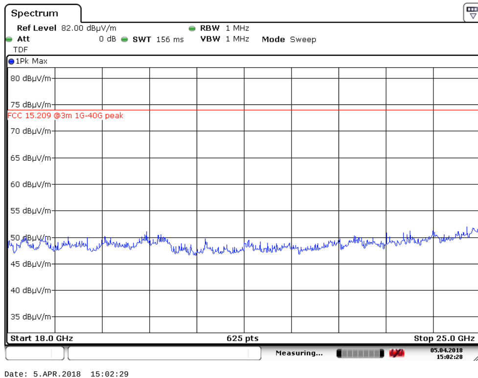
Radiated Emissions ch. 2440 MHz, 18 – 25 GHz, VP, @3m – Pre-scan, antenna 1
