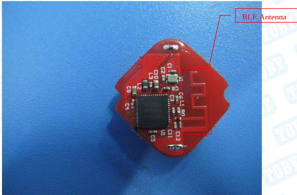
Photo 12 Appearance of PCB
