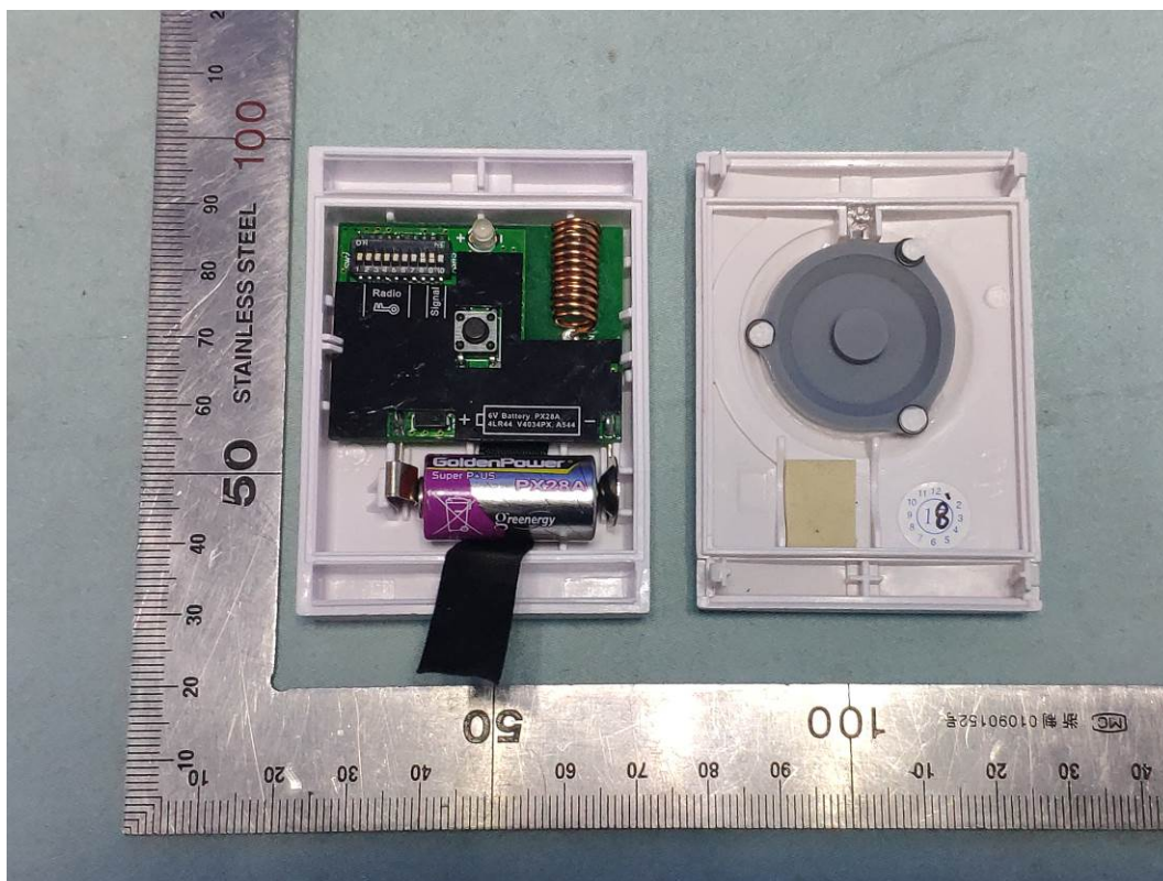
FIGURE 3 PUSH BUTTON TRANSMITTER (M/N: BE1240-433) COVER REMOVED
