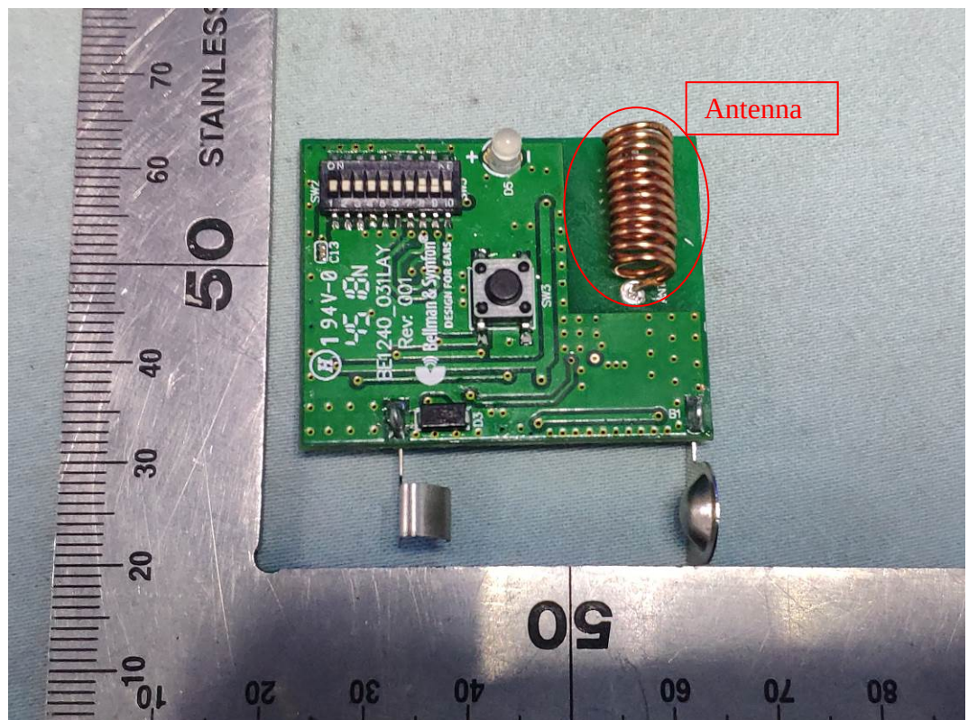
FIGURE 6 PUSH BUTTON TRANSMITTER (M/N: BE1240-433) ANTENNA
