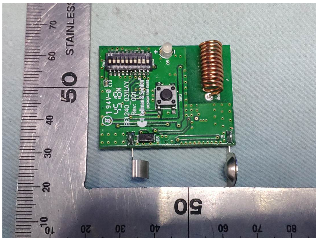
FIGURE 4 PUSH BUTTON TRANSMITTER (M/N: BE1240-433) MAIN BOARD(FRONT VIEW)
