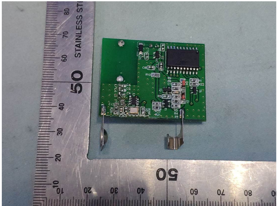
FIGURE 5 PUSH BUTTON TRANSMITTER (M/N: BE1240-433) MAIN BOARD(BACK VIEW)
