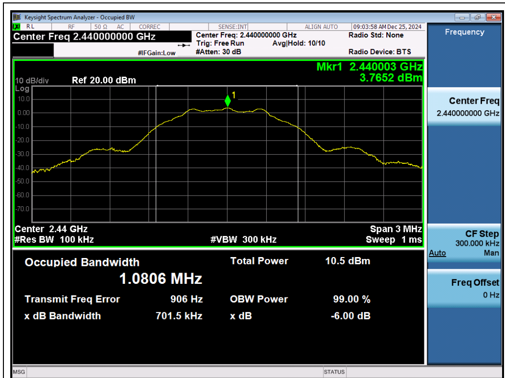
Test_Graph_LE1M_ANT1_2440_1Mbps_DTSSBW
