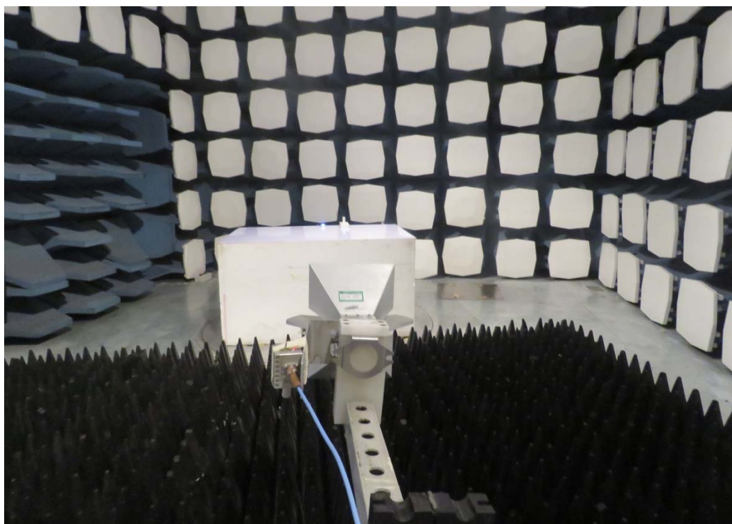
30MHz-1GHz
