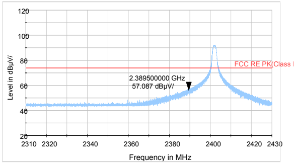
BLE Channel 0 Peak
