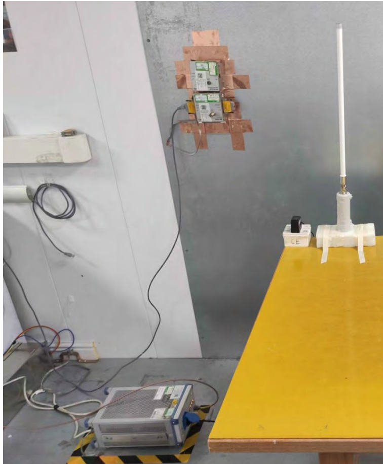
Conducted emissions
