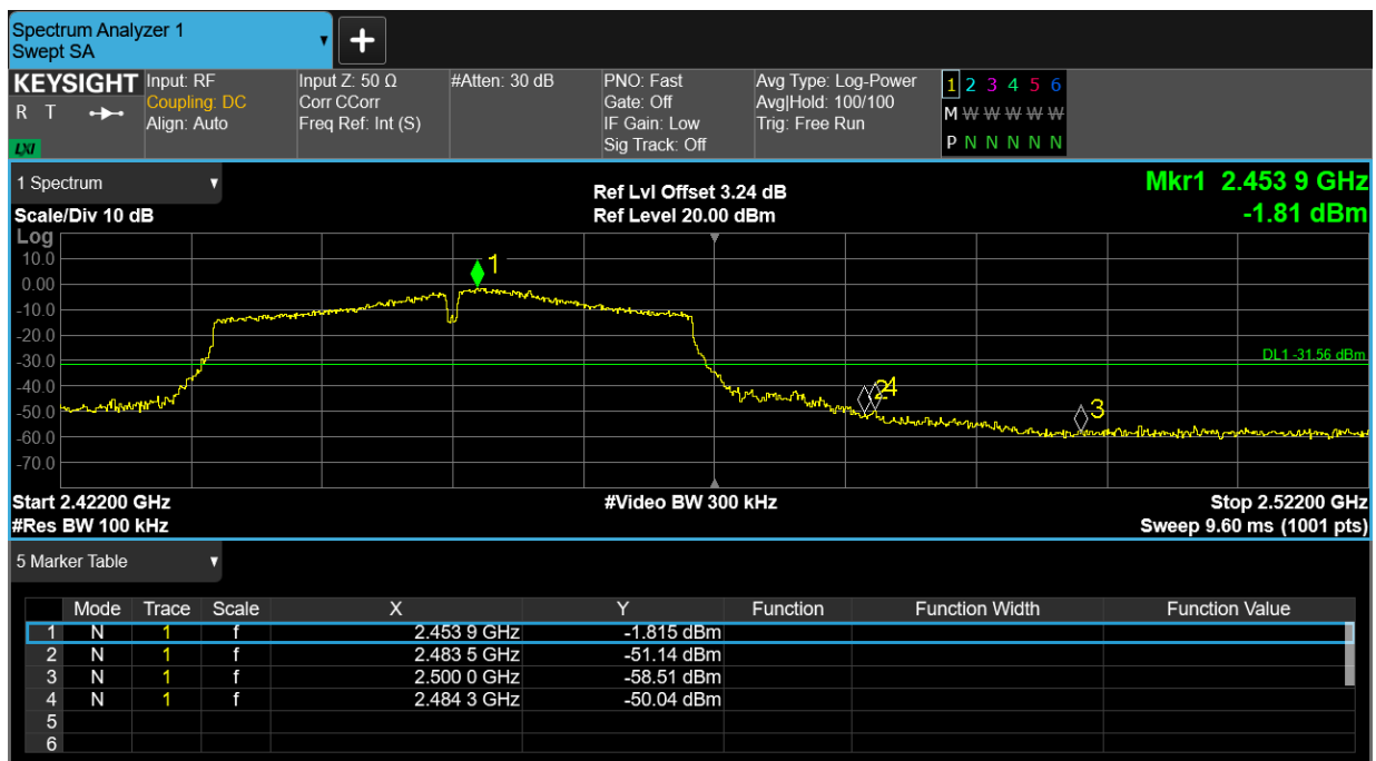
Band Edge NVNT n40 2452MHz Ant1 Emission
