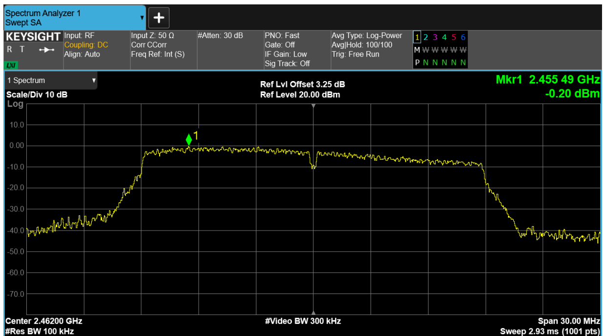
Tx. Spurious NVNT n20 2462MHz Ant1 Emission
