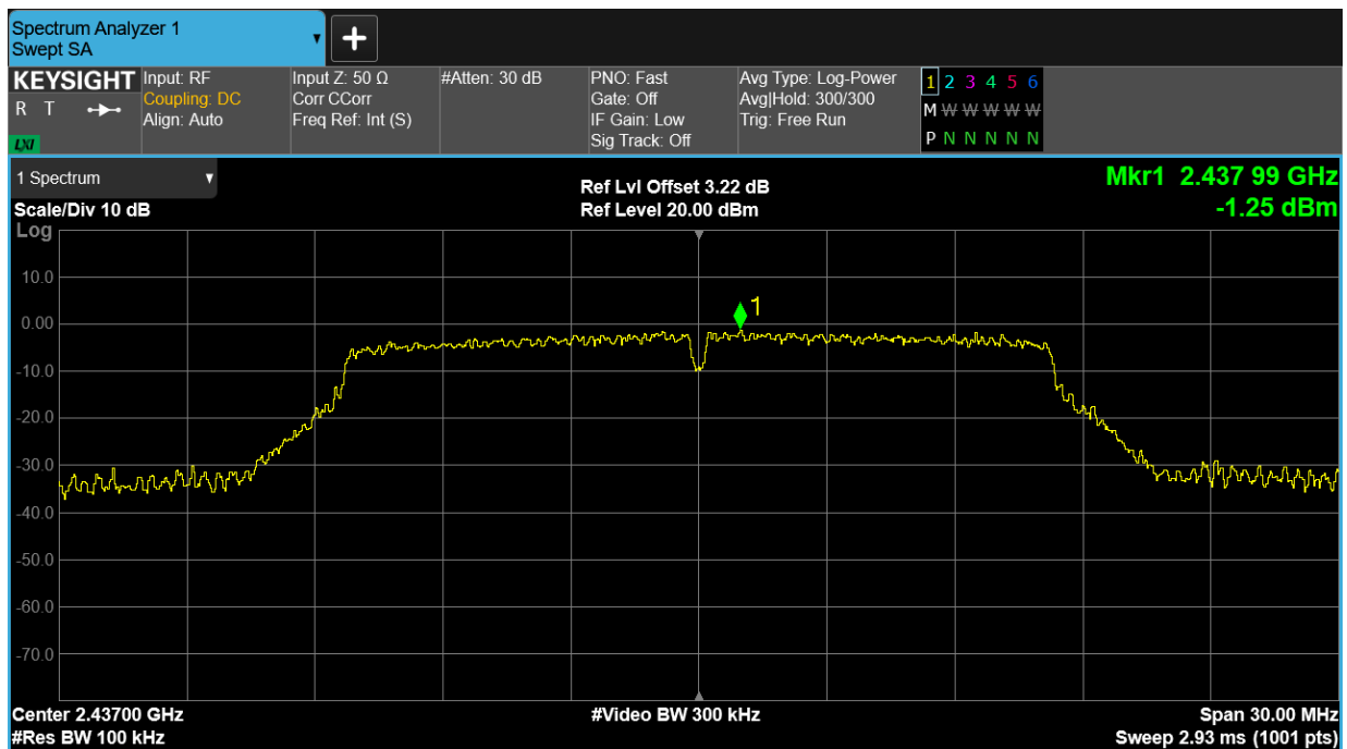
Tx. Spurious NVNT g 2437MHz Ant1 Emission
