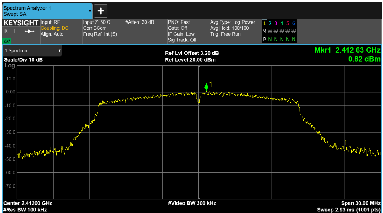
Tx. Spurious NVNT g 2412MHz Ant1 Emission
