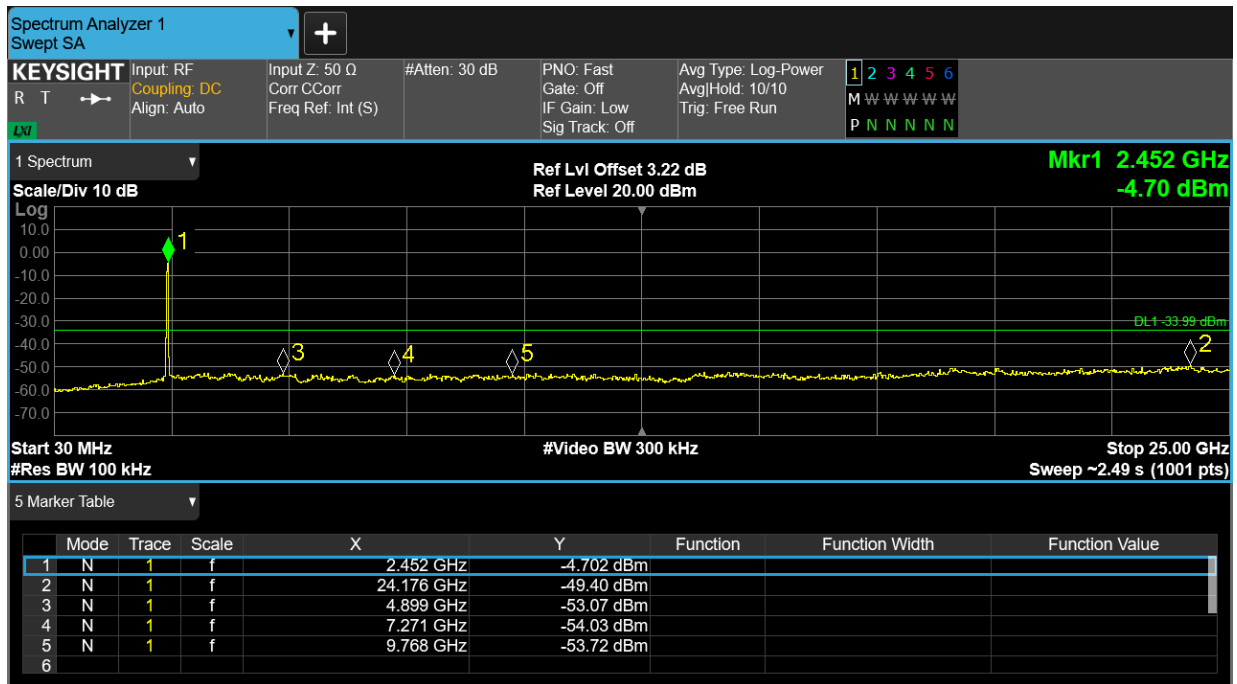
Tx. Spurious NVNT n40 2452MHz Ant1 Ref
