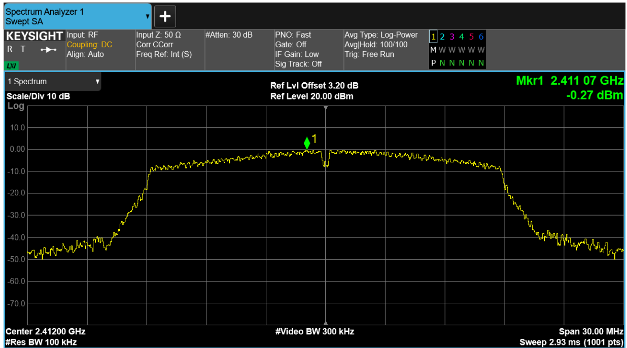
Band Edge NVNT n20 2412MHz Ant1 Emission
