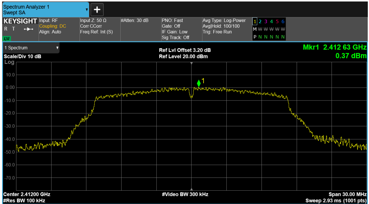
Band Edge NVNT g 2412MHz Ant1 Emission
