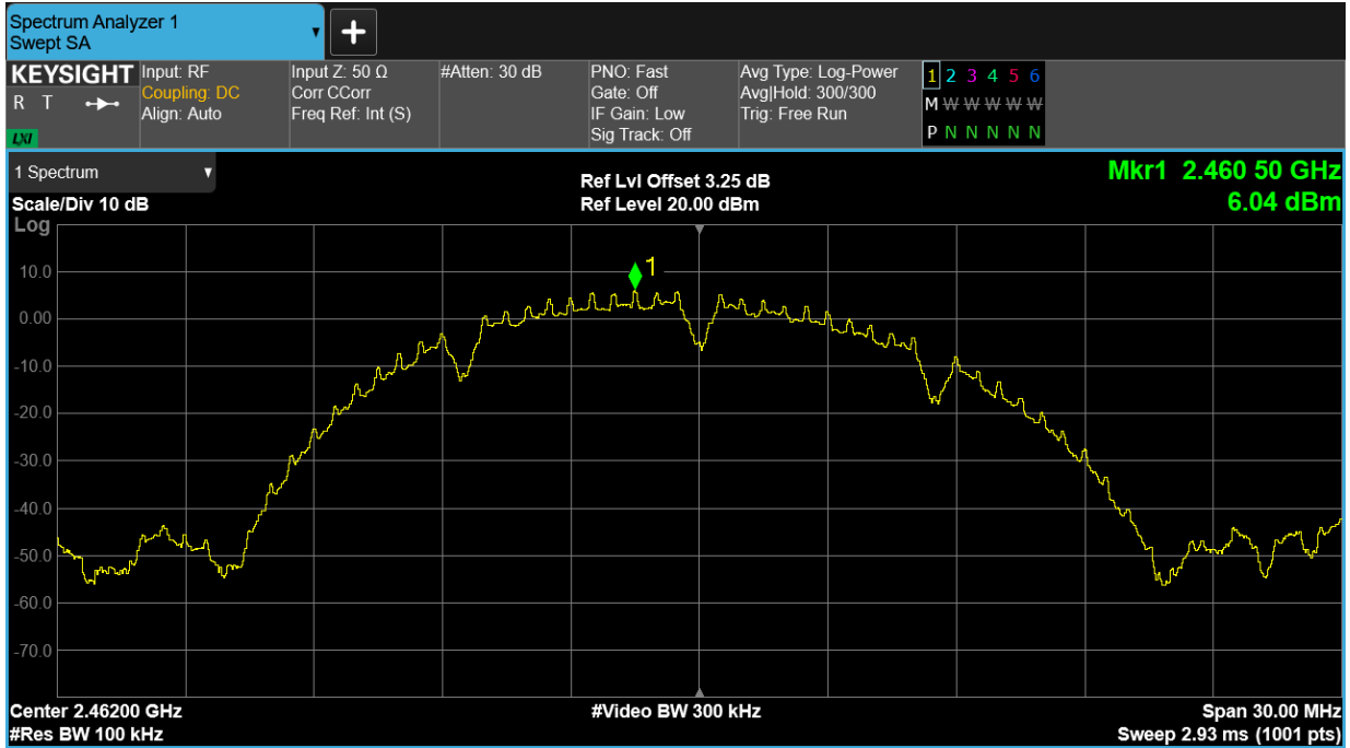
Band Edge NVNT b 2462MHz Ant1 Emission
