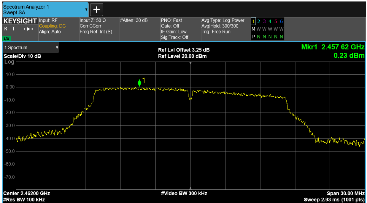
Band Edge NVNT g 2462MHz Ant1 Emission
