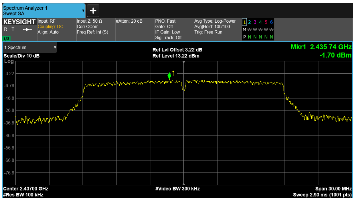
Tx. Spurious NVNT n20 2437MHz Ant1 Emission
