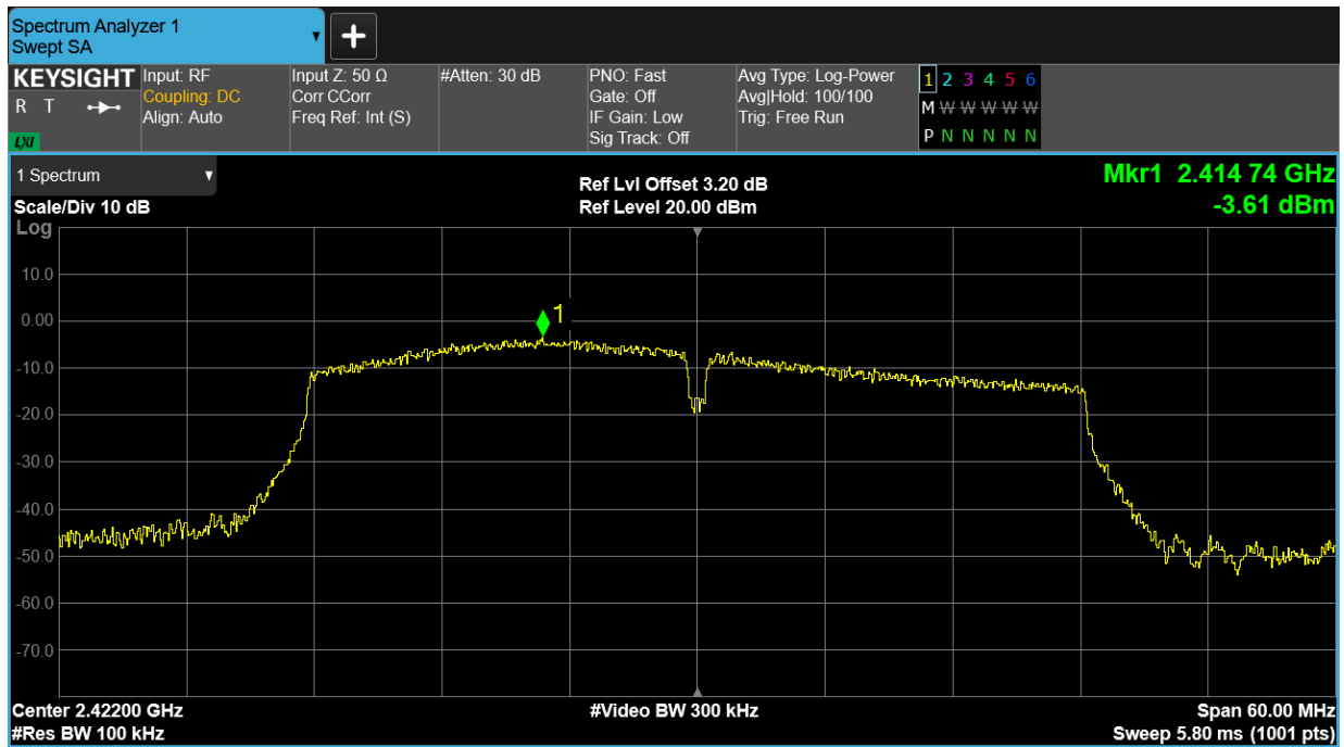
Band Edge NVNT n40 2422MHz Ant1 Emission
