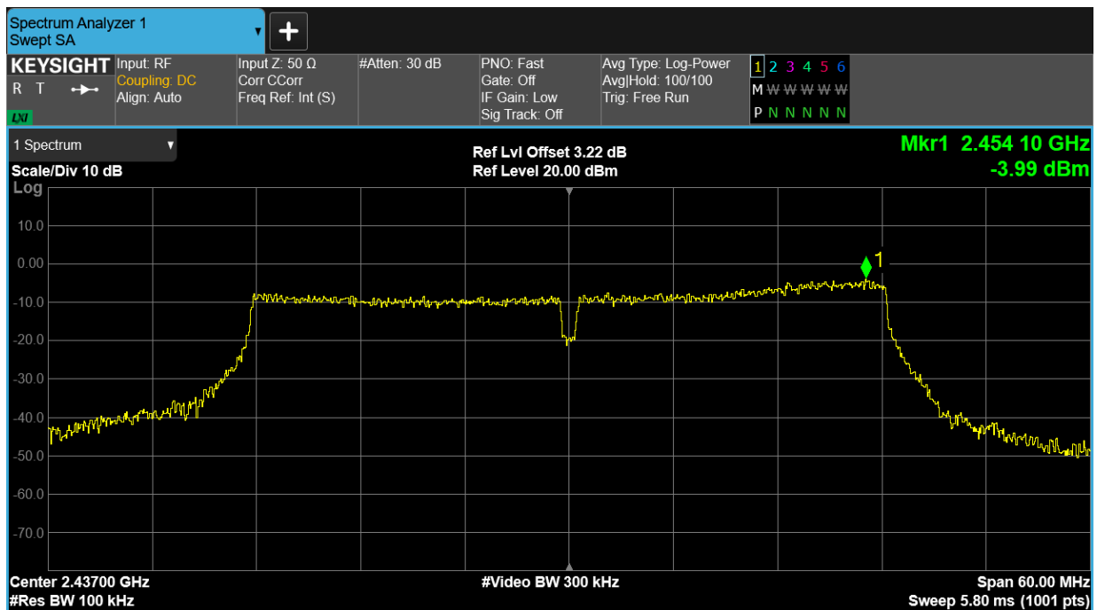
Tx. Spurious NVNT n40 2437MHz Ant1 Emission
