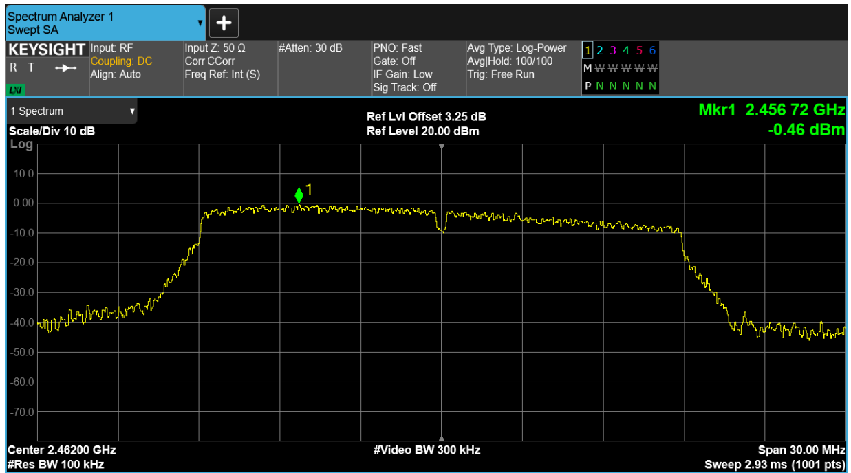
Band Edge NVNT n20 2462MHz Ant1 Emission
