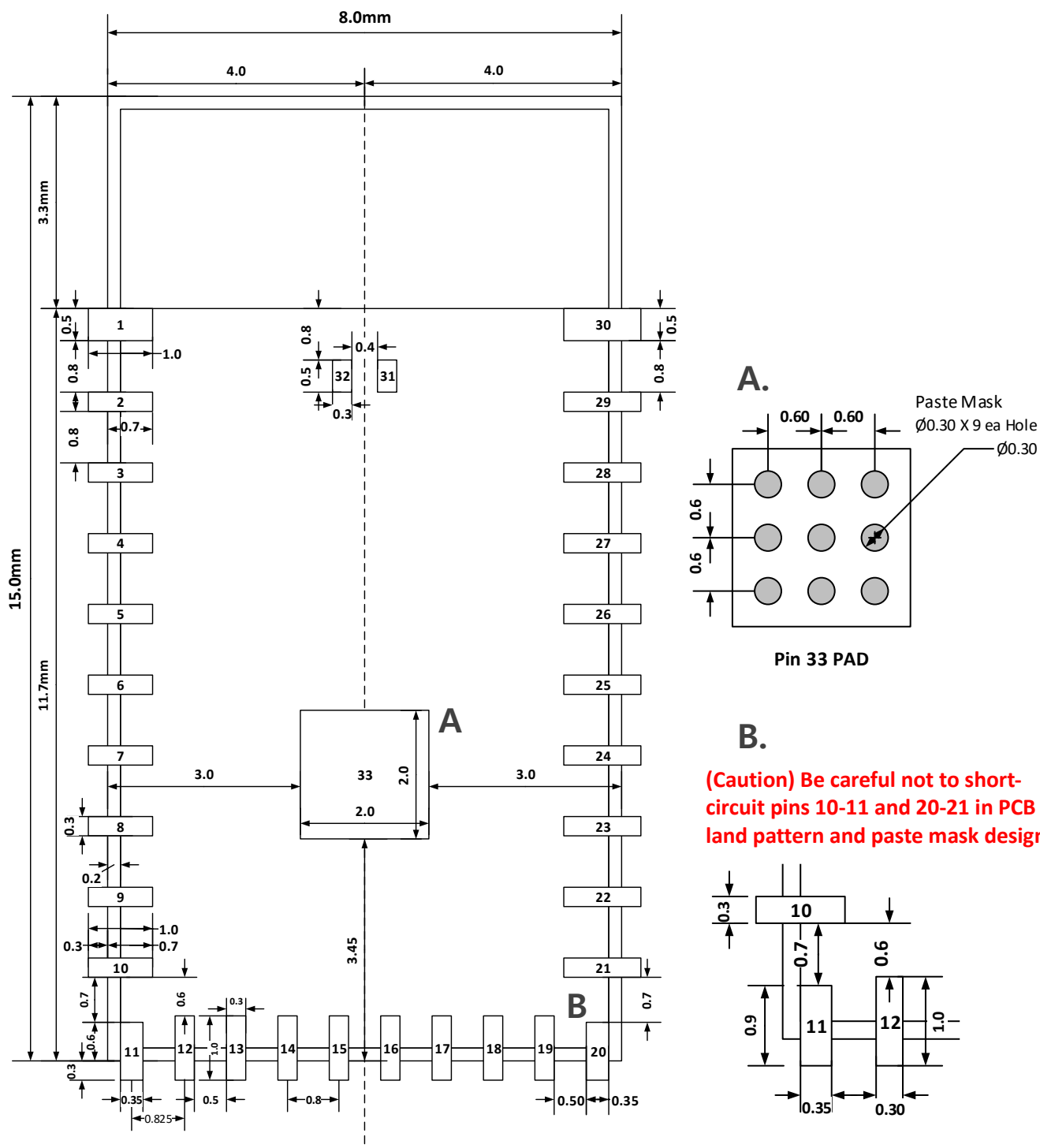
Land Pattern (TOP VIEW)
