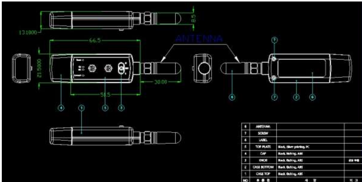
Figure F-1 Antenna Location
