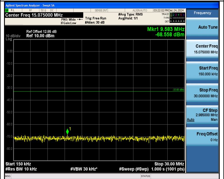
Band4_5MHz_16QAM_20375_25RB#0_0.15~30_0.15~30
