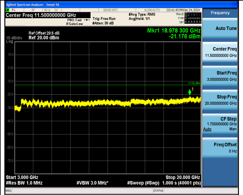
Band4_10MHz_QPSK_20000_1RB#49_3000~20000_3000~20000
