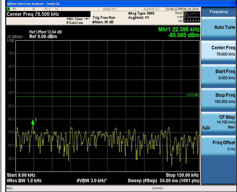
Band4_10MHz_16QAM_20175_1RB#49_0.009~0.15_0.009~0.15
