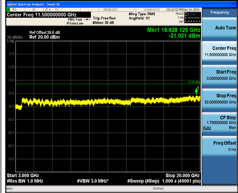
Band4_5MHz_16QAM_20375_25RB#0_3000~20000_3000~20000
