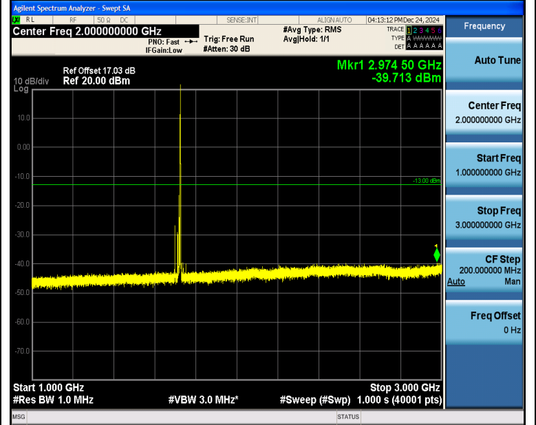
Band4_15MHz_QPSK_20025_1RB#74_1000~3000_1000~3000
