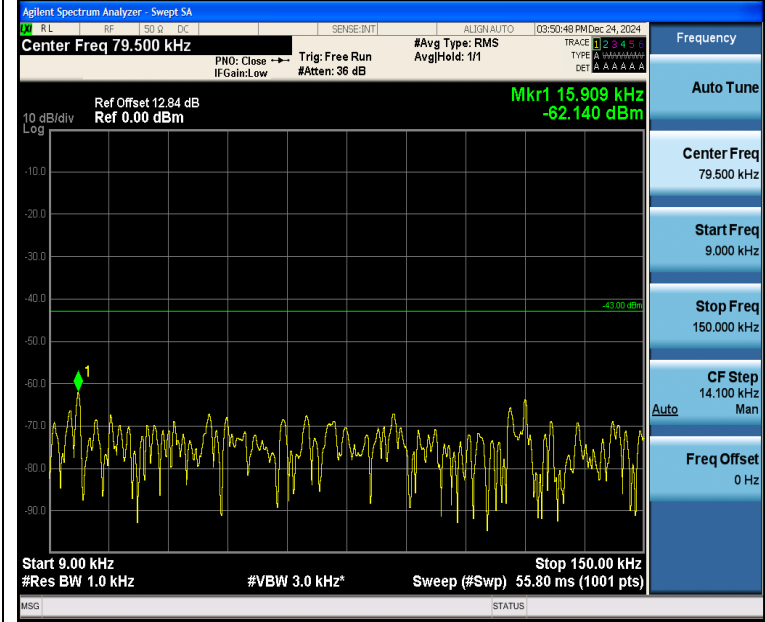
Band4_10MHz_16QAM_20350_1RB#49_0.009~0.15_0.009~0.15
