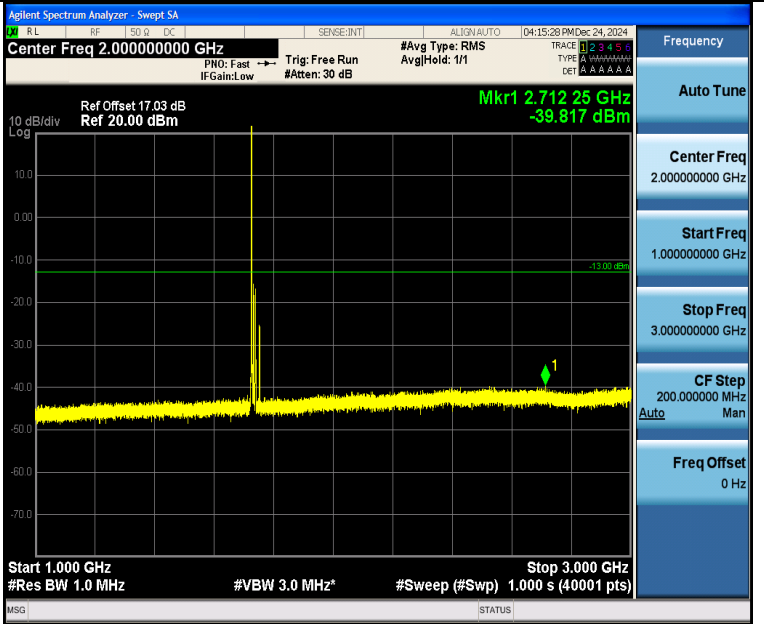
Band4_15MHz_QPSK_20175_1RB#0_1000~3000_1000~3000
