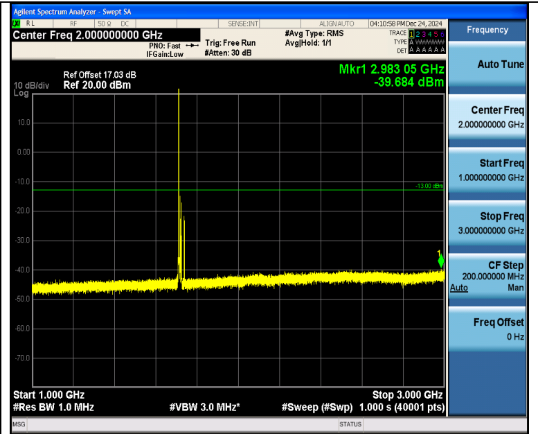
Band4_15MHz_QPSK_20025_1RB#0_1000~3000_1000~3000
