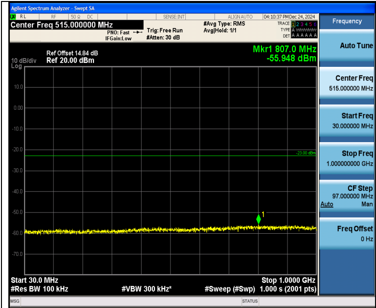
Band4_15MHz_QPSK_20025_1RB#0_30~1000_30~1000
