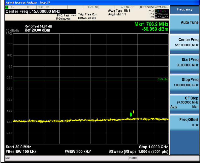
Band4_10MHz_16QAM_20000_1RB#0_30~1000_30~1000
