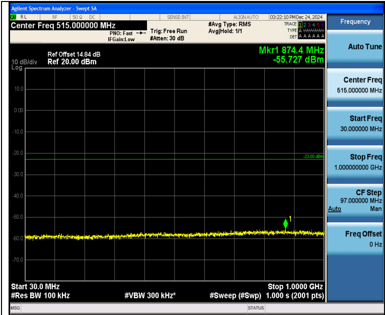
Band4_5MHz_16QAM_20375_25RB#0_30~1000_30~1000
