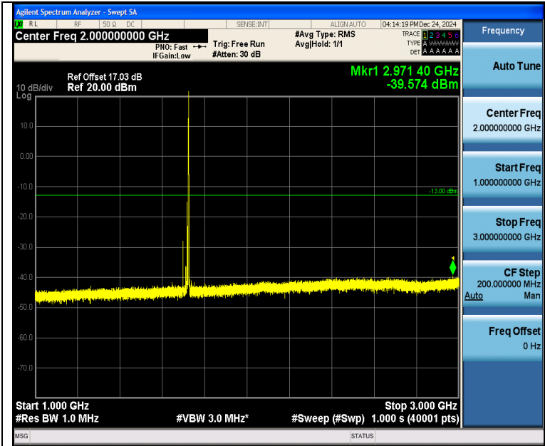
Band4_15MHz_16QAM_20025_1RB#74_1000~3000_1000~3000
