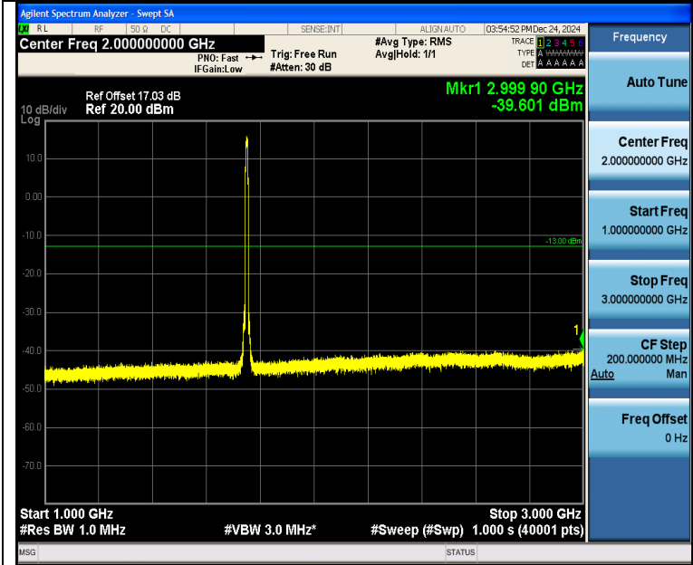
Band4_10MHz_QPSK_20350_50RB#0_1000~3000_1000~3000
