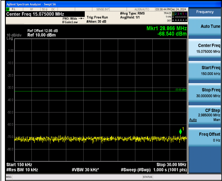
Band4_10MHz_QPSK_20000_1RB#0_0.15~30_0.15~30
