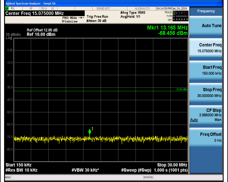
Band4_15MHz_QPSK_20175_1RB#0_0.15~30_0.15~30
