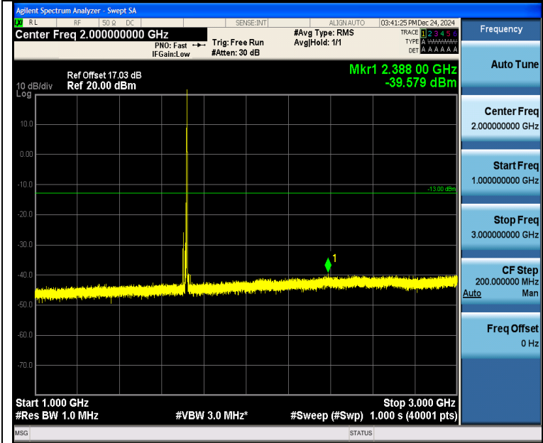
Band4_10MHz_QPSK_20000_1RB#49_1000~3000_1000~3000
