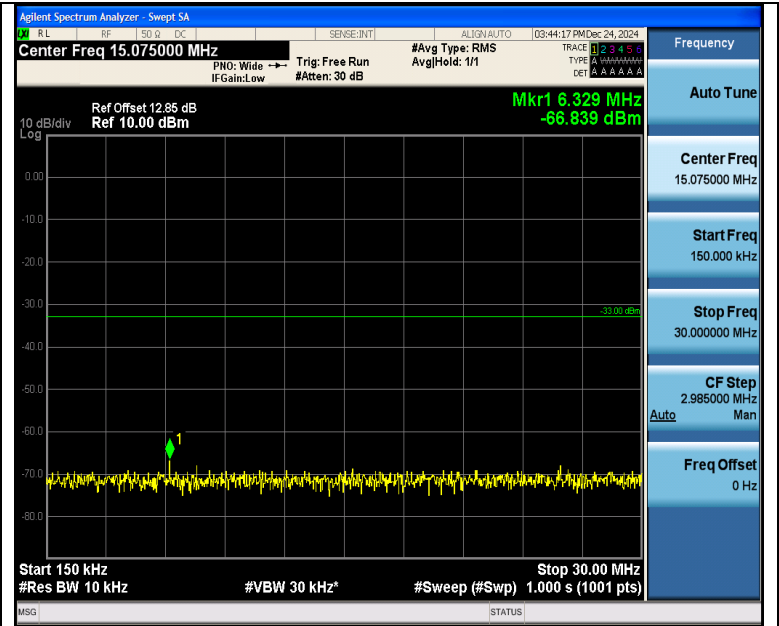
Band4_10MHz_16QAM_20175_1RB#0_0.15~30_0.15~30
