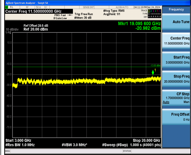
Band4_15MHz_QPSK_20025_1RB#0_3000~20000_3000~20000
