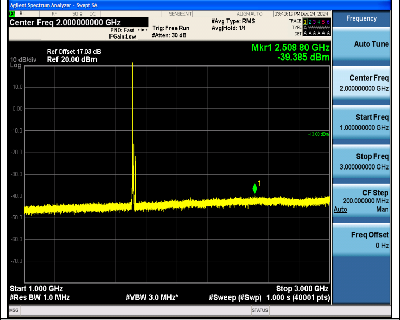
Band4_10MHz_16QAM_20000_1RB#0_1000~3000_1000~3000
