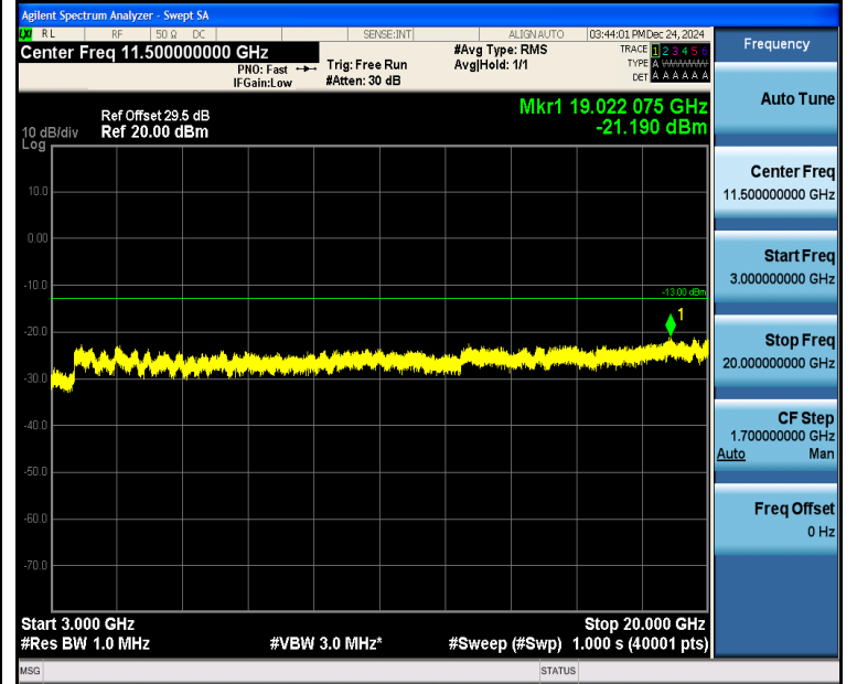
Band4_10MHz_QPSK_20175_1RB#0_3000~20000_3000~20000
