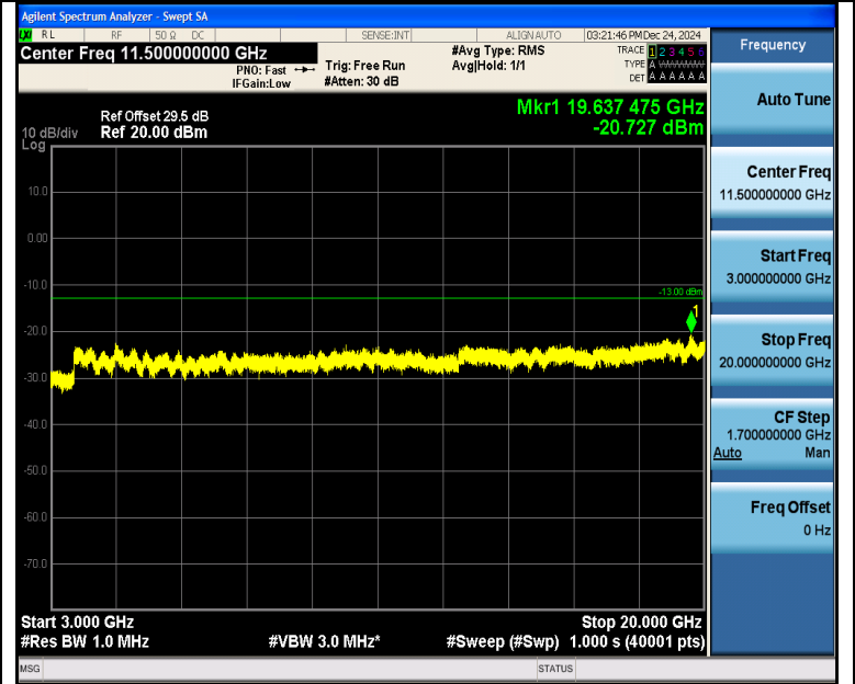
Band4_5MHz_QPSK_20375_25RB#0_3000~20000_3000~20000
