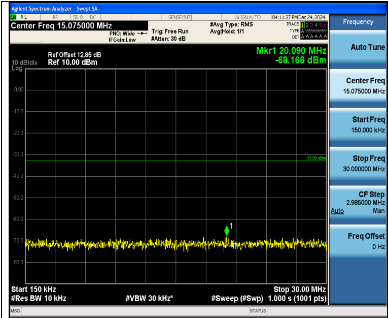
Band4_15MHz_16QAM_20025_1RB#0_0.15~30_0.15~30
