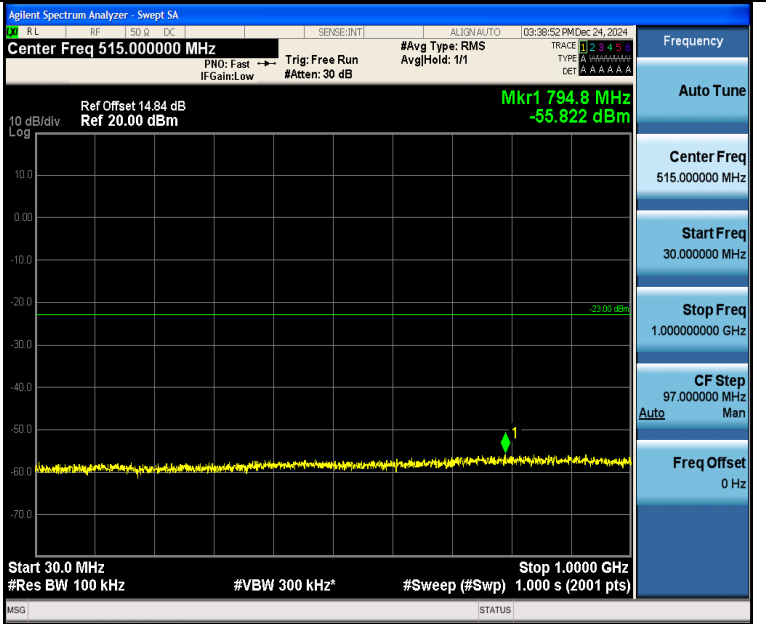
Band4_10MHz_QPSK_20000_1RB#0_30~1000_30~1000
