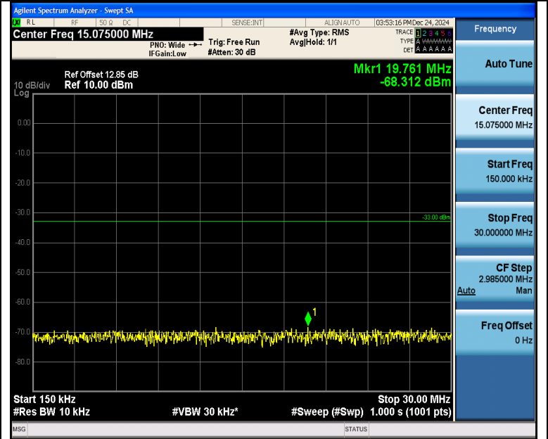
Band4_10MHz_QPSK_20175_50RB#0_0.15~30_0.15~30
