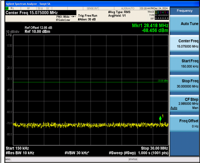
Band4_5MHz_QPSK_20375_1RB#24_0.15~30_0.15~30
