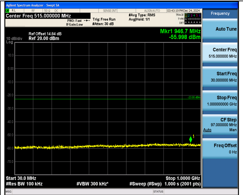
Band4_10MHz_QPSK_20175_1RB#0_30~1000_30~1000
