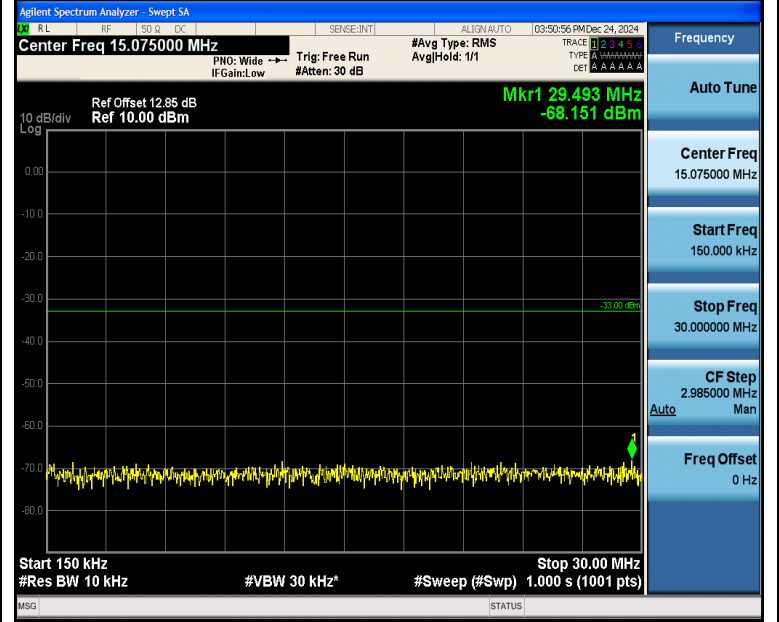
Band4_10MHz_16QAM_20350_1RB#49_0.15~30_0.15~30
