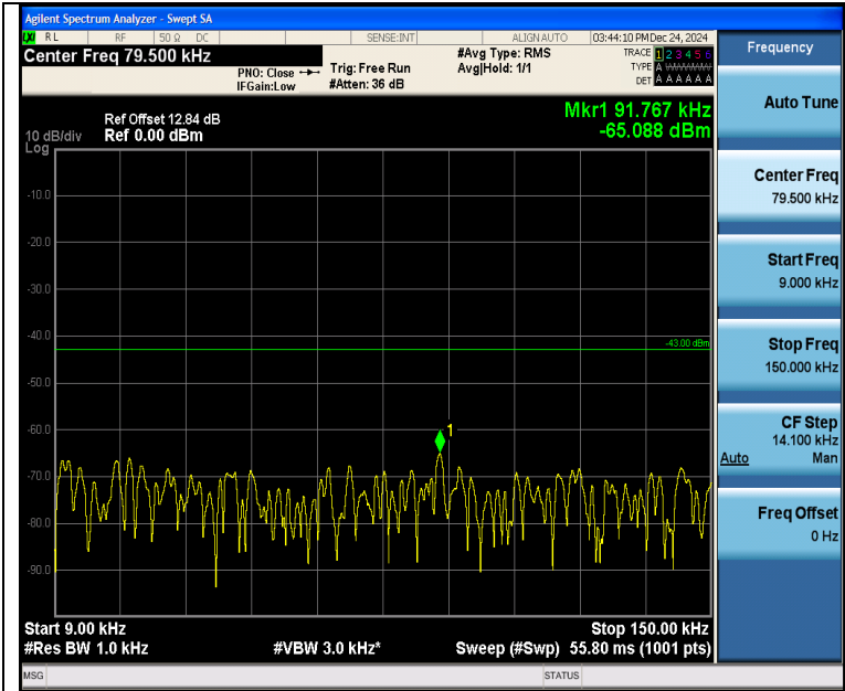
Band4_10MHz_16QAM_20175_1RB#0_0.009~0.15_0.009~0.15
