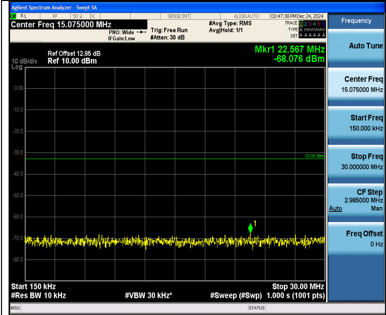
Band4_10MHz_QPSK_20350_1RB#0_0.15~30_0.15~30
