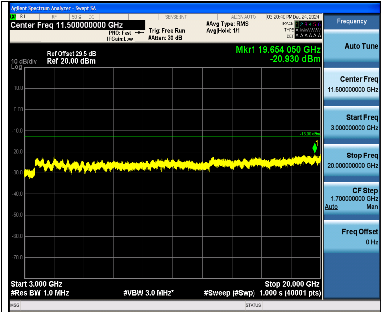
Band4_5MHz_16QAM_20375_1RB#24_3000~20000_3000~20000
