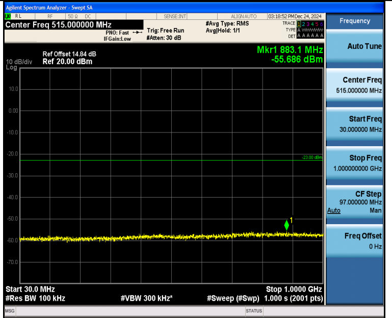
Band4_5MHz_QPSK_20375_1RB#24_30~1000_30~1000
