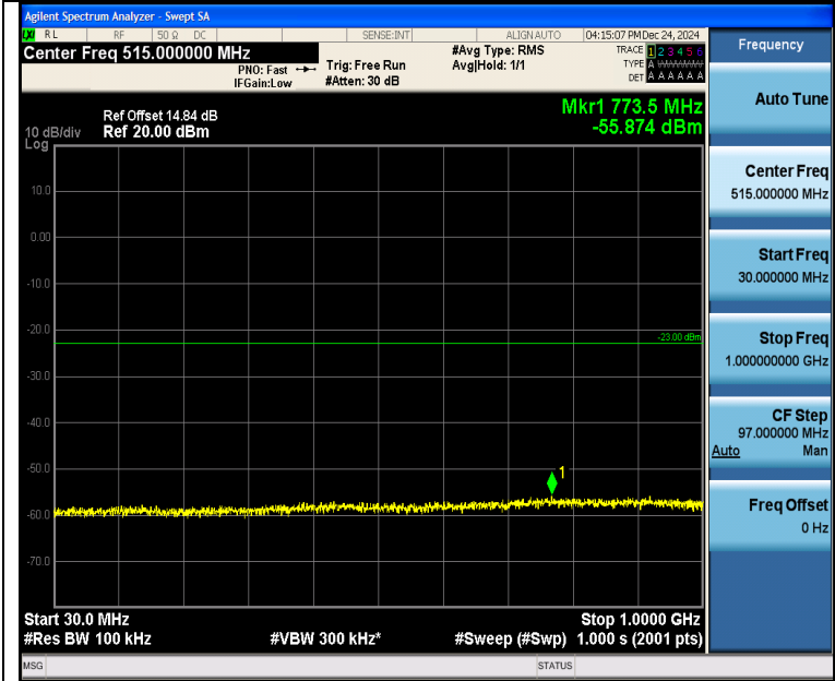
Band4_15MHz_QPSK_20175_1RB#0_30~1000_30~1000
