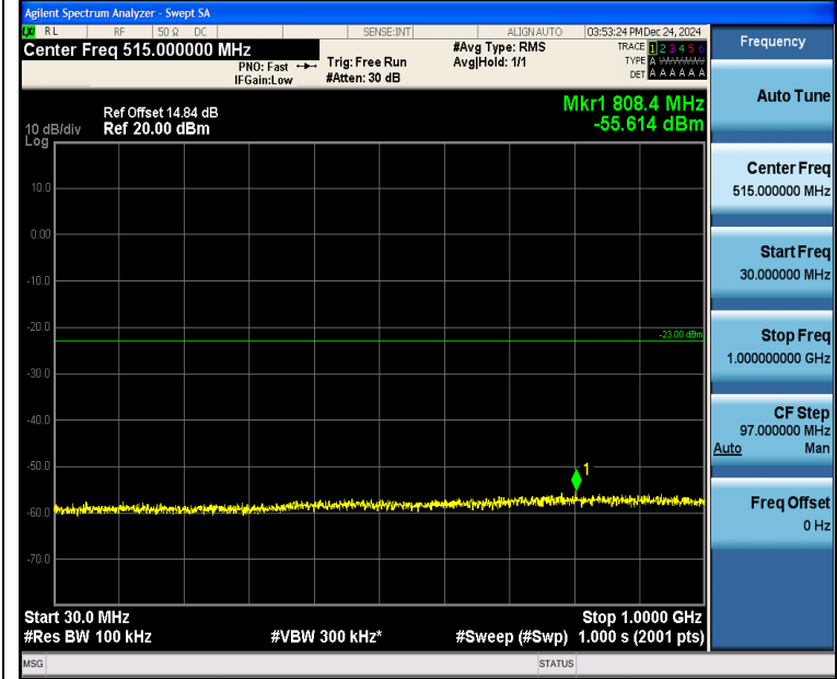
Band4_10MHz_QPSK_20175_50RB#0_30~1000_30~1000
