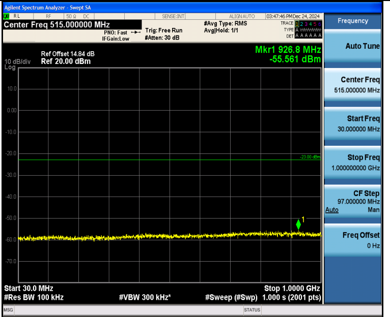
Band4_10MHz_QPSK_20350_1RB#0_30~1000_30~1000
