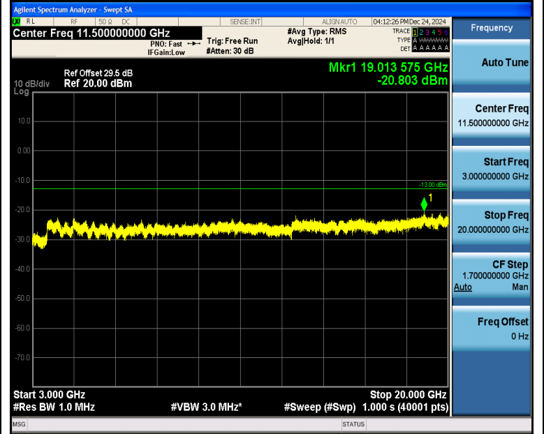
Band4_15MHz_16QAM_20025_1RB#0_3000~20000_3000~20000
