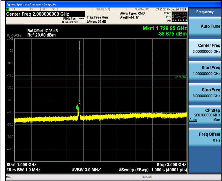
Band4_5MHz_QPSK_20375_25RB#0_1000~3000_1000~3000
