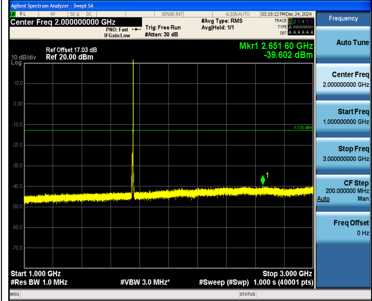
Band4_5MHz_QPSK_20375_1RB#24_1000~3000_1000~3000
