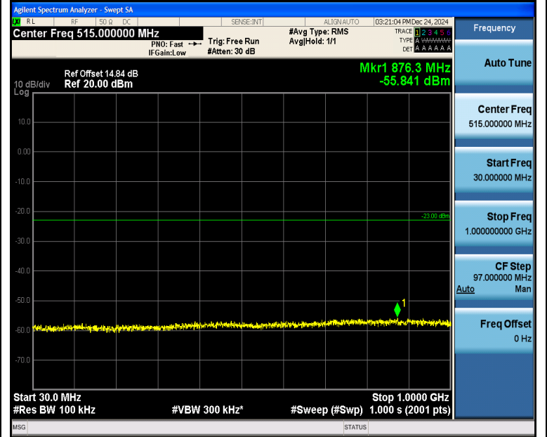
Band4_5MHz_QPSK_20375_25RB#0_30~1000_30~1000
