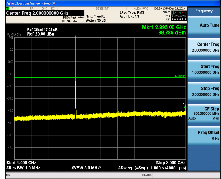
Band4_10MHz_QPSK_20000_1RB#0_1000~3000_1000~3000
