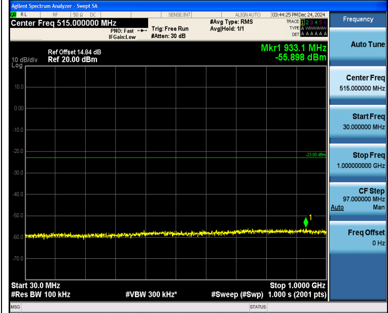
Band4_10MHz_16QAM_20175_1RB#0_30~1000_30~1000
