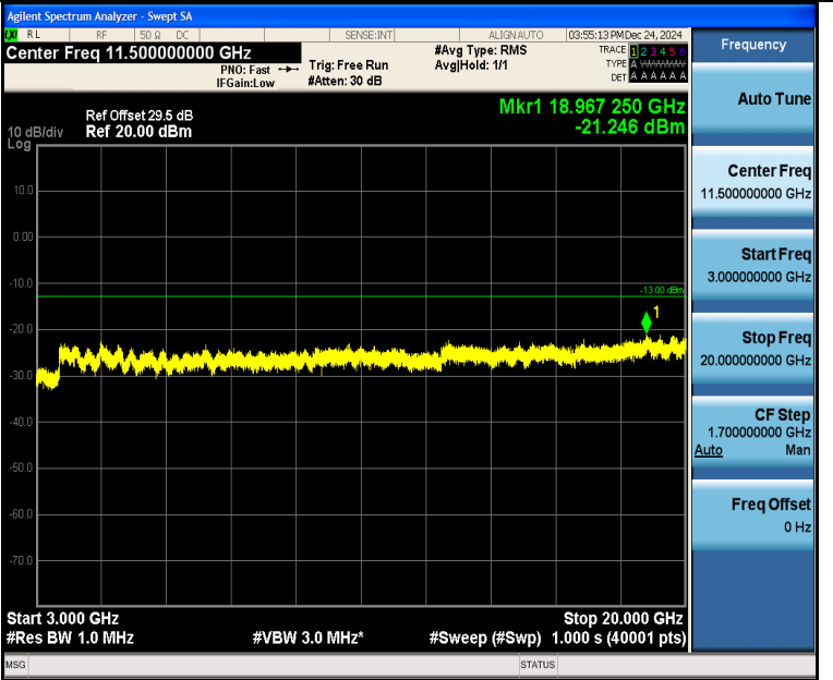
Band4_10MHz_QPSK_20350_50RB#0_3000~20000_3000~20000
