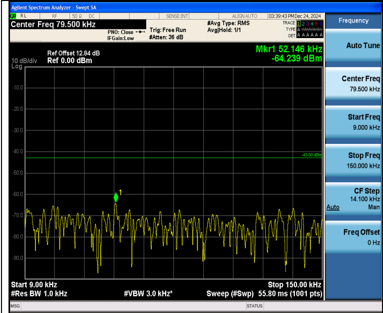
Band4_10MHz_16QAM_20000_1RB#0_0.009~0.15_0.009~0.15
