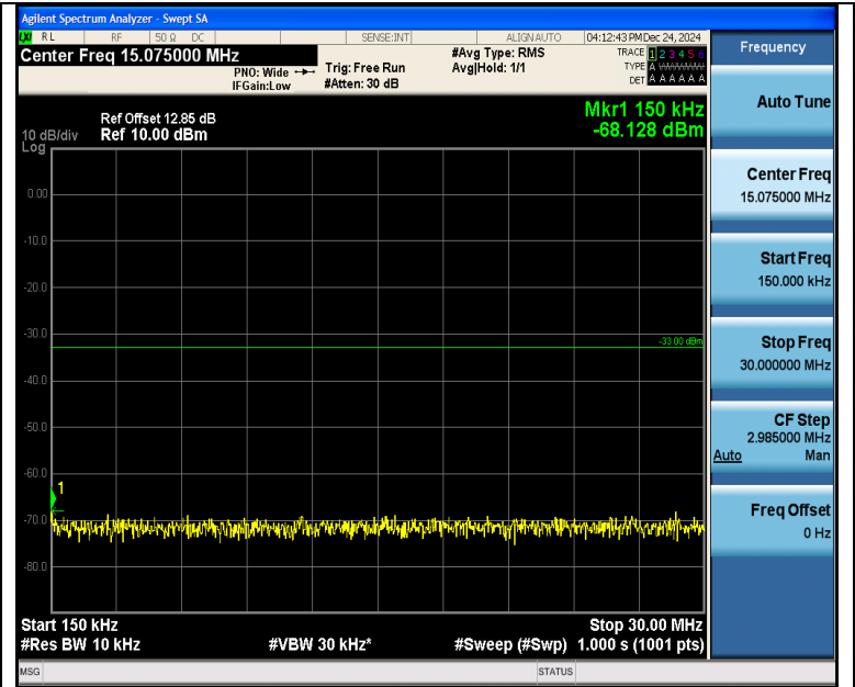
Band4_15MHz_QPSK_20025_1RB#74_0.15~30_0.15~30
