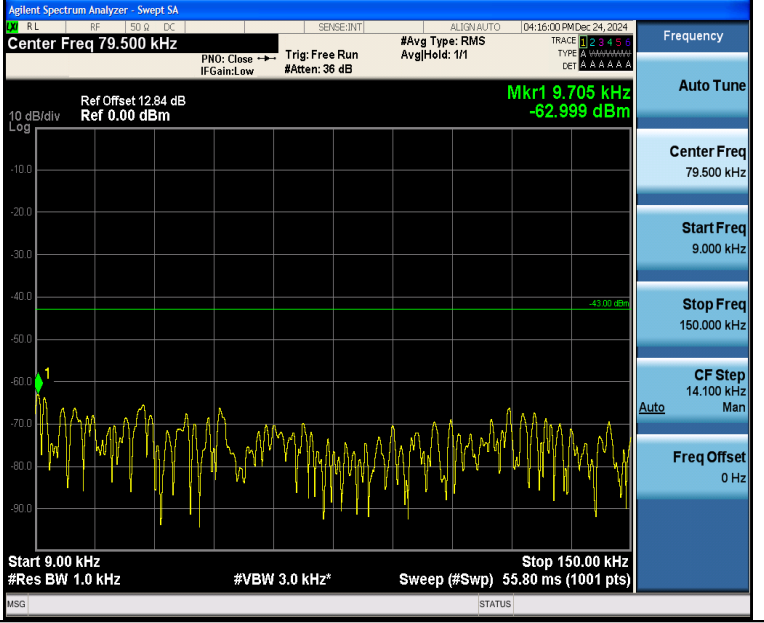
Band4_15MHz_16QAM_20175_1RB#0_0.009~0.15_0.009~0.15
