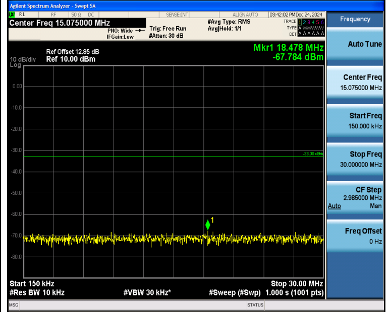
Band4_10MHz_16QAM_20000_1RB#49_0.15~30_0.15~30
