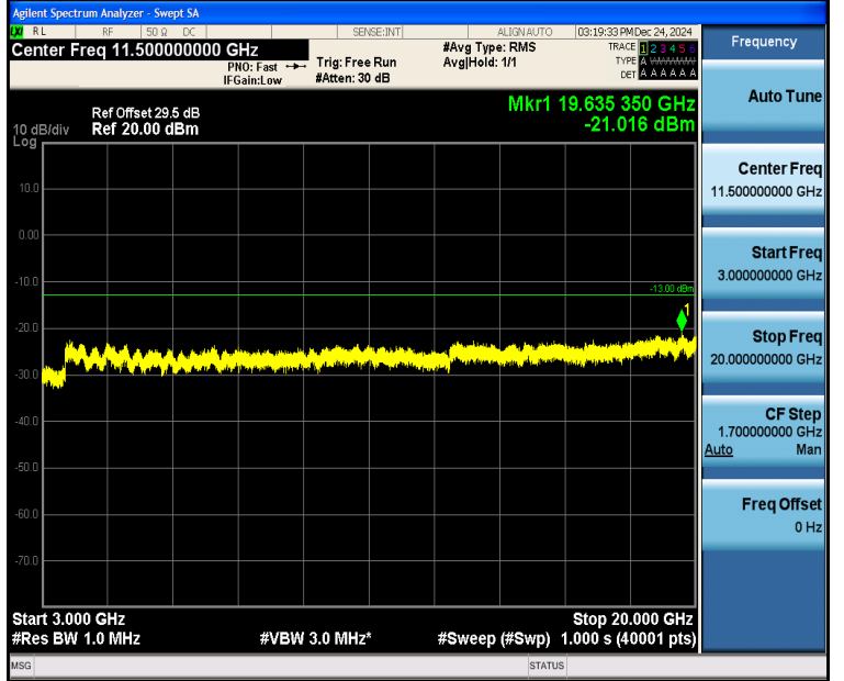
Band4_5MHz_QPSK_20375_1RB#24_3000~20000_3000~20000
