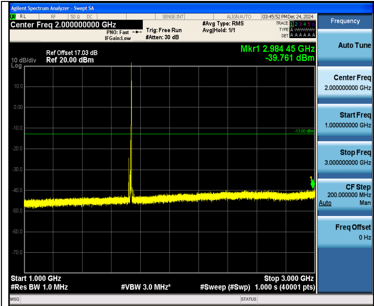
Band4_10MHz_QPSK_20175_1RB#49_1000~3000_1000~3000
