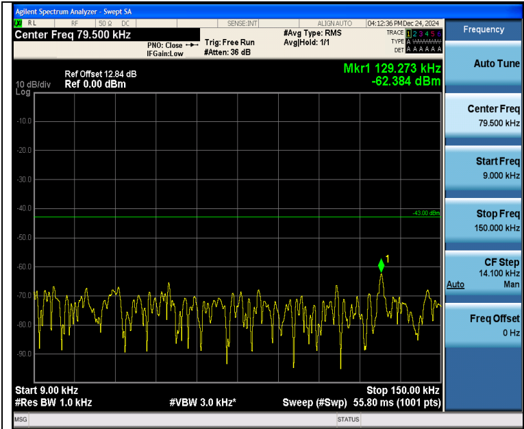
Band4_15MHz_QPSK_20025_1RB#74_0.009~0.15_0.009~0.15
