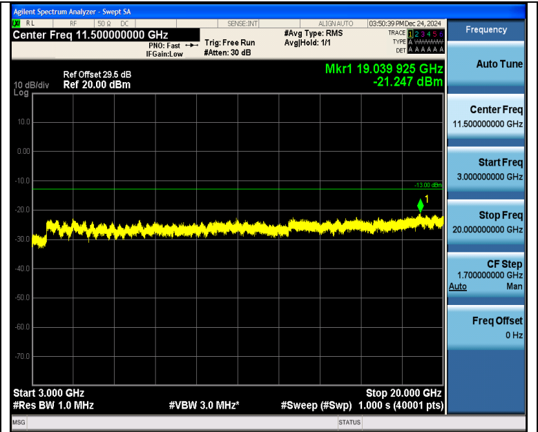
Band4_10MHz_QPSK_20350_1RB#49_3000~20000_3000~20000
