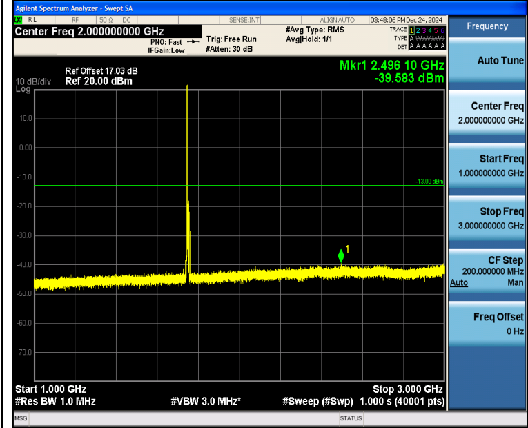
Band4_10MHz_QPSK_20350_1RB#0_1000~3000_1000~3000
