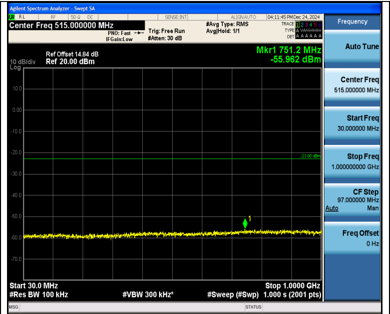
Band4_15MHz_16QAM_20025_1RB#0_30~1000_30~1000
