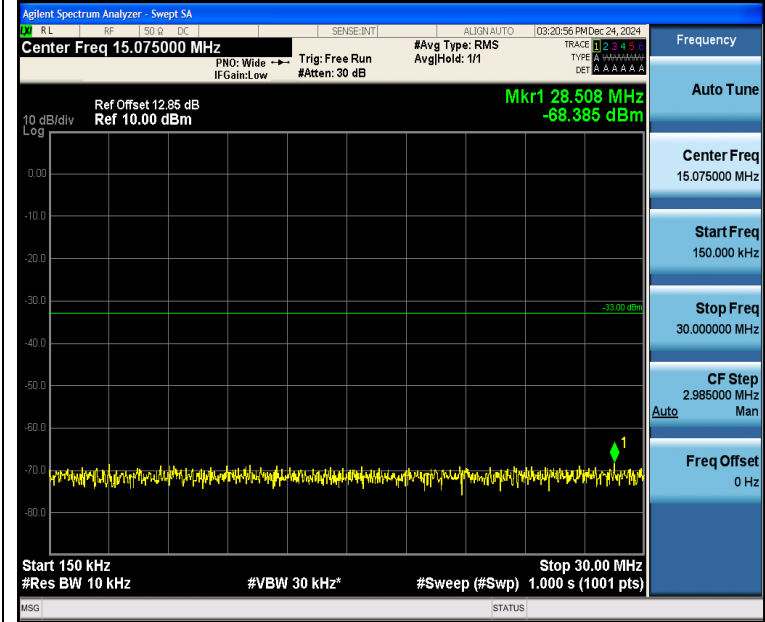
Band4_5MHz_QPSK_20375_25RB#0_0.15~30_0.15~30
