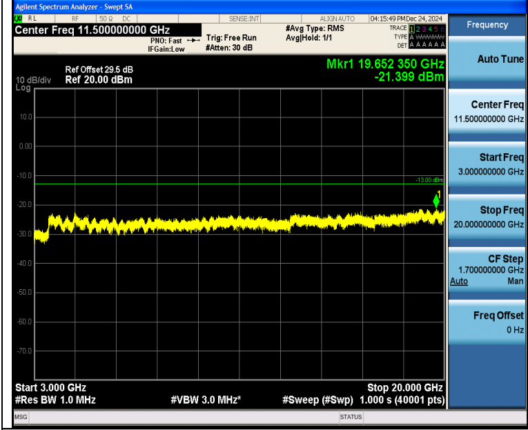
Band4_15MHz_QPSK_20175_1RB#0_3000~20000_3000~20000
