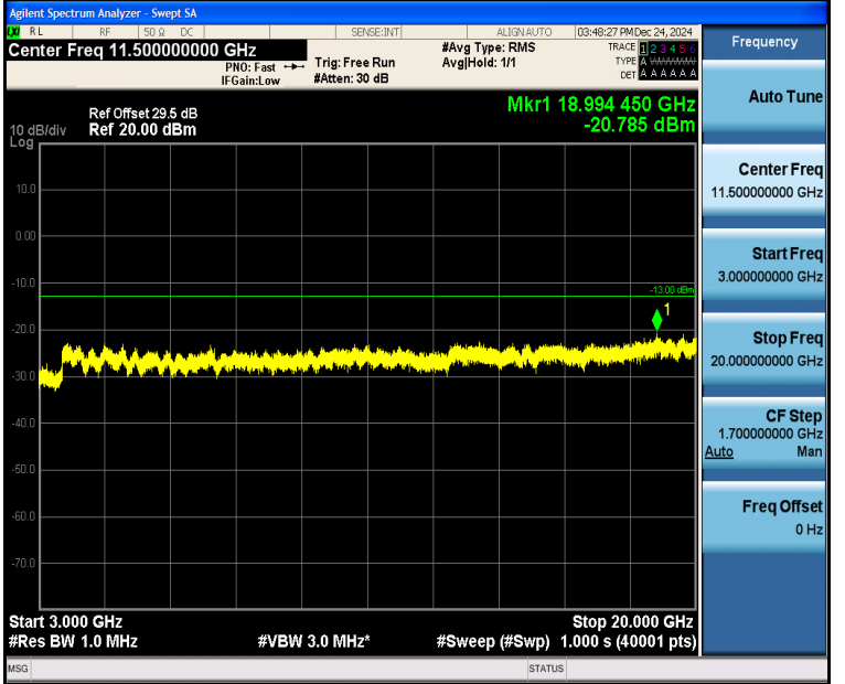
Band4_10MHz_QPSK_20350_1RB#0_3000~20000_3000~20000
