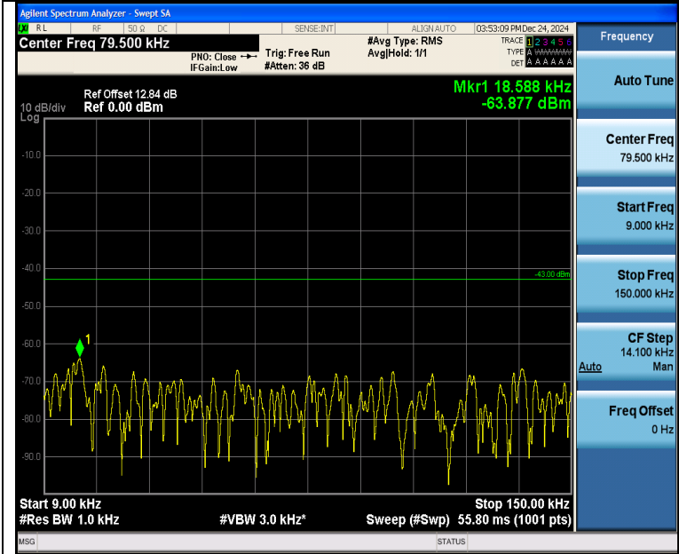
Band4_10MHz_QPSK_20175_50RB#0_0.009~0.15_0.009~0.15
