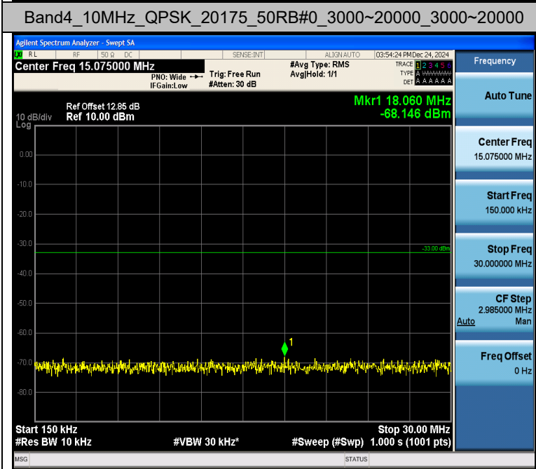
Band4_10MHz_QPSK_20175_50RB#0_3000~20000_3000~20000
