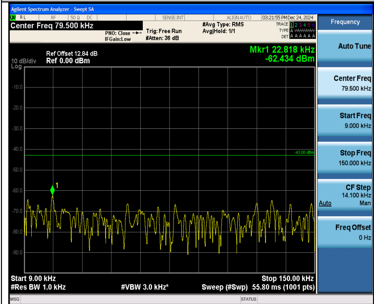
Band4_5MHz_16QAM_20375_25RB#0_0.009~0.15_0.009~0.15
