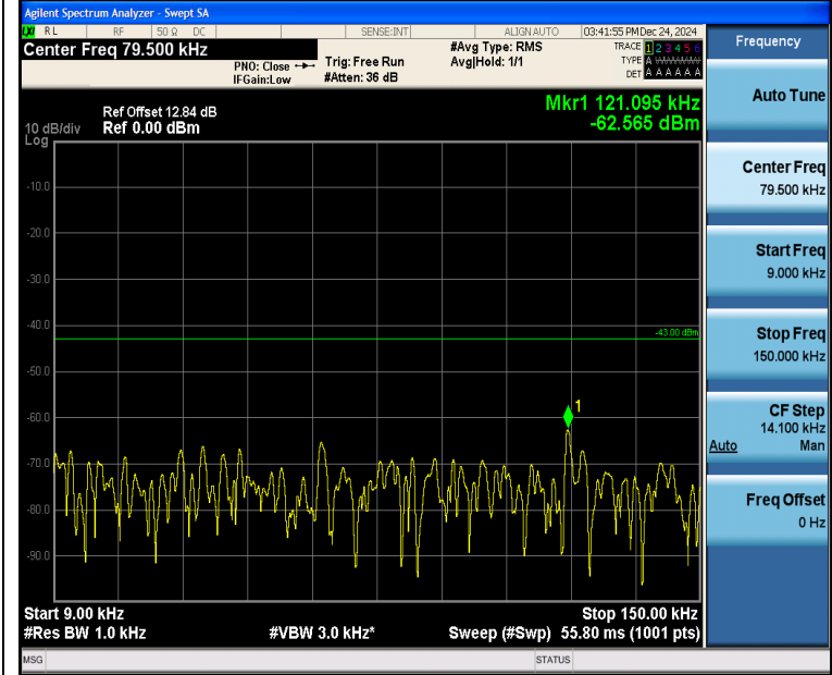
Band4_10MHz_16QAM_20000_1RB#49_0.009~0.15_0.009~0.15
