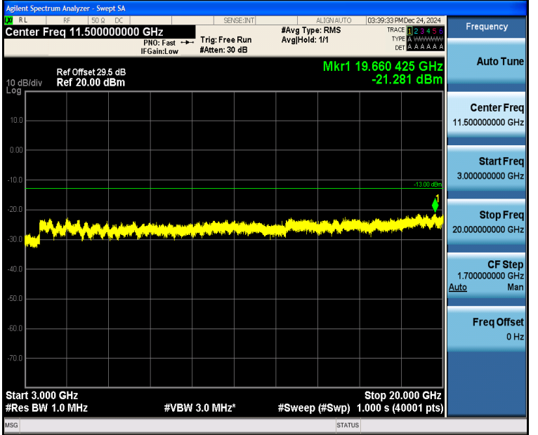
Band4_10MHz_QPSK_20000_1RB#0_3000~20000_3000~20000
