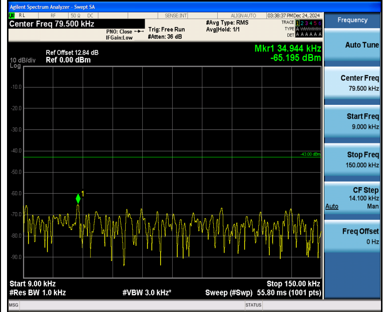
Band4_10MHz_QPSK_20000_1RB#0_0.009~0.15_0.009~0.15
