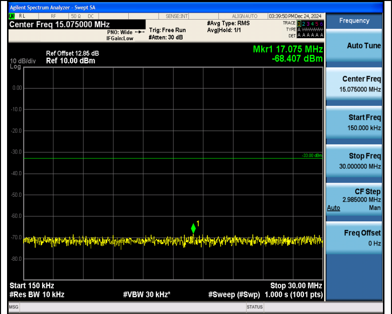
Band4_10MHz_16QAM_20000_1RB#0_0.15~30_0.15~30
