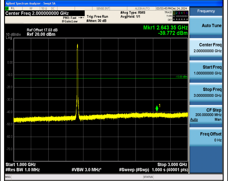
Band4_10MHz_QPSK_20175_50RB#0_1000~3000_1000~3000
