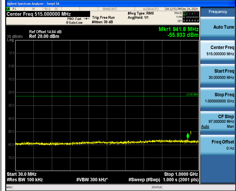
Band4_15MHz_QPSK_20025_1RB#74_30~1000_30~1000
