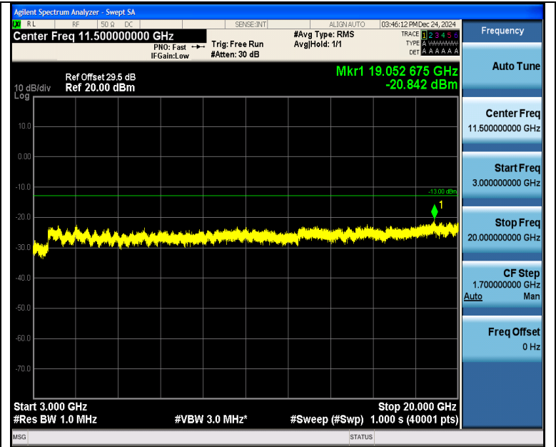
Band4_10MHz_QPSK_20175_1RB#49_3000~20000_3000~20000
