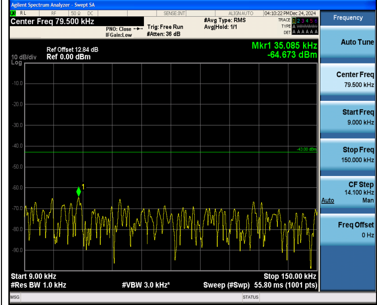
Band4_15MHz_QPSK_20025_1RB#0_0.009~0.15_0.009~0.15
