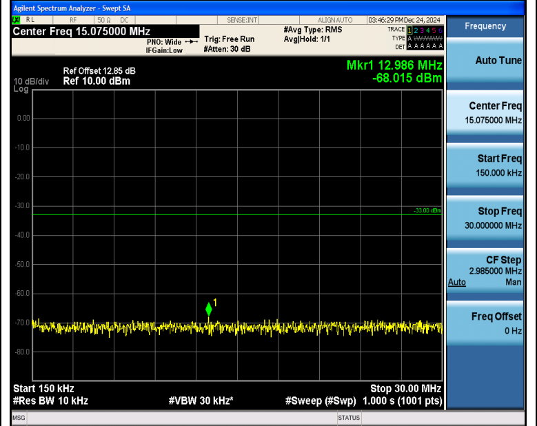
Band4_10MHz_16QAM_20175_1RB#49_0.15~30_0.15~30
