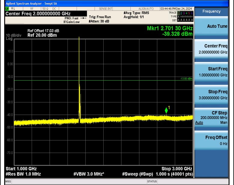
Band4_10MHz_16QAM_20175_1RB#0_1000~3000_1000~3000
