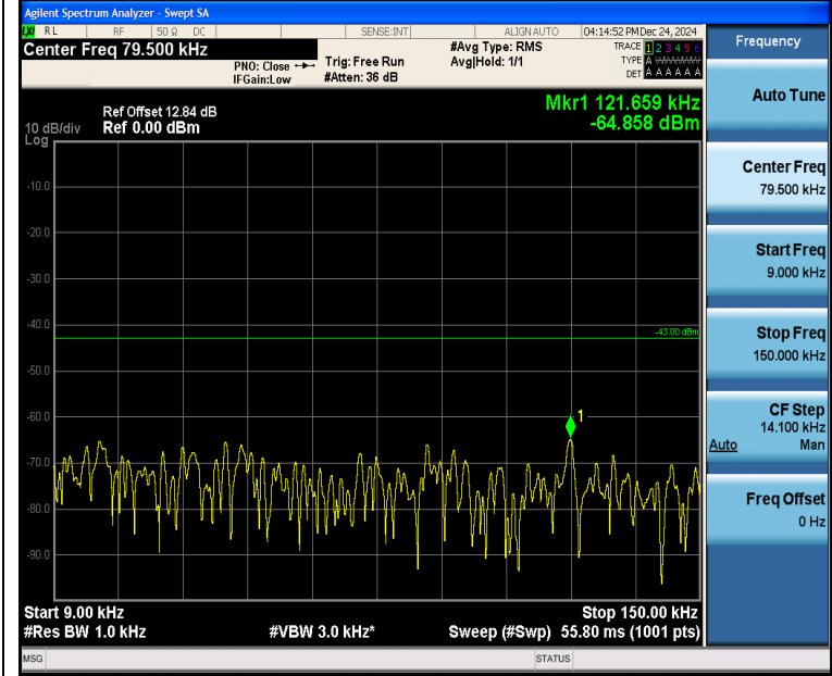
Band4_15MHz_QPSK_20175_1RB#0_0.009~0.15_0.009~0.15
