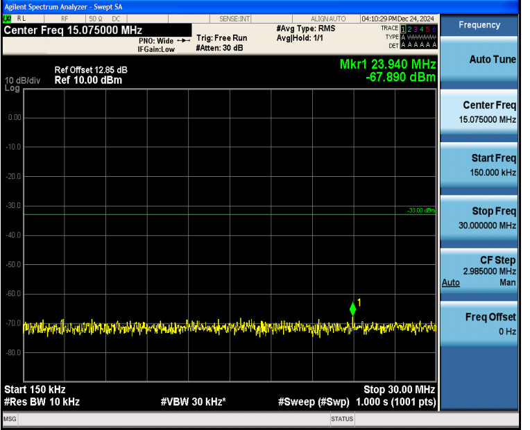
Band4_15MHz_QPSK_20025_1RB#0_0.15~30_0.15~30
