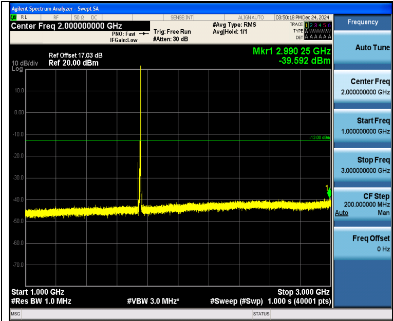
Band4_10MHz_QPSK_20350_1RB#49_1000~3000_1000~3000
