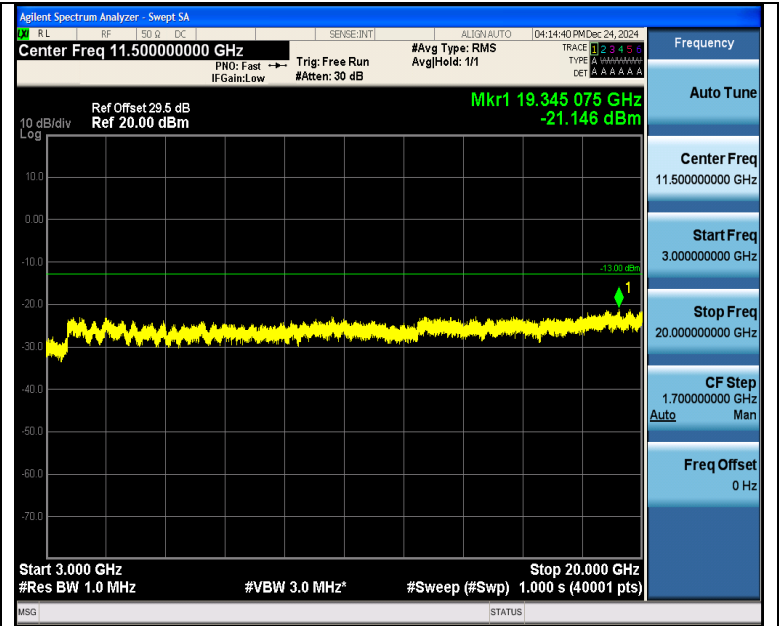
Band4_15MHz_16QAM_20025_1RB#74_3000~20000_3000~20000
