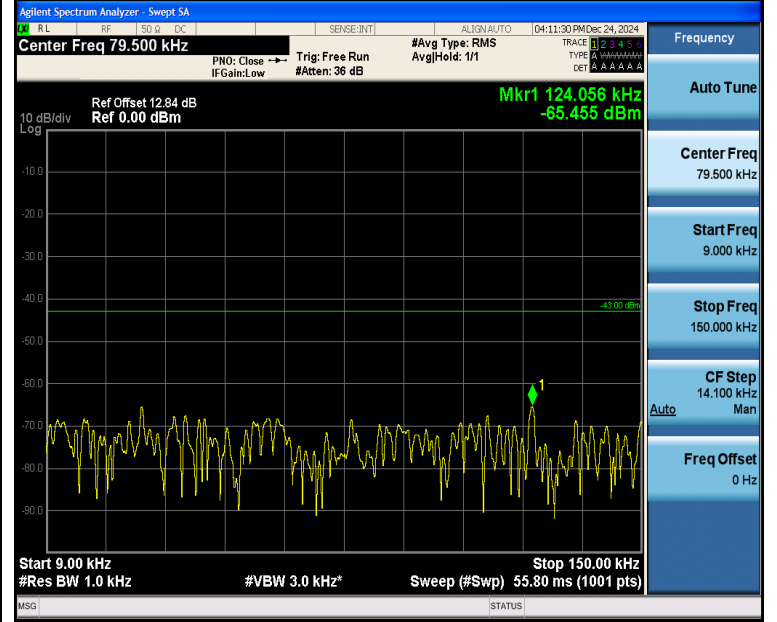
Band4_15MHz_16QAM_20025_1RB#0_0.009~0.15_0.009~0.15
