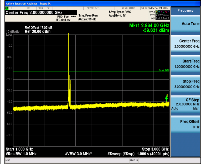
Band4_15MHz_16QAM_20025_1RB#0_1000~3000_1000~3000
