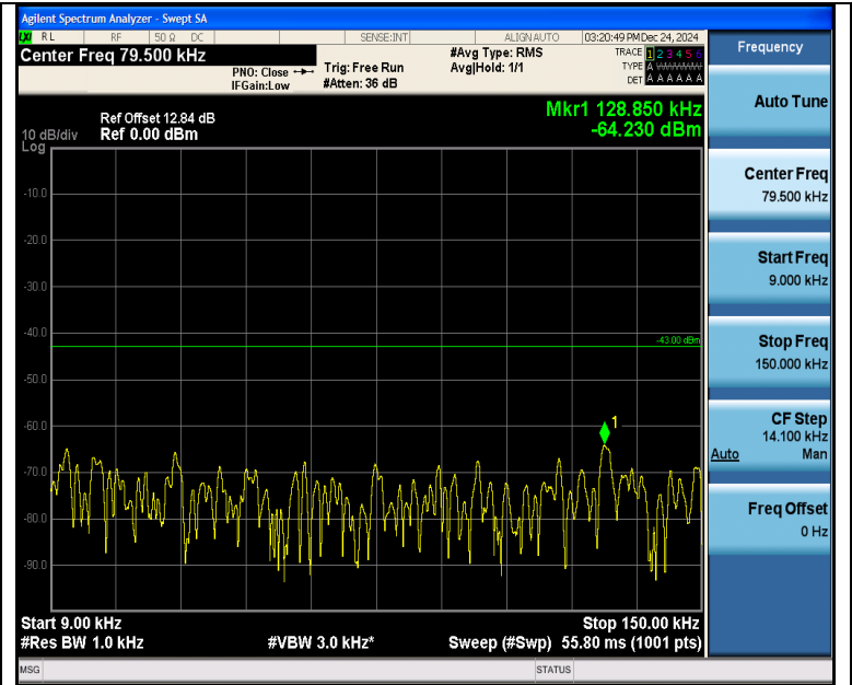
Band4_5MHz_QPSK_20375_25RB#0_0.009~0.15_0.009~0.15
