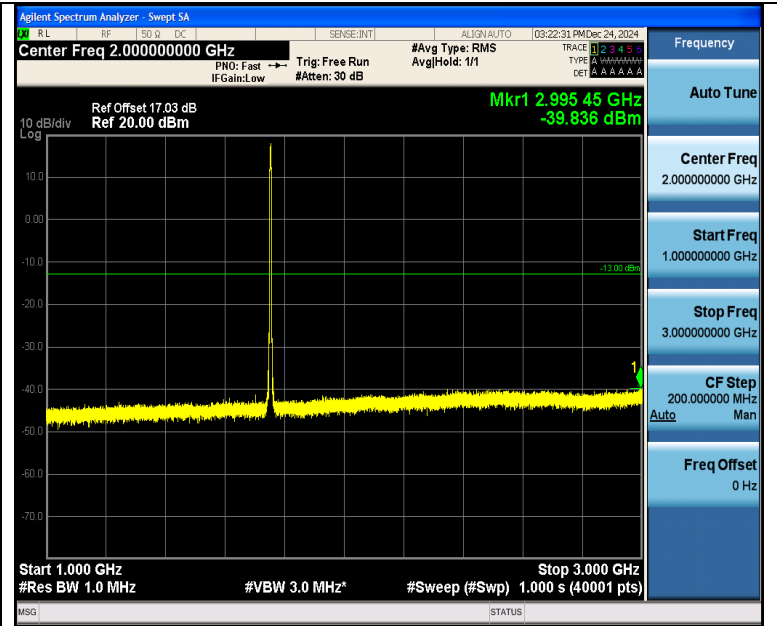
Band4_5MHz_16QAM_20375_25RB#0_1000~3000_1000~3000
