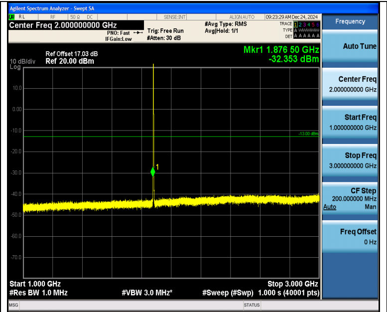
Band2_1.4MHz_QPSK_18900_6RB#0_1000~3000_1000~3000
