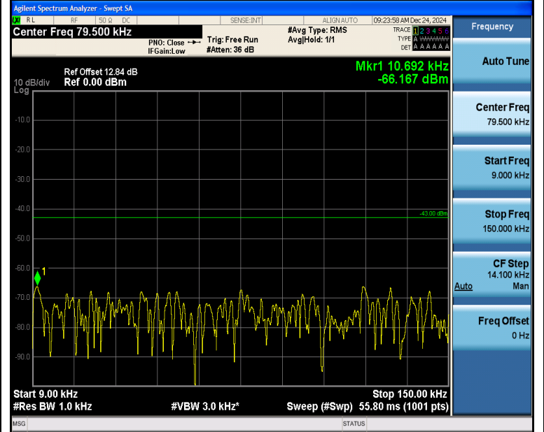
Band2_1.4MHz_16QAM_18900_6RB#0_0.009~0.15_0.009~0.15
