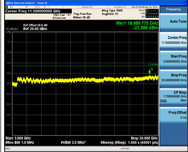
Band2_1.4MHz_QPSK_18607_1RB#5_3000~20000_3000~20000
