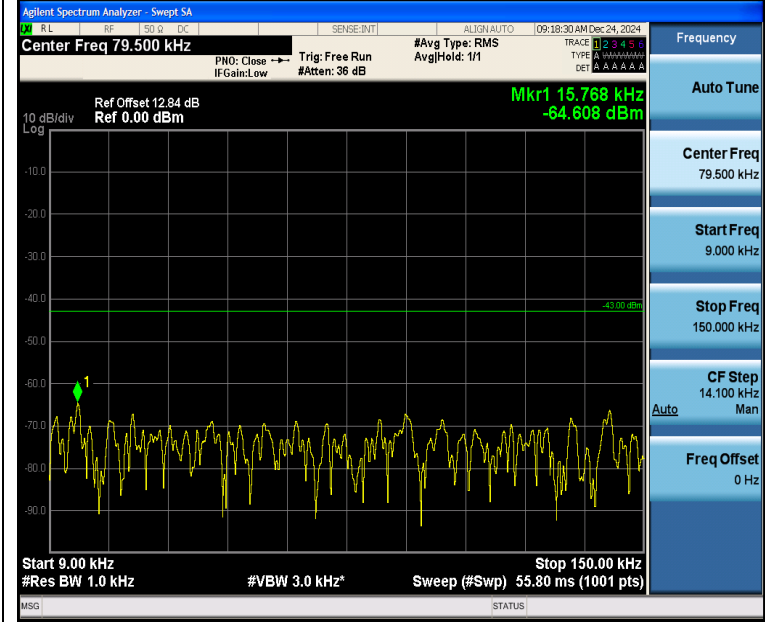
Band2_1.4MHz_QPSK_18900_1RB#0_0.009~0.15_0.009~0.15
