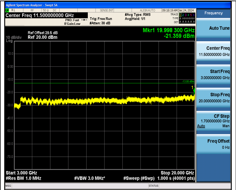
Band2_1.4MHz_16QAM_18607_6RB#0_3000~20000_3000~20000
