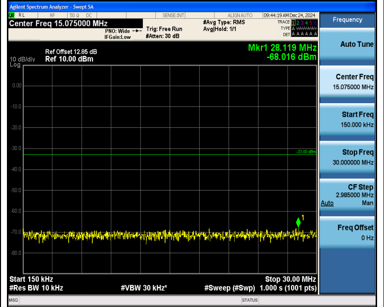
Band2_3MHz_QPSK_18900_1RB#14_0.15~30_0.15~30
