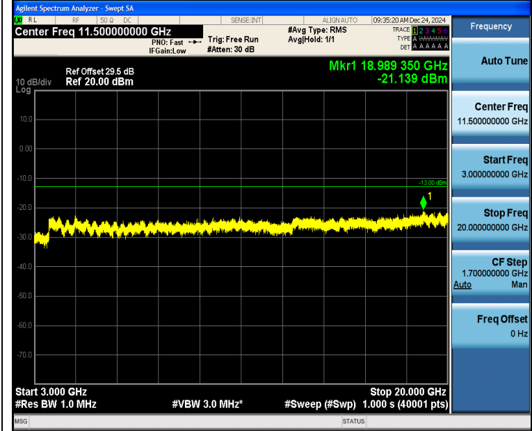
Band2_3MHz_QPSK_18615_1RB#0_3000~20000_3000~20000
