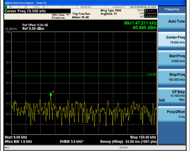
Band2_1.4MHz_16QAM_18607_1RB#5_0.009~0.15_0.009~0.15
