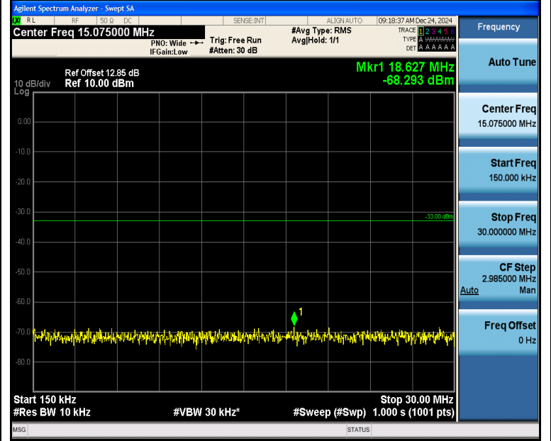
Band2_1.4MHz_QPSK_18900_1RB#0_0.15~30_0.15~30
