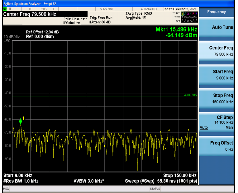
Band2_3MHz_16QAM_18615_1RB#0_0.009~0.15_0.009~0.15
