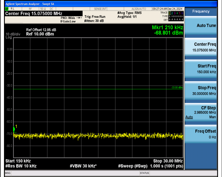
Band2_1.4MHz_QPSK_19193_1RB#5_0.15~30_0.15~30
