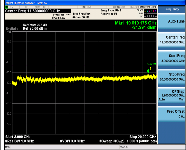
Band2_1.4MHz_QPSK_18900_6RB#0_3000~20000_3000~20000
