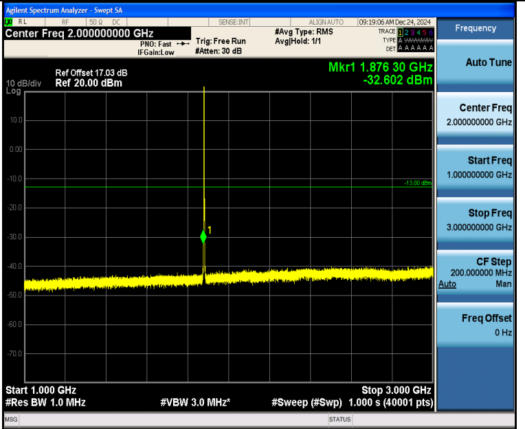
Band2_1.4MHz_QPSK_18900_1RB#0_1000~3000_1000~3000
