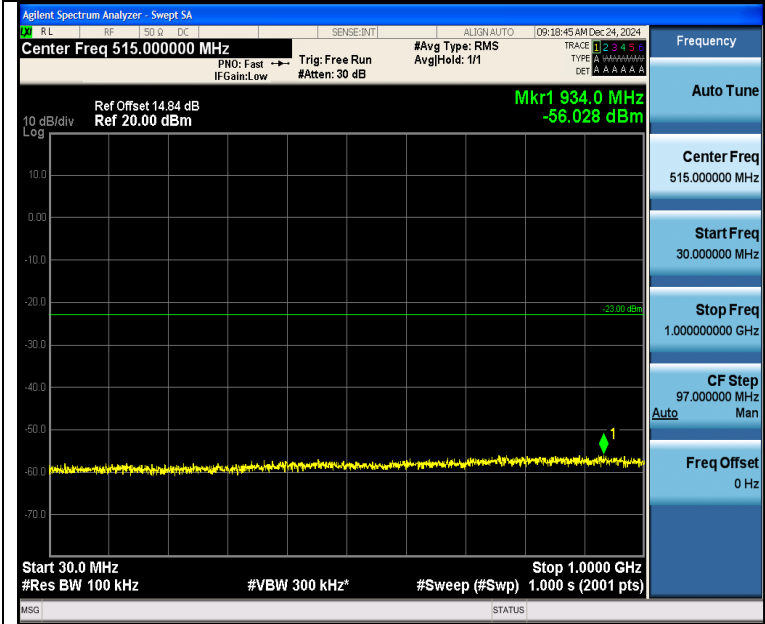
Band2_1.4MHz_QPSK_18900_1RB#0_30~1000_30~1000
