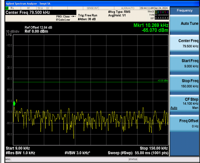
Band2_3MHz_QPSK_18900_1RB#14_0.009~0.15_0.009~0.15
