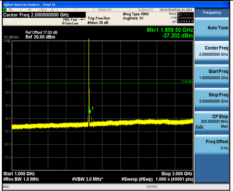
Band2_3MHz_QPSK_18615_1RB#0_1000~3000_1000~3000
