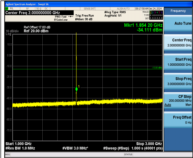
Band2_1.4MHz_16QAM_18607_6RB#0_1000~3000_1000~3000
