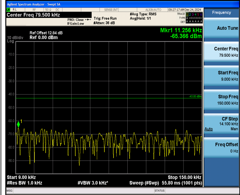
Band2_1.4MHz_QPSK_19193_1RB#5_0.009~0.15_0.009~0.15
