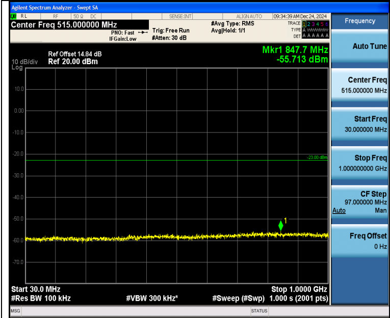
Band2_3MHz_QPSK_18615_1RB#0_30~1000_30~1000
