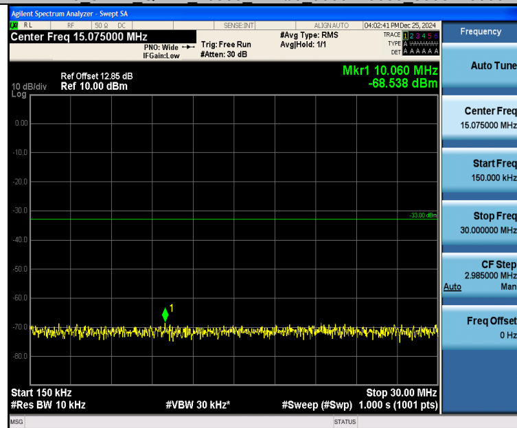
Band25_5MHz_16QAM_26365_1RB#0_0.15~30_0.15~30
