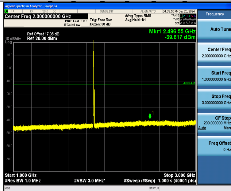
Band25_5MHz_16QAM_26365_1RB#0_1000~3000_1000~3000
