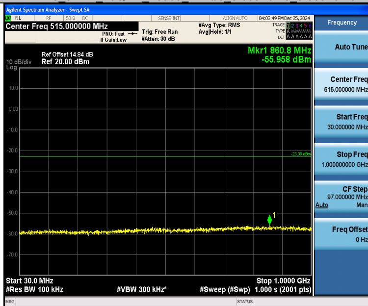
Band25_5MHz_16QAM_26365_1RB#0_30~1000_30~1000
