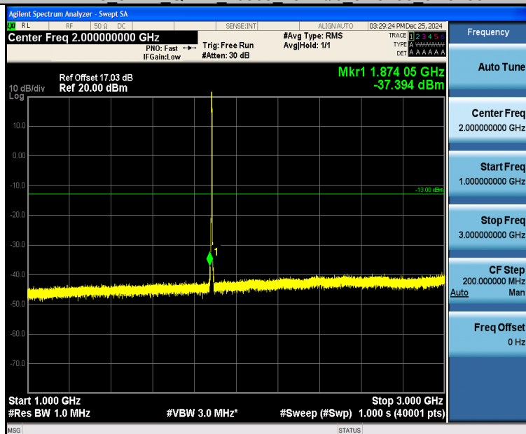
Band25_3MHz_QPSK_26365_15RB#0_1000~3000_1000~3000
