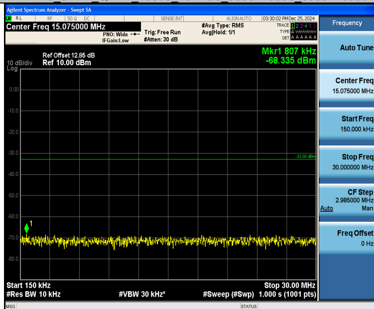
Band25_3MHz_16QAM_26365_15RB#0_0.15~30_0.15~30
