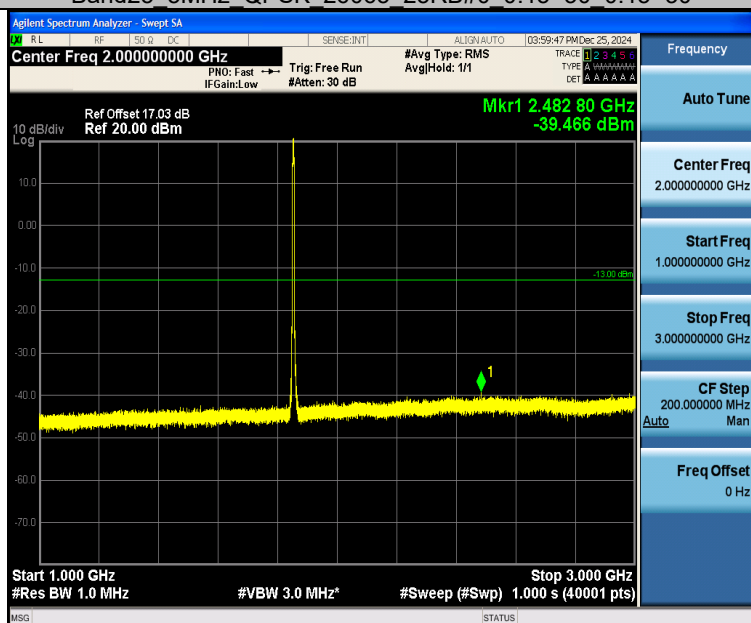
Band25_5MHz_QPSK_26065_25RB#0_1000~3000_1000~3000
