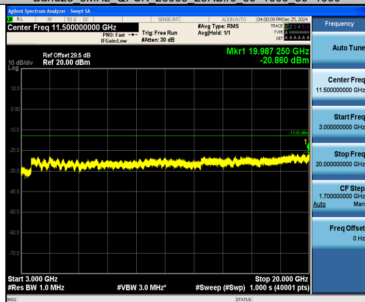
Band25_5MHz_QPSK_26065_25RB#0_3000~20000_3000~20000
