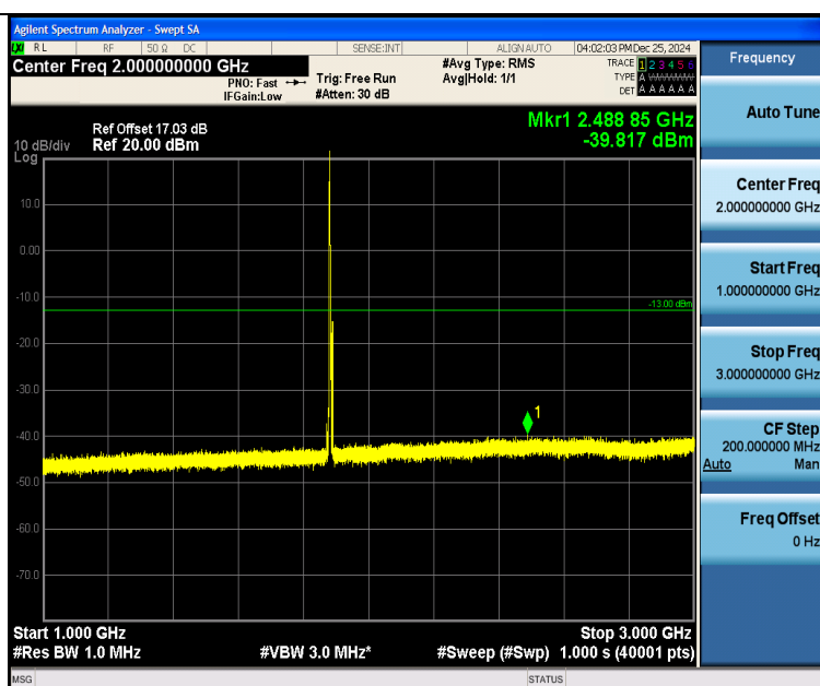
Band25_5MHz_QPSK_26365_1RB#0_1000~3000_1000~3000
