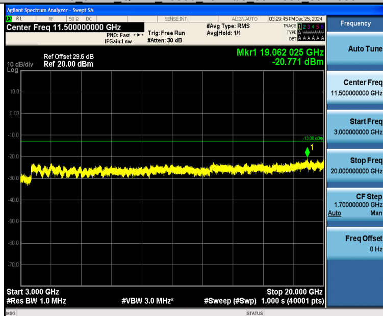
Band25_3MHz_QPSK_26365_15RB#0_3000~20000_3000~20000
