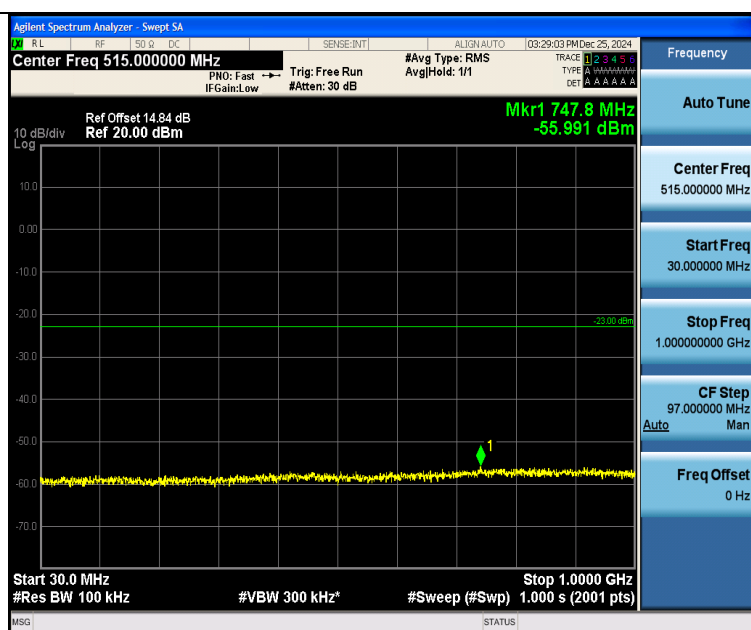
Band25_3MHz_QPSK_26365_15RB#0_30~1000_30~1000
