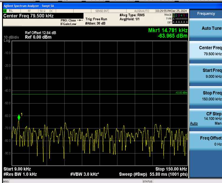
Band25_3MHz_16QAM_26365_15RB#0_0.009~0.15_0.009~0.15
