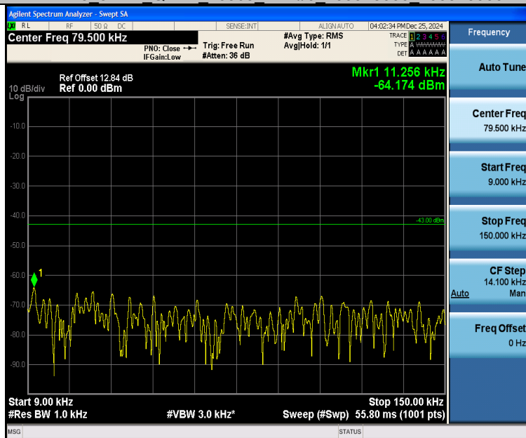
Band25_5MHz_16QAM_26365_1RB#0_0.009~0.15_0.009~0.15
