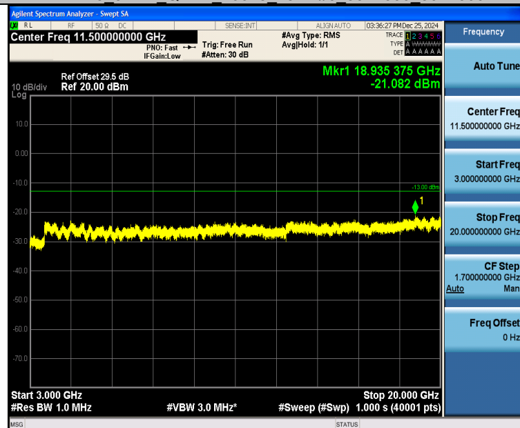
Band25_3MHz_QPSK_26675_15RB#0_3000~20000_3000~20000
