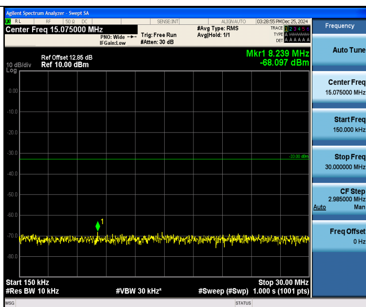
Band25_3MHz_QPSK_26365_15RB#0_0.15~30_0.15~30
