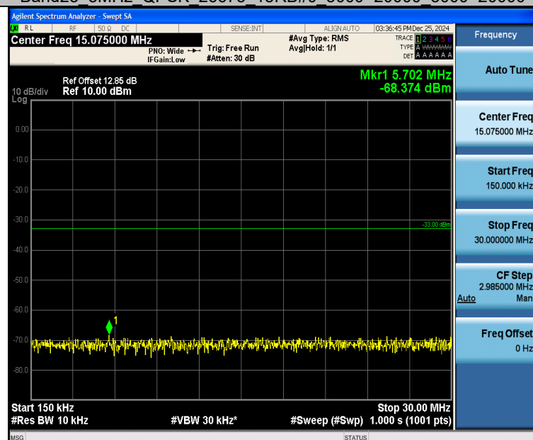
Band25_3MHz_16QAM_26675_15RB#0_0.15~30_0.15~30
