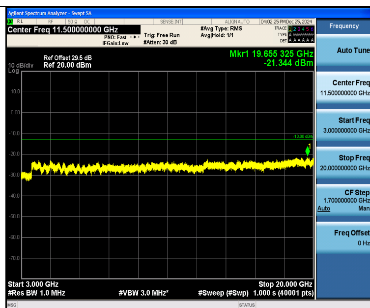
Band25_5MHz_QPSK_26365_1RB#0_3000~20000_3000~20000
