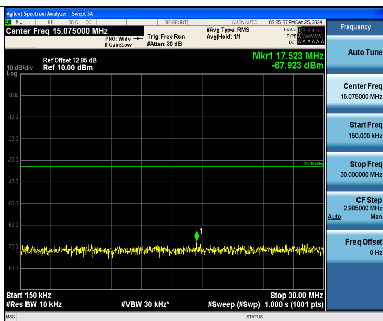
Band25_3MHz_QPSK_26675_15RB#0_0.15~30_0.15~30
