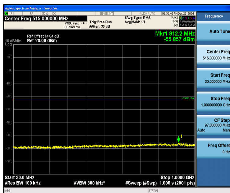
Band25_3MHz_QPSK_26675_15RB#0_30~1000_30~1000
