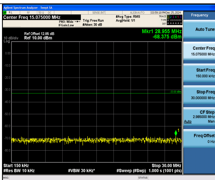
Band25_5MHz_QPSK_26065_25RB#0_0.15~30_0.15~30
