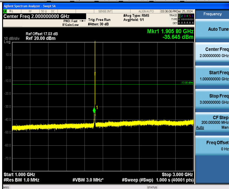
Band25_3MHz_QPSK_26675_15RB#0_1000~3000_1000~3000
