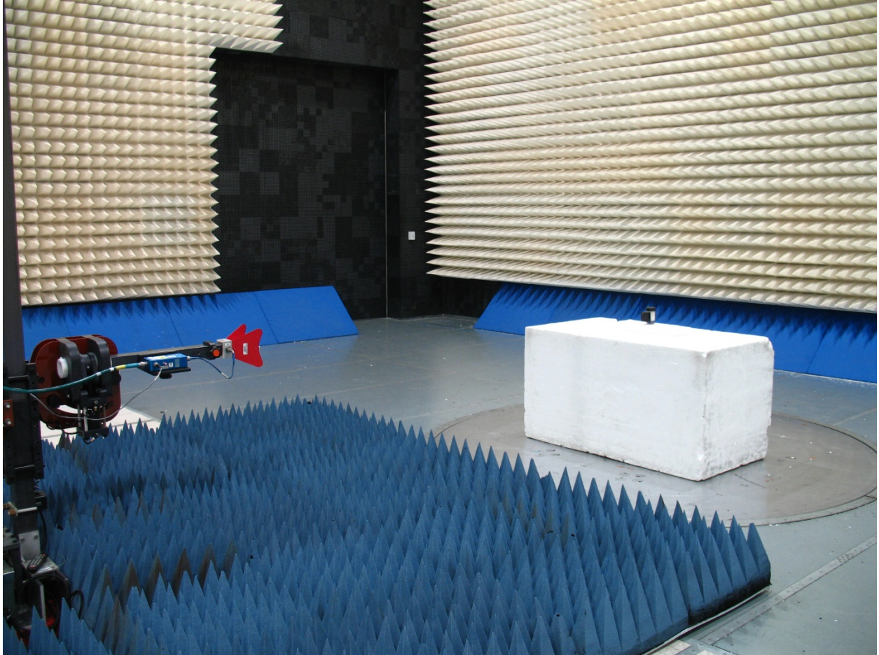
Radiated Emissions, 1GHz-18GHz (Receive/idle mode)
