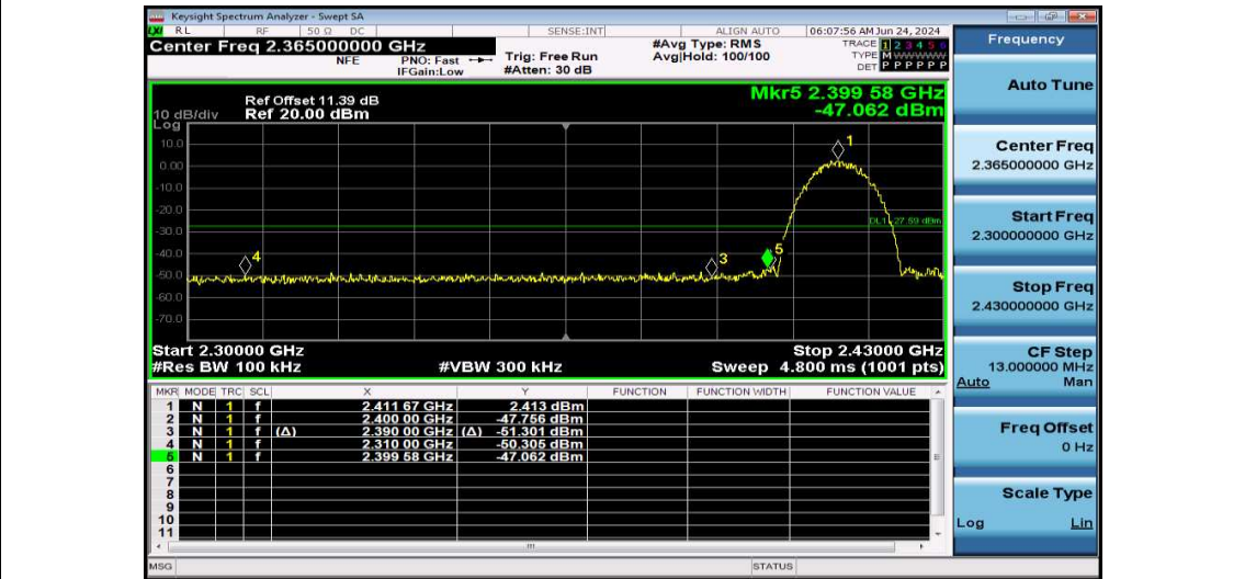
11B-Ant2-2412-PASS
