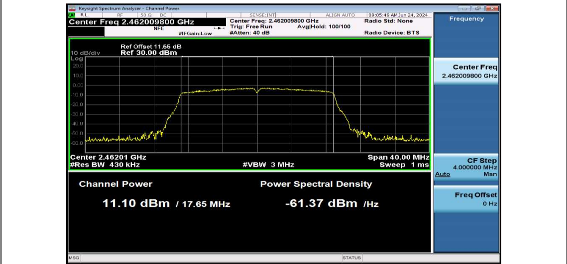
11N20MIMO-Ant2-2462-PASS
