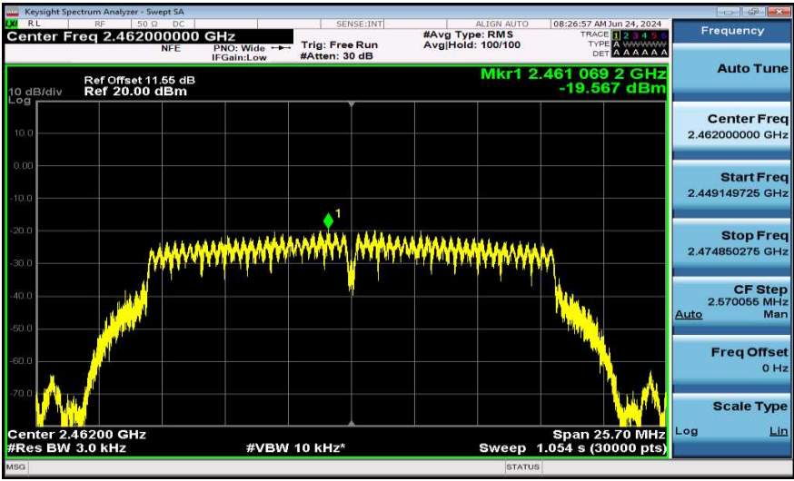
11G-Ant2-2462-PASS
