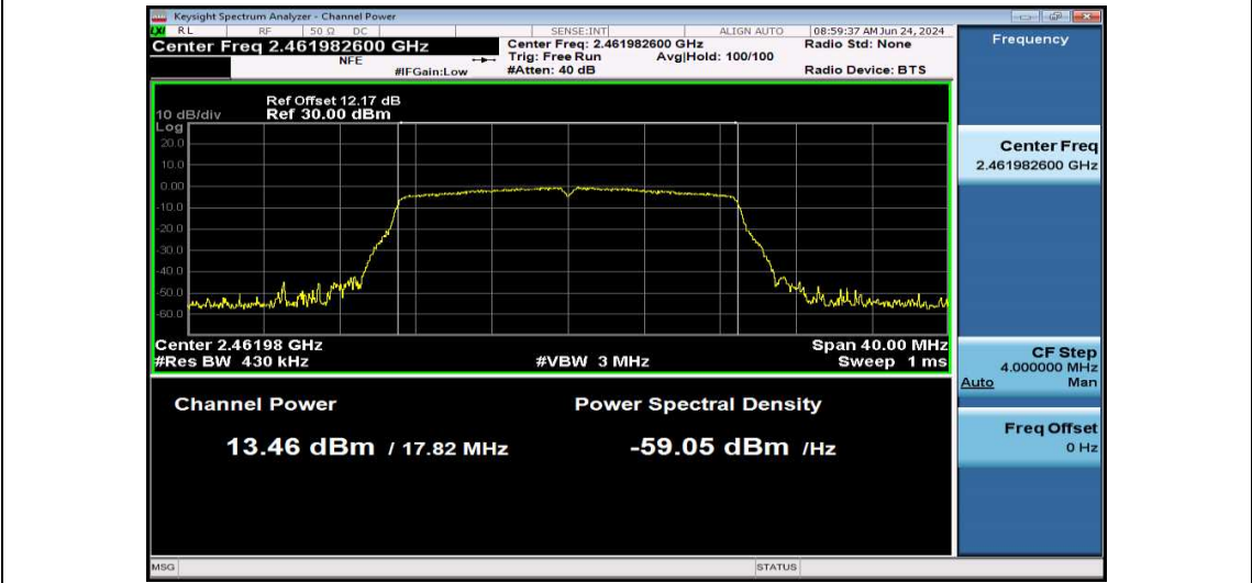
11N20MIMO-Ant1-2462-PASS
