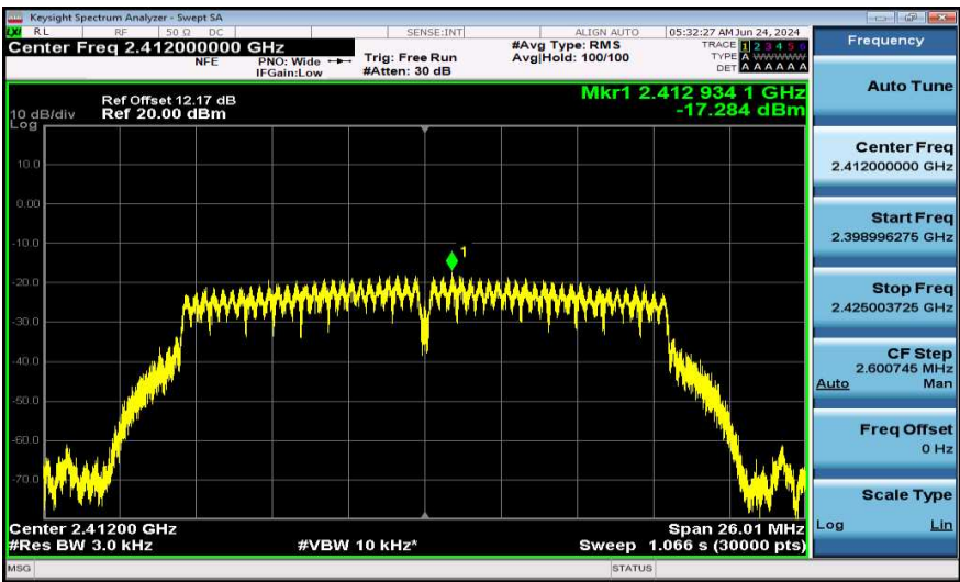
11G-Ant1-2412-PASS
