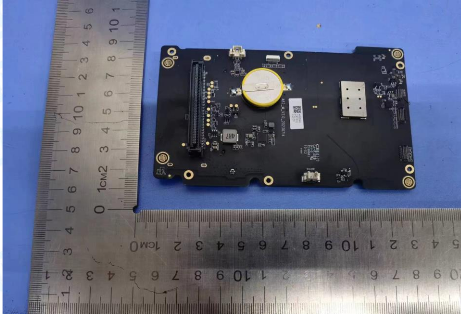
Photo 26 Appearance of PCB
