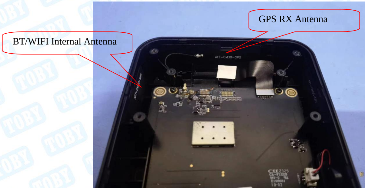
Photo 20 Internal of EUT
