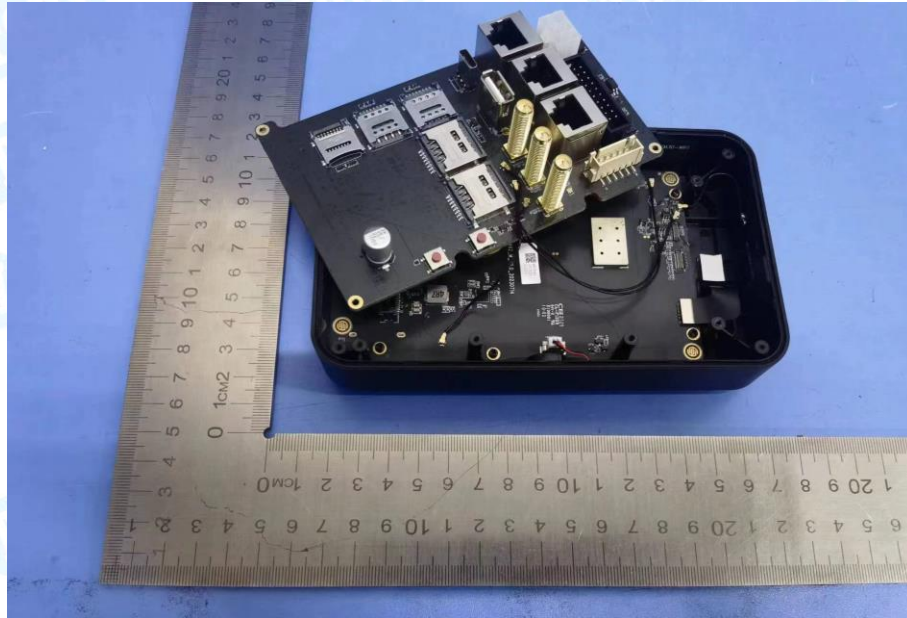
Photo 18 Internal of EUT
