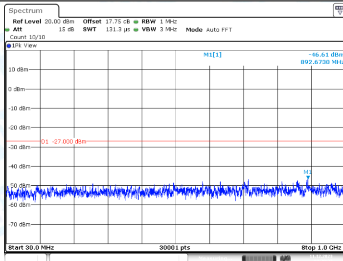
11N40SISO_Ant1_5755_30~1000
