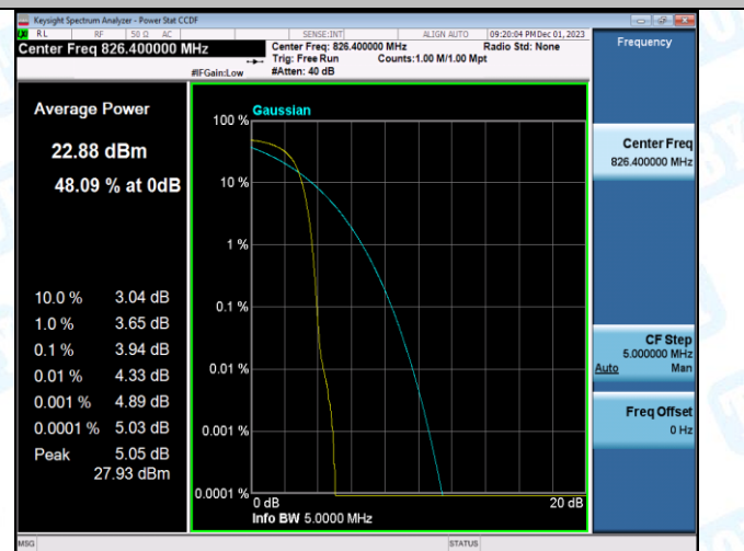
Band5-4233-4-PASS
