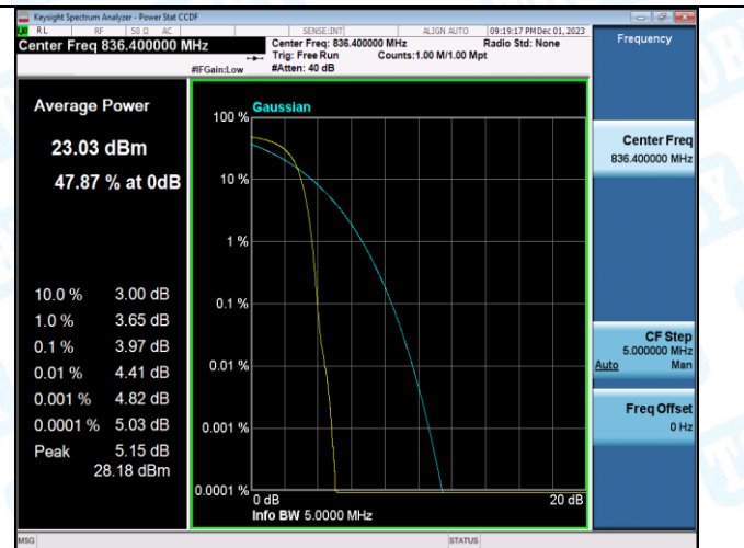
Band5-4132-4-PASS
