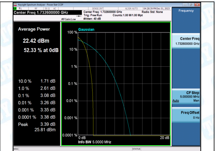
Band4-1312-2-PASS
