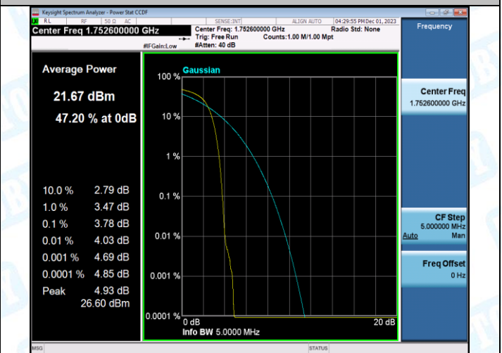
Band4-1413-3-PASS
