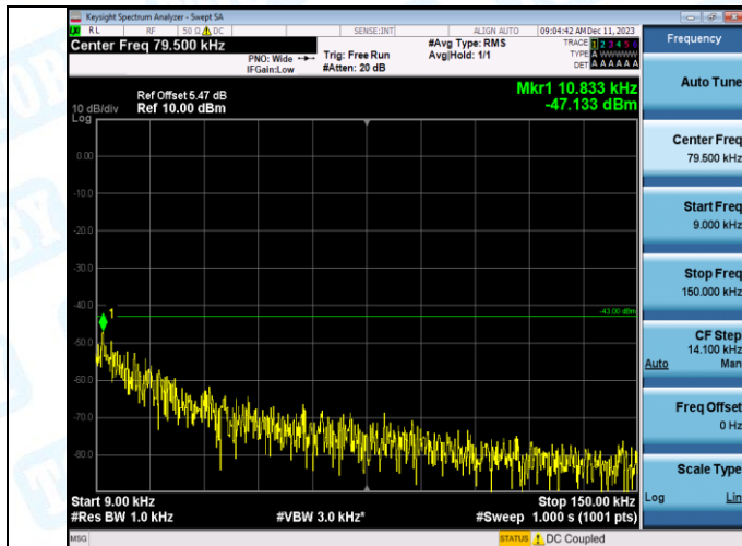
Band2-9400-5-0.009~0.15MHz-PASS
