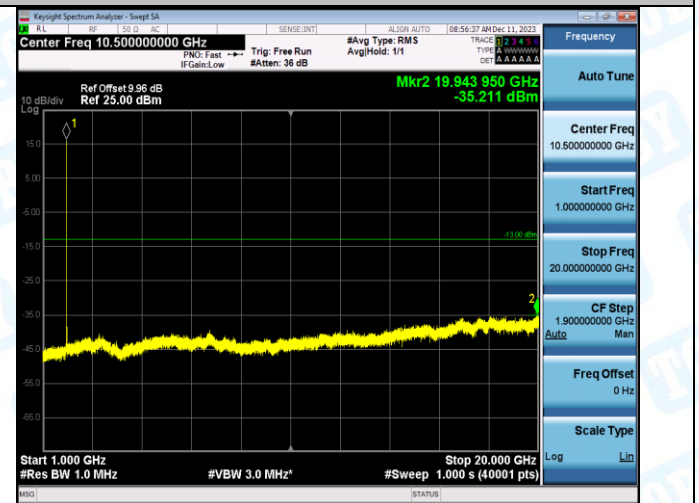
Band2-9262-5-1000~20000MHz-PASS
