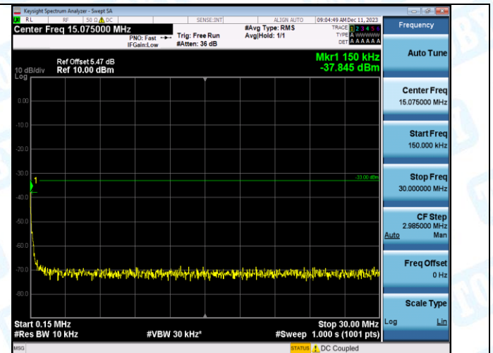
Band2-9400-5-0.15~30MHz-PASS
