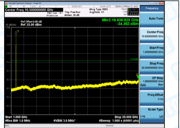
Band4-1513-3-0.15~30MHz-PASS
