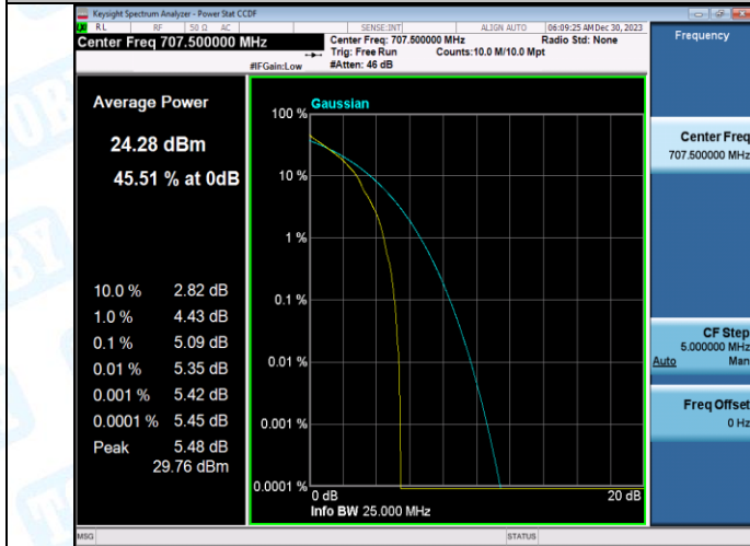
Band12-5MHz-QPSK-23095-25RB#0-PASS
