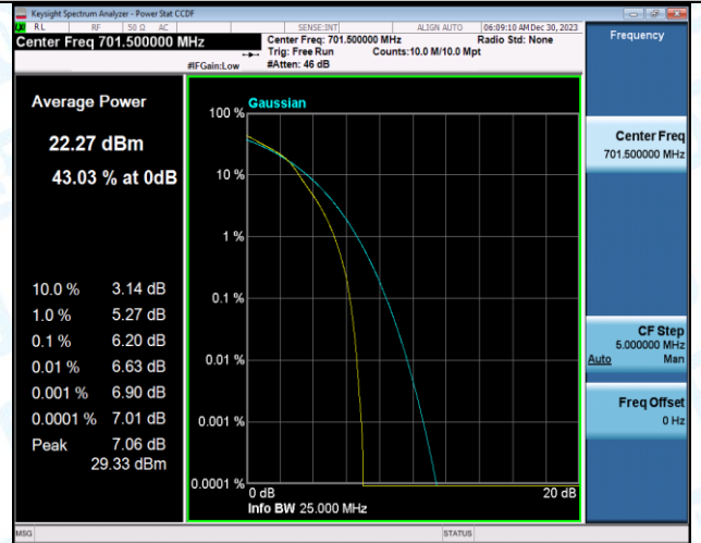
Band12-5MHz-16QAM-23095-1RB#0-PASS
