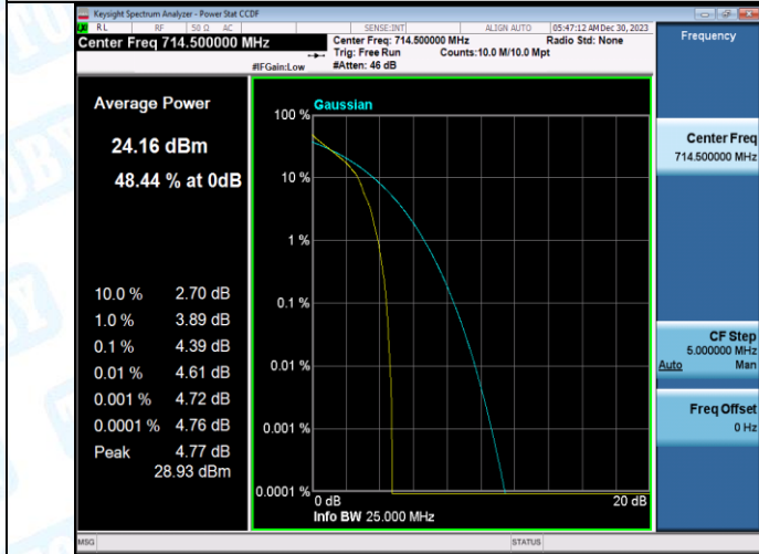
Band12-3MHz-QPSK-23165-15RB#0-PASS
