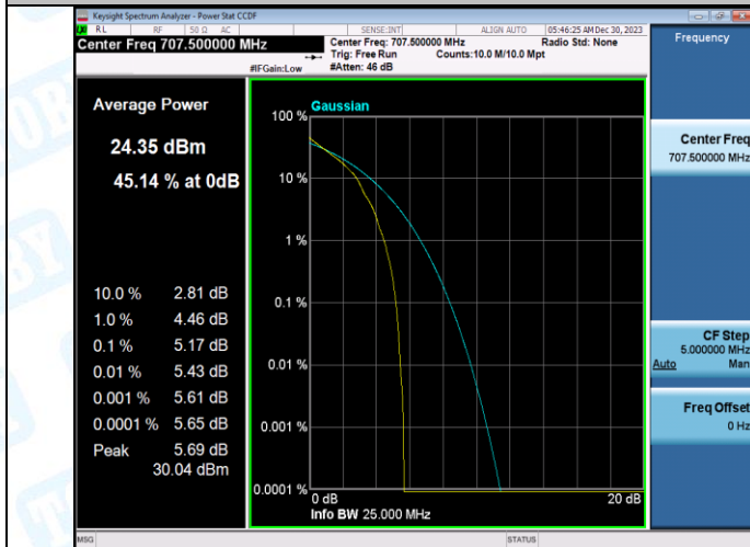
Band12-3MHz-QPSK-23095-15RB#0-PASS
