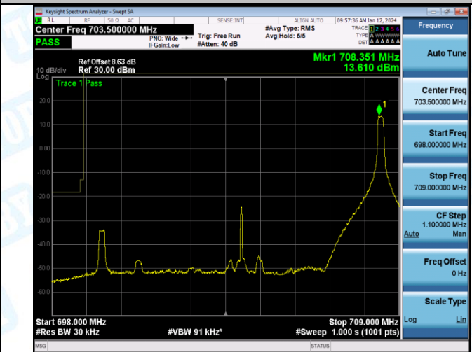
Band12_10MHz_16QAM_23060_50RB#0
