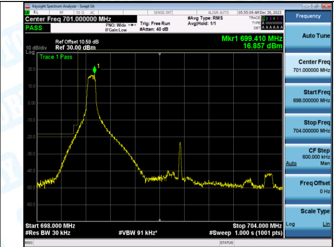
Band12_5MHz_16QAM_23035_1RB#24
