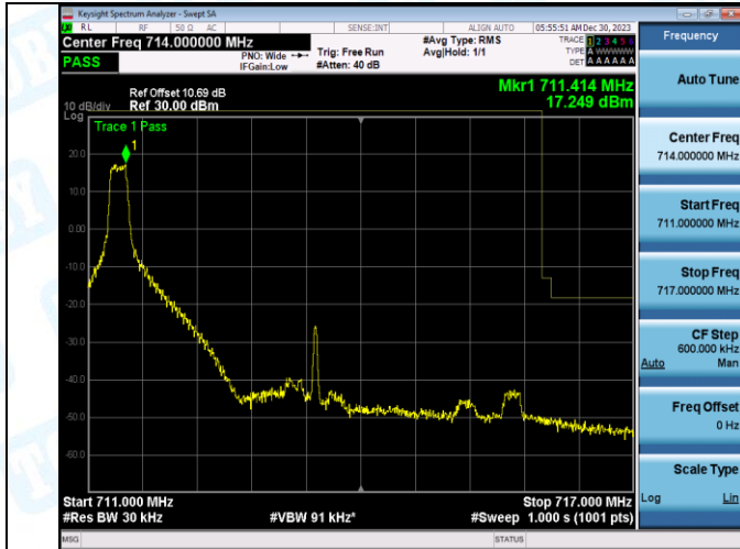
Band12_5MHz_QPSK_23155_1RB#24
