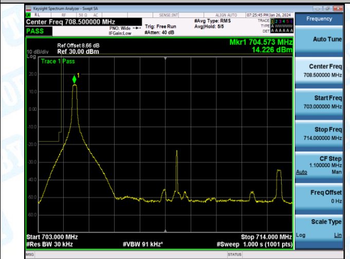
Band17_10MHz_16QAM_23780_50RB#0
