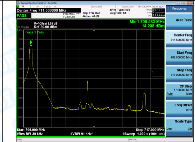
Band17_10MHz_16QAM_23800_50RB#0
