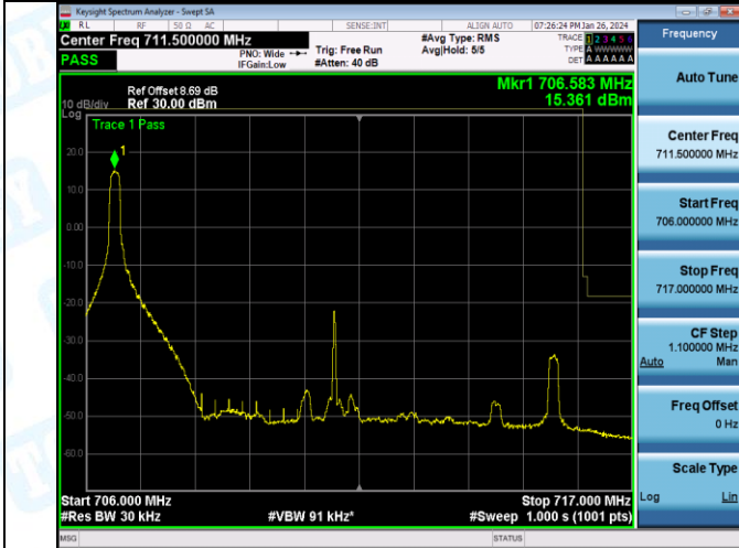
Band17_10MHz_QPSK_23800_50RB#0
