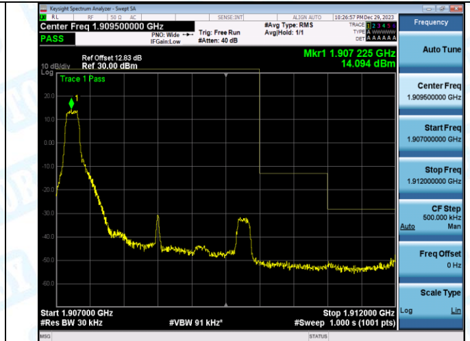
Band2_3MHz_16QAM_19185_1RB#14
