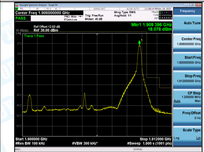
Band2_10MHz_16QAM_19150_50RB#0
