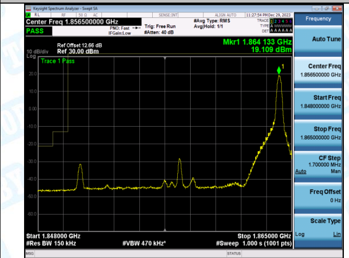
Band2_15MHz_16QAM_18675_75RB#0
