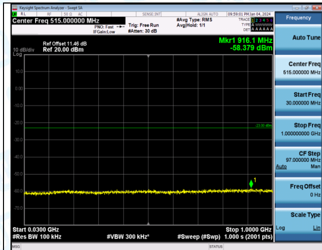
Band2_3MHz_16QAM_18615_1RB#0_3000-20000_3000-20000
