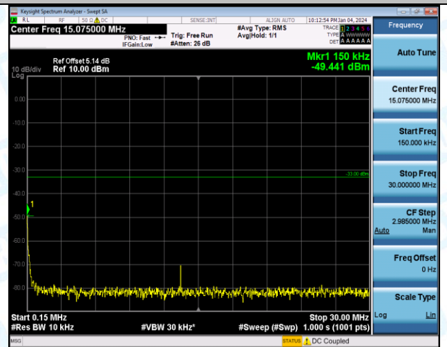
Band2_10MHz_16QAM_18900_1RB#0_1000~3000_1000~3000
