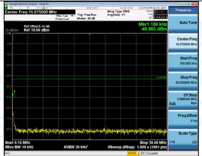
Band2_10MHz_16QAM_19150_1RB#0_1000~3000_1000~3000
