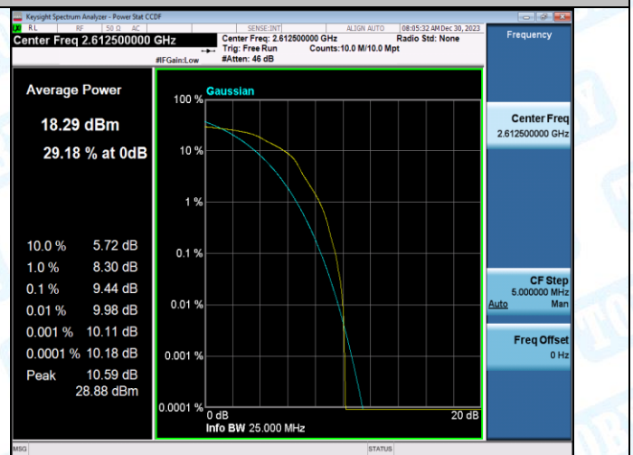
Band38-15MHz-16QAM-38175-75RB#0-PASS
