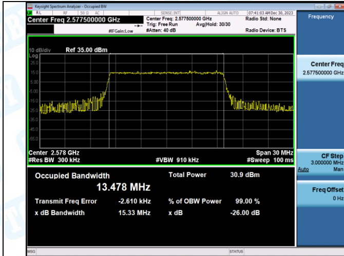
Band38-15MHz-QPSK-38000-75RB#0-PASS
