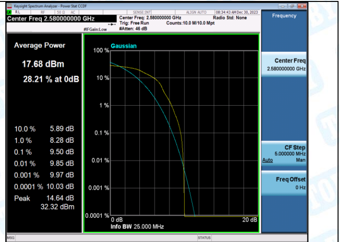
Band38-20MHz-16QAM-37850-100RB#0-PASS
