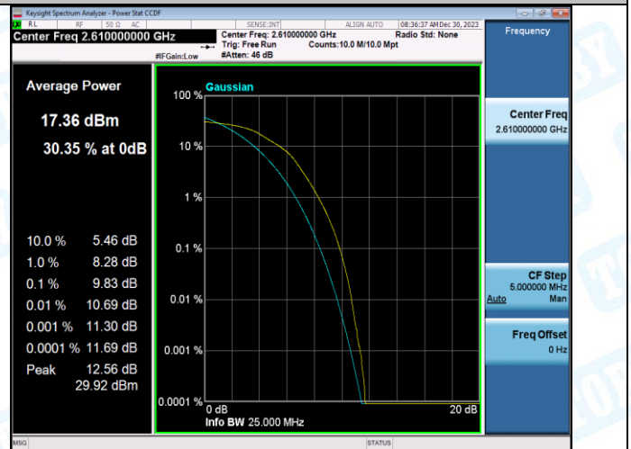
Band38-20MHz-16QAM-38150-100RB#0-PASS
