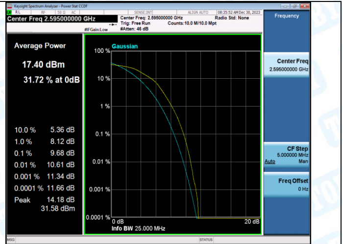
Band38-20MHz-16QAM-38150-1RB#0-PASS
