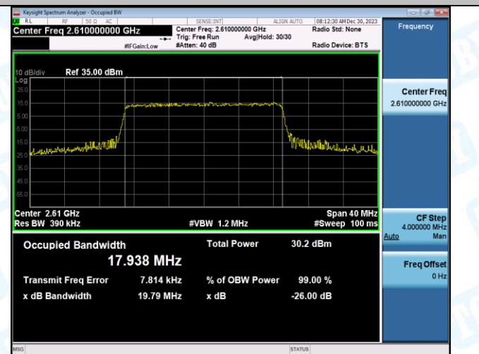
Band38-20MHz-16QAM-38150-100RB#0-PASS
