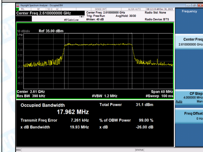
Band38-20MHz-QPSK-38150-100RB#0-PASS
