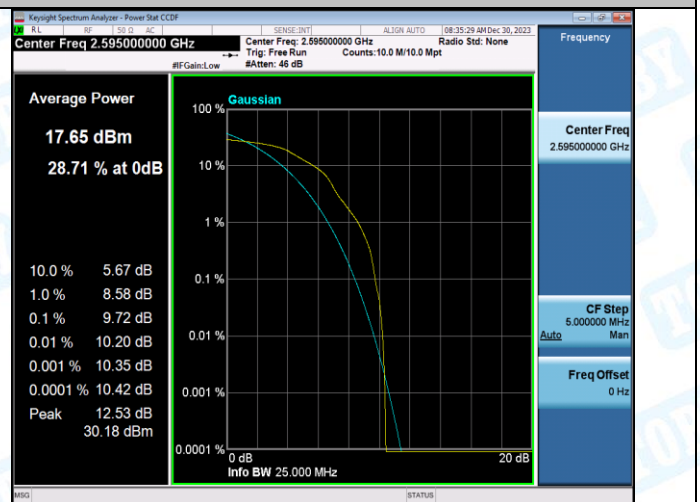
Band38-20MHz-16QAM-38000-100RB#0-PASS
