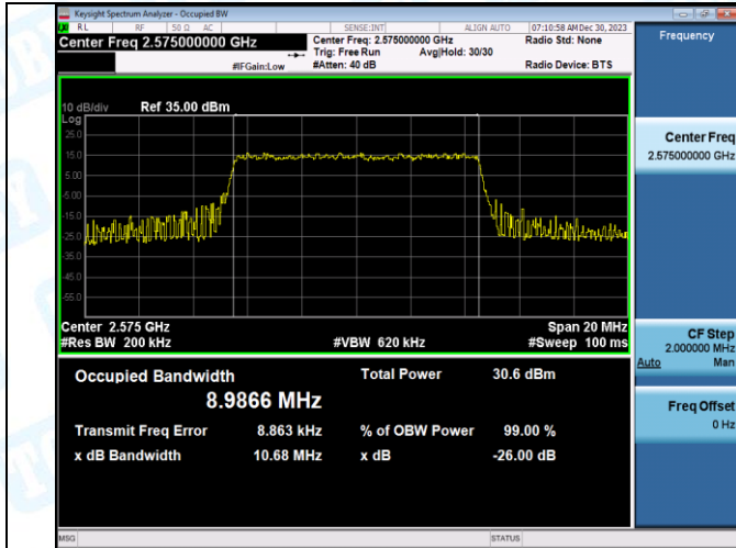
Band38-10MHz-QPSK-38000-50RB#0-PASS
