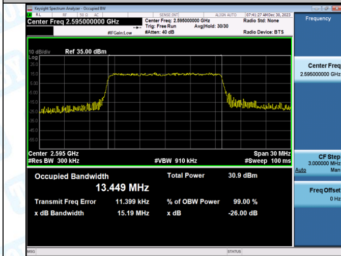
Band38-15MHz-QPSK-38175-75RB#0-PASS
