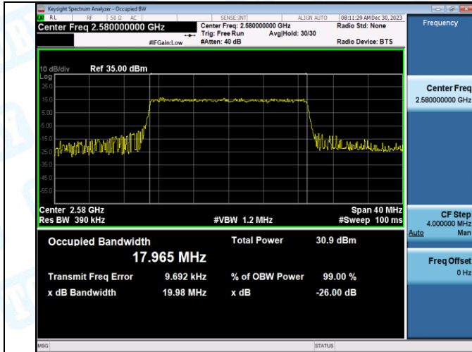
Band38-20MHz-QPSK-38000-100RB#0-PASS
