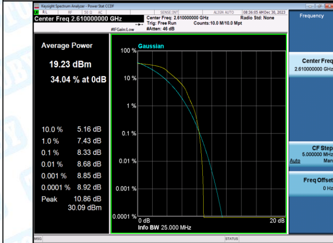
Band38-20MHz-QPSK-38150-100RB#0-PASS
