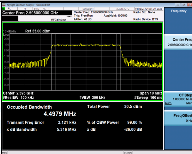
Band38-5MHz-QPSK-38225-25RB#0-PASS
