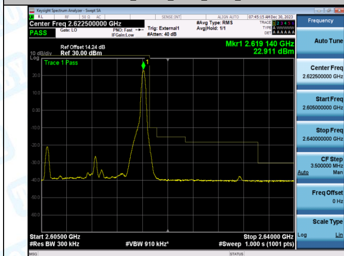
Band38_15MHz_QPSK_38175_75RB#0
