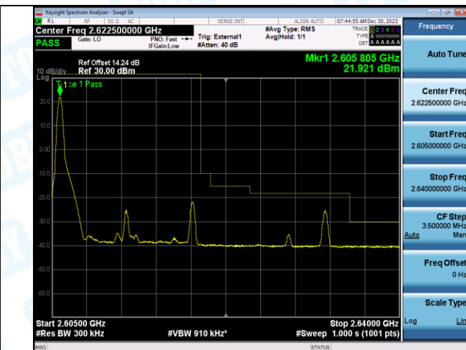
Band38_15MHz_16QAM_38175_1RB#74
