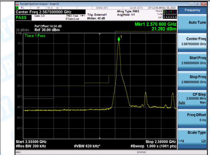
Band38_10MHz_16QAM_37800_1RB#49
