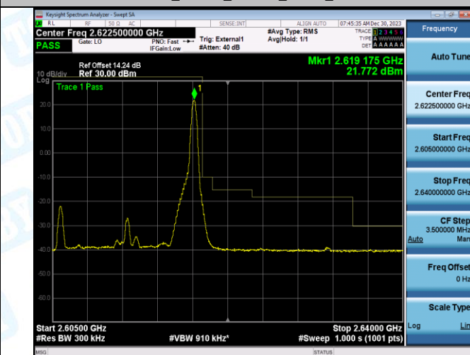
Band38_15MHz_16QAM_38175_75RB#0
