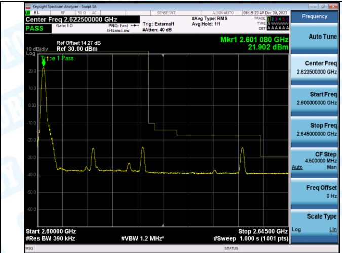
Band38_20MHz_16QAM_38150_1RB#99
