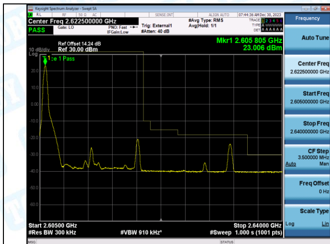
Band38_15MHz_QPSK_38175_1RB#74
