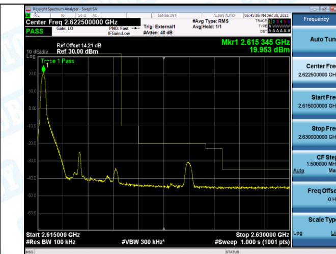
Band38_5MHz_16QAM_38225_1RB#24
