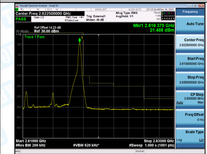
Band38_10MHz_16QAM_38200_50RB#0
