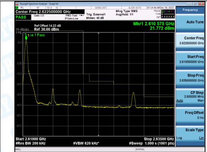
Band38_10MHz_16QAM_38200_1RB#49
