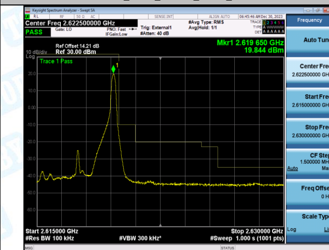
Band38_5MHz_16QAM_38225_25RB#0
