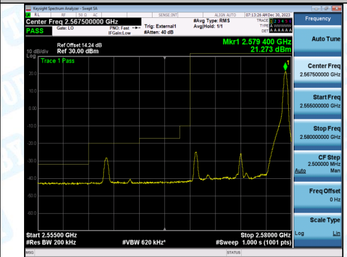
Band38_10MHz_16QAM_37800_50RB#0
