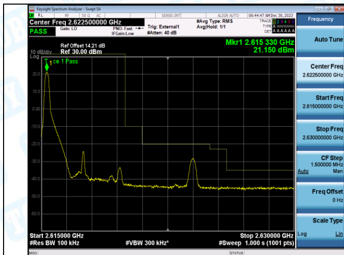
Band38_5MHz_QPSK_38225_1RB#24
