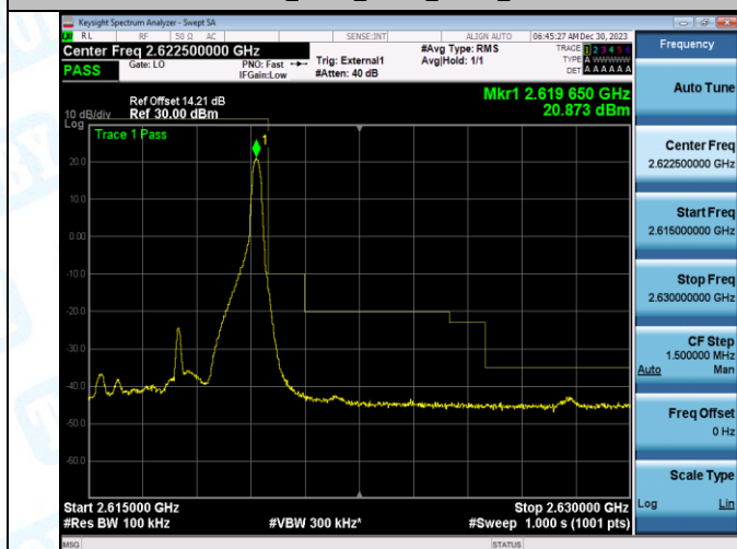
Band38_5MHz_QPSK_38225_25RB#0
