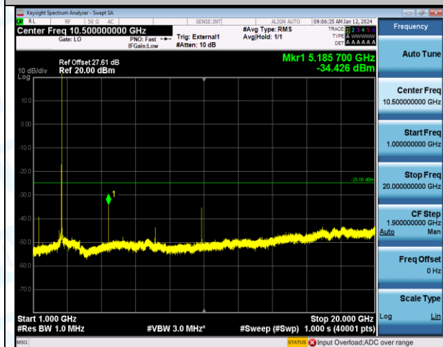
Band38_5MHz_16QAM_38000_1RB#0_0.009~0.15_0.009~0.15
