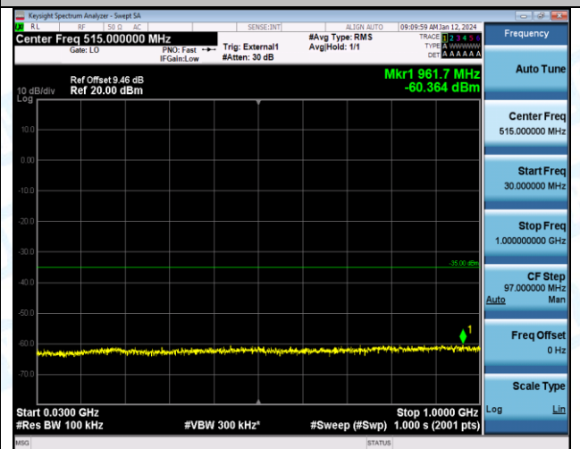
Band38_15MHz_QPSK_38175_1RB#0_30~1000_30~1000
