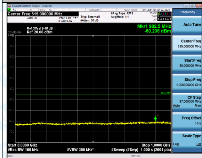
Band38_10MHz_16QAM_37800_1RB#0_20000~27000_20000~27000
