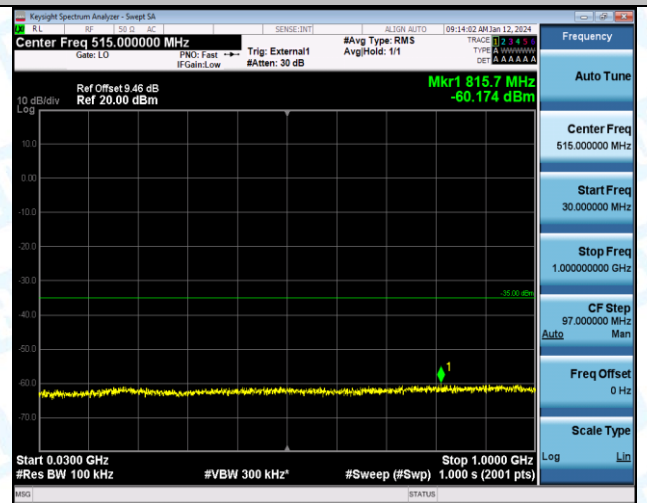
Band38_10MHz_QPSK_37800_1RB#0_20000~27000_20000~27000
