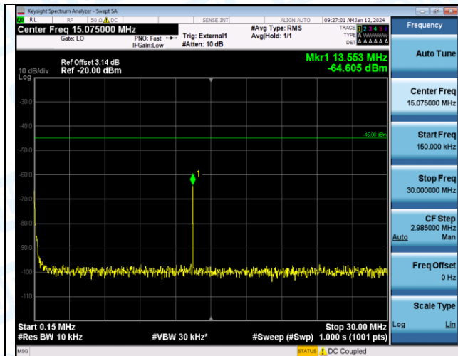
Band38_15MHz_16QAM_37825_1RB#0_1000~20000_1000~20000
