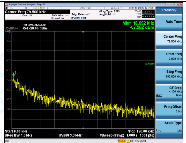
Band38_20MHz_QPSK_37850_1RB#0_0.009~0.15_0.009~0.15
