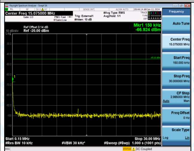
Band38_20MHz_QPSK_38150_1RB#0_1000~20000_1000~20000
