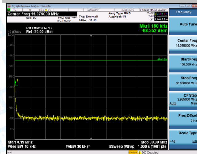
Band38_20MHz_QPSK_37850_1RB#0_1000~20000_1000~20000
