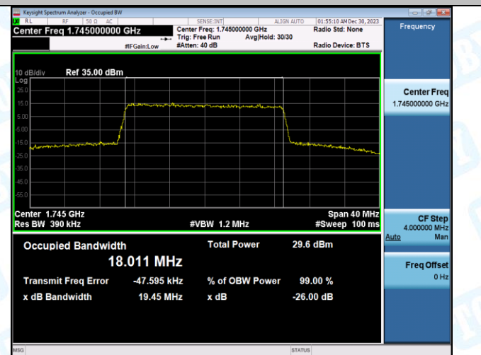
Band4-20MHz-16QAM-20300-100RB#0-PASS
