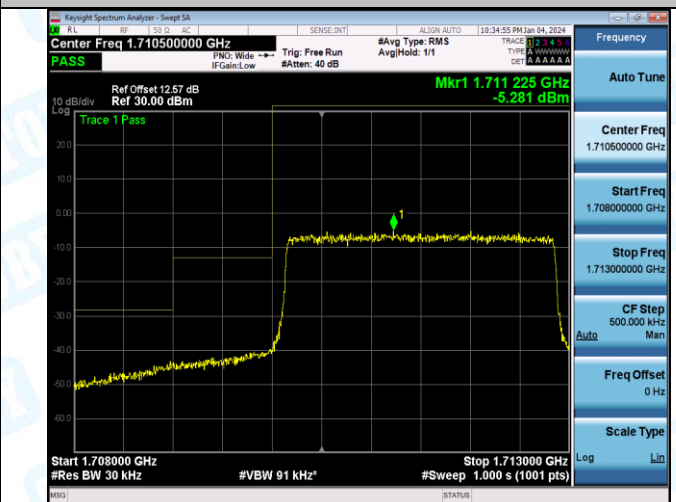
Band4_5MHz_16QAM_19975_1RB#0
