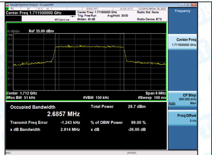
Band4-3MHz-16QAM-20175-15RB#0-PASS
