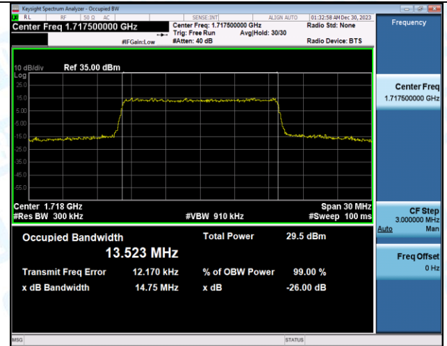
Band4-15MHz-16QAM-20175-75RB#0-PASS
