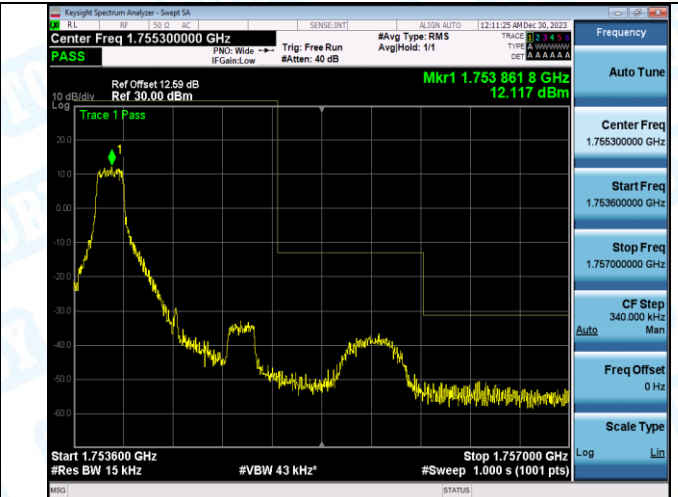
Band4_1.4MHz_16QAM_20393_1RB#5
