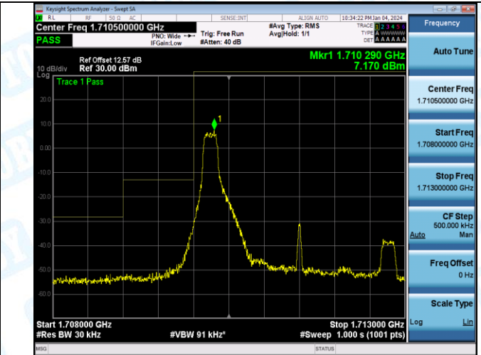
Band4_3MHz_16QAM_19965_1RB#14
