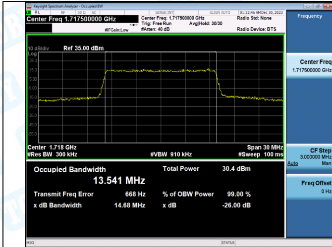
Band4-15MHz-QPSK-20175-75RB#0-PASS
