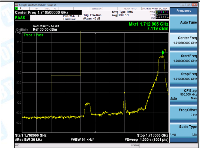
Band4_3MHz_16QAM_19965_15RB#0
