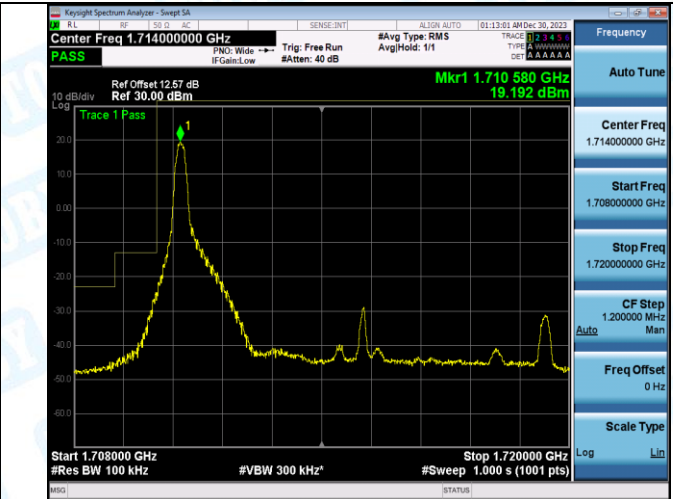
Band4_10MHz_16QAM_20000_1RB#49
