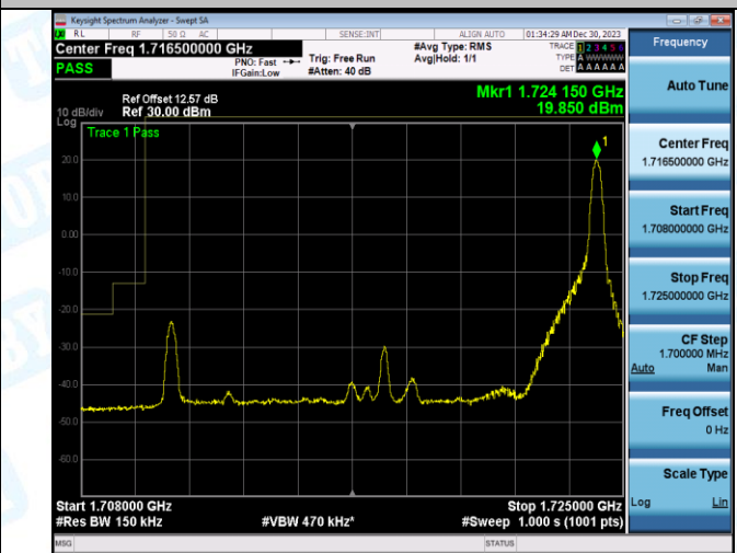
Band4_15MHz_16QAM_2025_75RB#0
