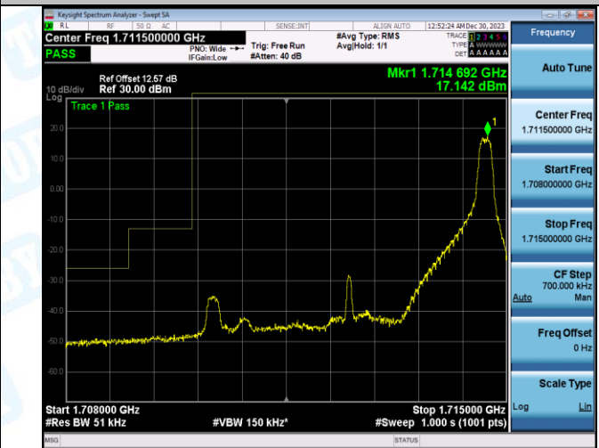
Band4_5MHz_16QAM_19975_25RB#0
