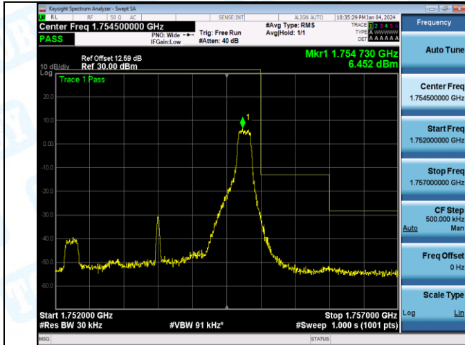
Band4_3MHz_16QAM_20385_15RB#0
