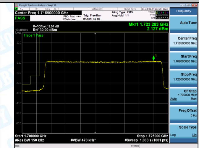
Band4_15MHz_16QAM_2025_1RB#0
