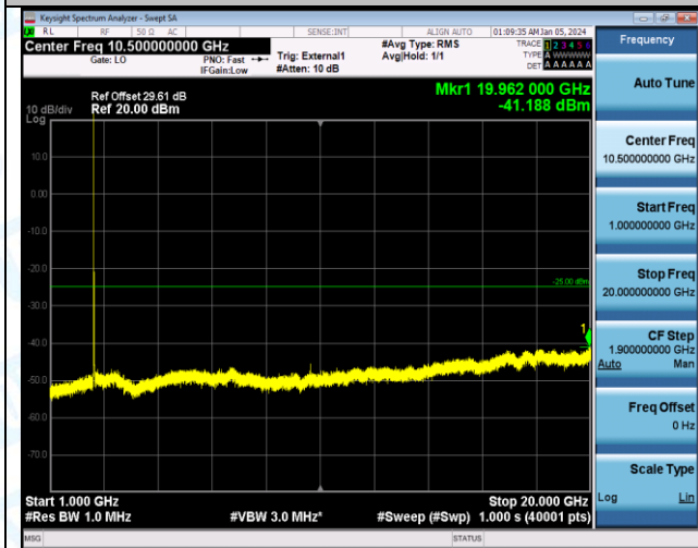
Band41_15MHz_QPSK_40590_1RB#0_0.15~30_0.15~30
