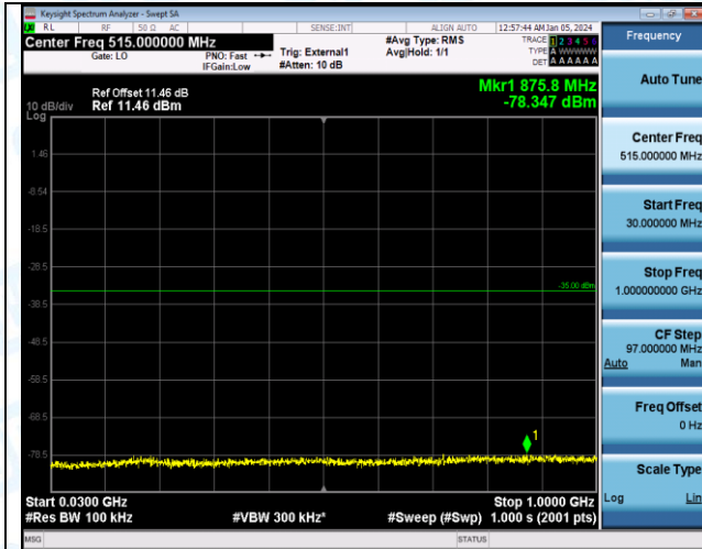
Band41_10MHz_16QAM_4090_1RB#0_1000~20000_1000~20000
