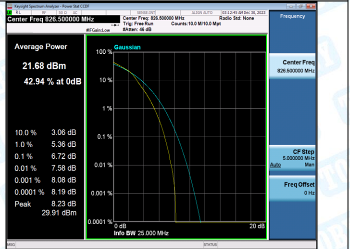
Band5-5MHz-16QAM-20525-1RB#0-PASS
