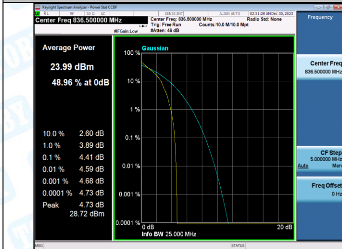
Band5-3MHz-QPSK-20525-15RB#0-PASS
