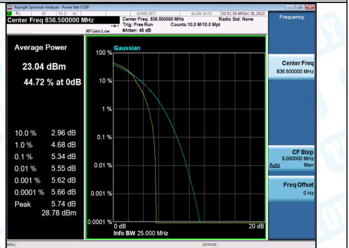
Band5-3MHz-16QAM-20525-15RB#0-PASS
