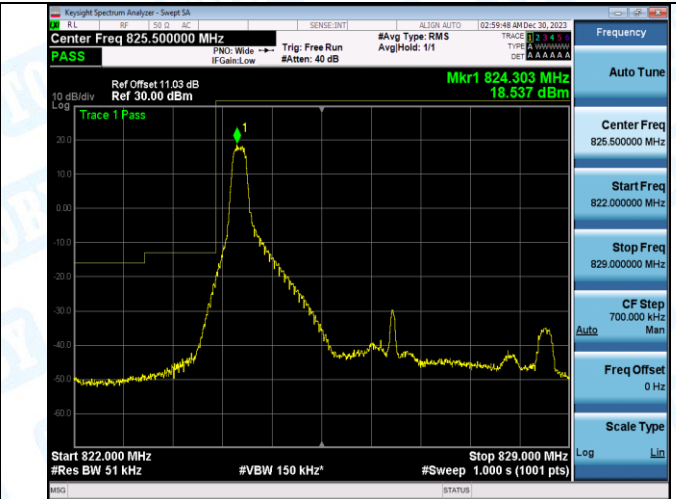
Band5_5MHz_16QAM_20425_1RB#24
