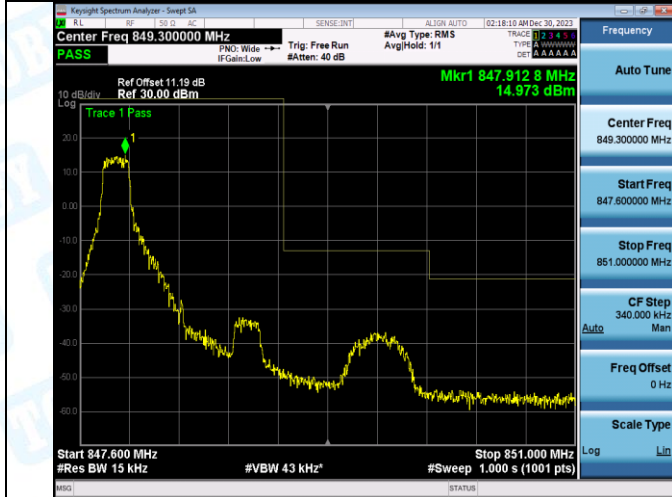
Band5_1.4MHz_QPSK_20643_1RB#5
