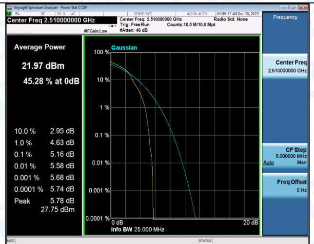
Band7-20MHz-16QAM-20850-100RB#0-PASS
