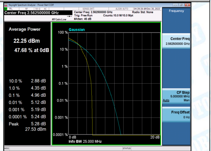
Band7-15MHz-16QAM-21375-75RB#0-PASS
