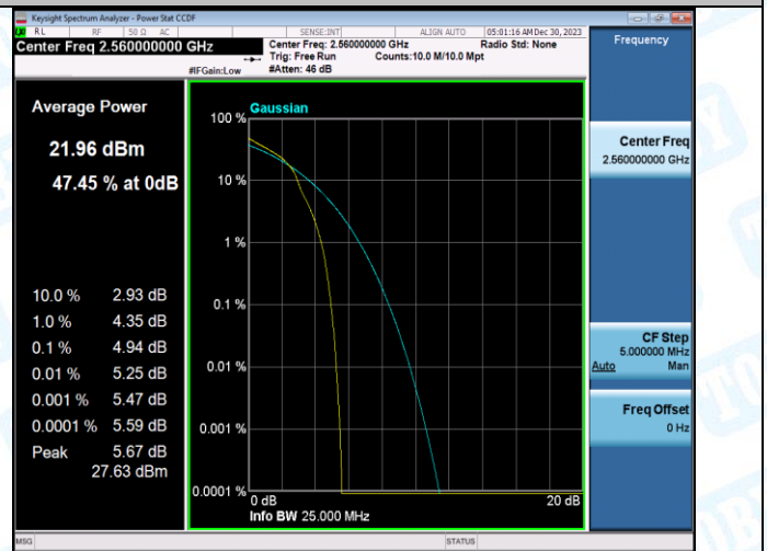
Band7-20MHz-16QAM-21350-100RB#0-PASS
