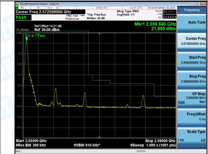
Band7_15MHz_16QAM_21375_1RB#74
