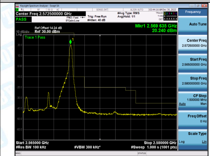
Band7_5MHz_16QAM_21425_25RB#0
