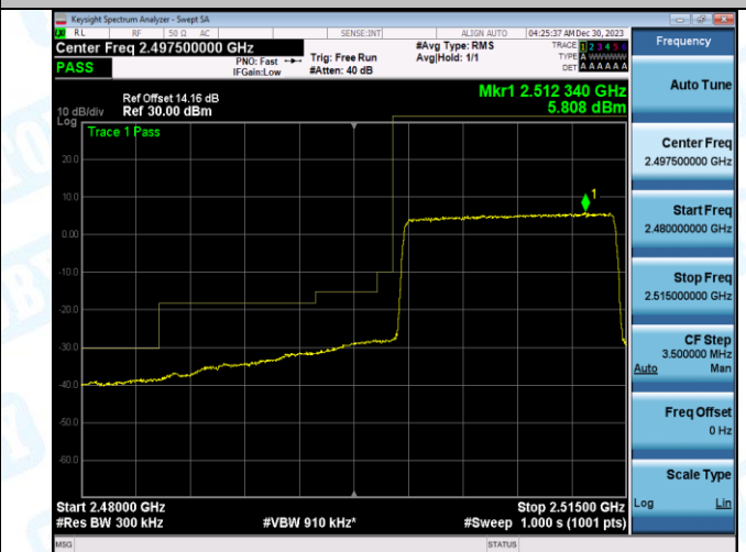
Band7_15MHz_16QAM_21375_1RB#0
