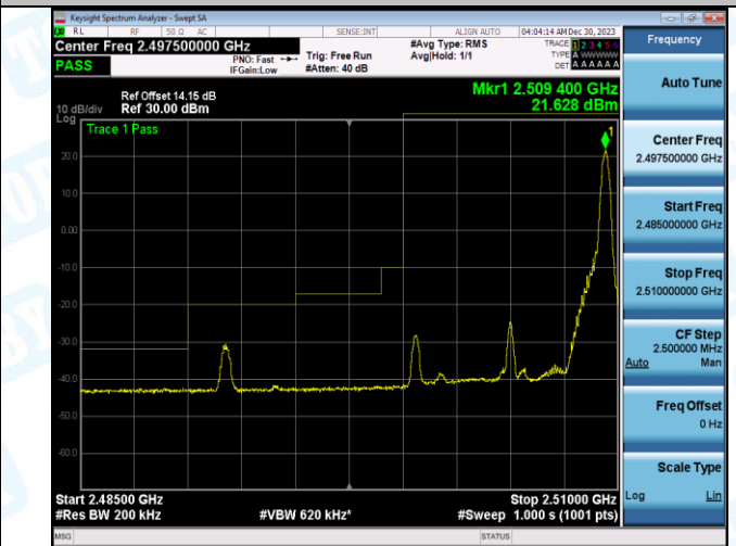
Band7_10MHz_16QAM_20800_50RB#0
