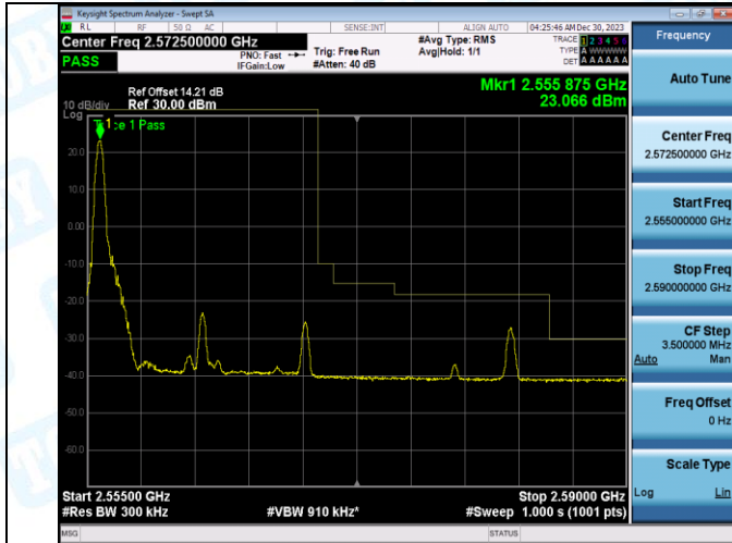
Band7_15MHz_QPSK_21375_1RB#74
