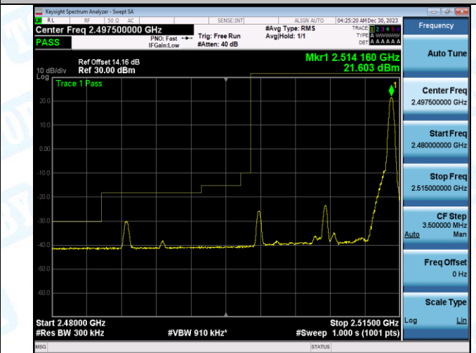
Band7_15MHz_16QAM_20825_75RB#0
