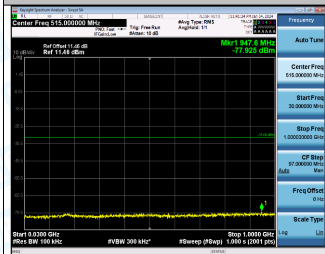
Band7_10MHz_QPSK_21400_1RB#0_20000~27000_20000~27000
