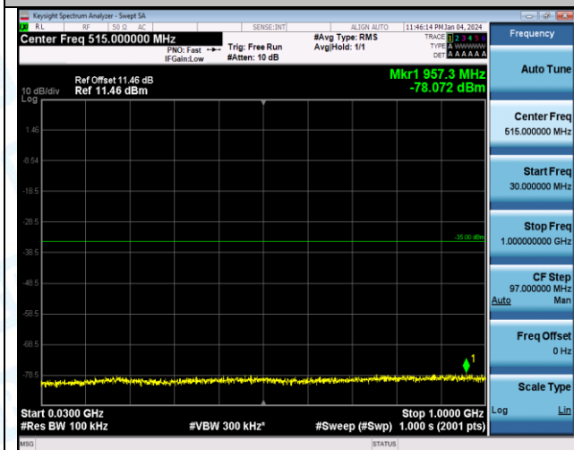
Band7_15MHz_16QAM_21100_1RB#0_20000~27000_20000~27000
